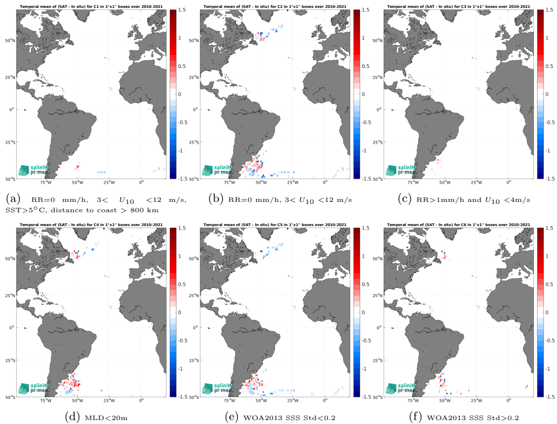
Figure 14: Temporal mean gridded over spatial boxes of size 1^\circ \times 1^\circ of \Delta\text{SSS} (CCI SSS L4 Merged-OI v4.41 - 7-day running (ESA) - Marine mammals) for 6 different subdatasets corresponding to:RR=0 mm/h, 3 < U_{10} < 12 m/s, SST>5°C, distance to coast > 800 km (a), RR=0 mm/h, 3 < U_{10} < 12 m/s (b), RR>1mm/h and U_{10} < 4 m/s (c),MLD<20m (d),WOA2013 SSS Std<0.2 (e),WOA2013 SSS Std>0.2 (f).
