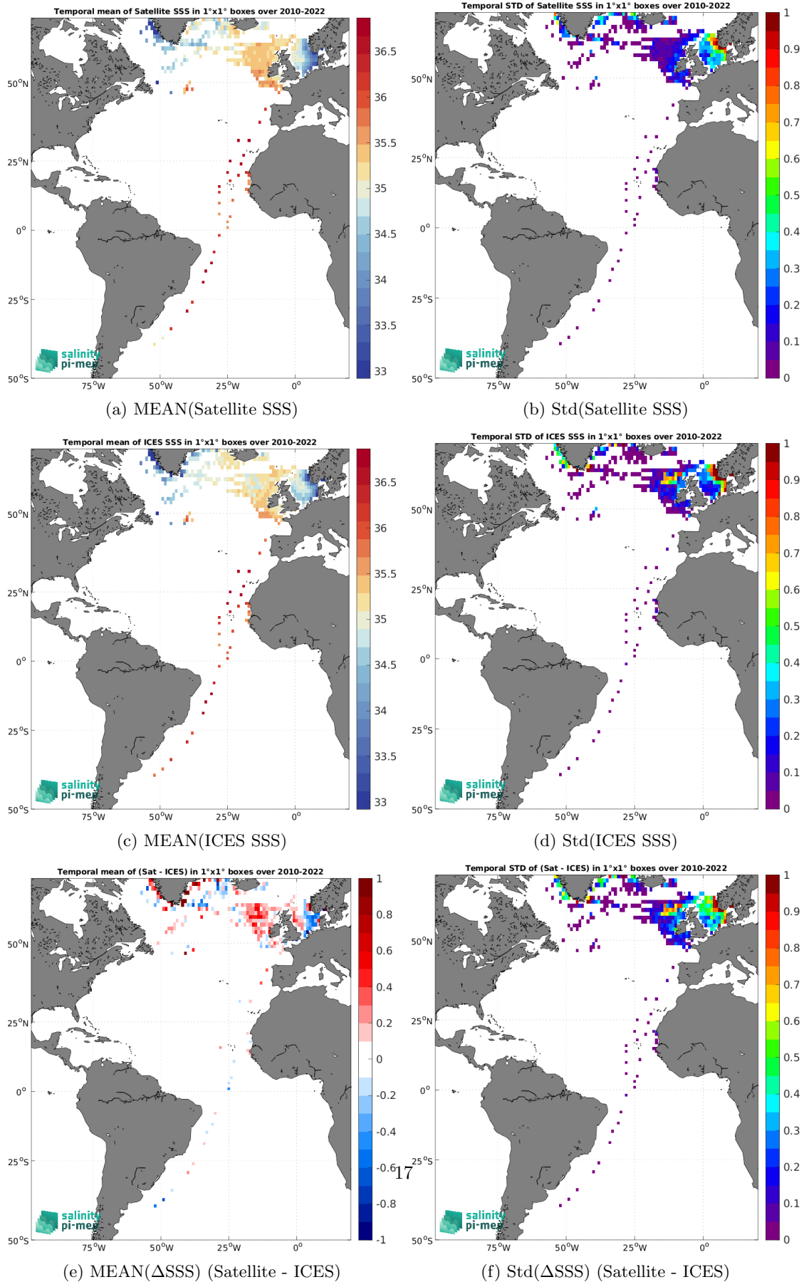
Figure 7: Temporal mean (left) and Std (right) of SSS from CCI SSS L4 Merged-OI v4.41 - 7-day running (ESA) (top), ICES (middle), and of \Delta SSS (Satellite - ICES). Only match-up pairs are used to generate these maps.
