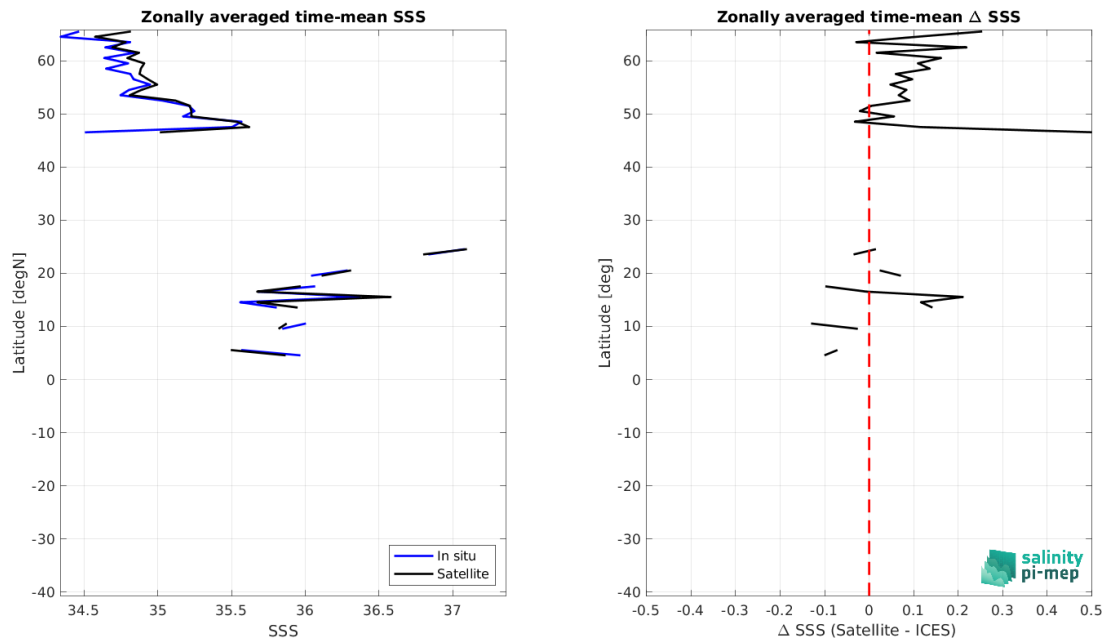
Figure 9: Left panel: Zonal mean SSS from CCI SSS L4 Merged-OI v4.41 - 7-day running (ESA) satellite product (black) and from ICES (blue). Right panel: Zonal mean of \Delta SSS (Satellite - ICES) for all the collected Pi-MEP match-up pairs estimated over the full satellite product period.
