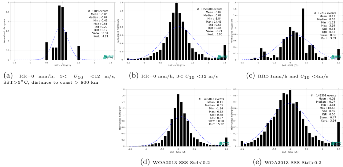
Figure 15: Normalized histogram of \Delta SSS (CCI SSS L4 Merged-OI v4.41 - 7-day running (ESA) - ICES) for 5 different subdatasets corresponding to: RR=0 mm/h, 3 < U_{10} < 12 m/s, SST > 5°C, distance to coast > 800 km (a), RR=0 mm/h, 3 < U_{10} < 12 m/s (b), RR > 1mm/h and U_{10} < 4 m/s (c), WOA2013 SSS Std < 0.2 (d), WOA2013 SSS Std > 0.2 (e).
