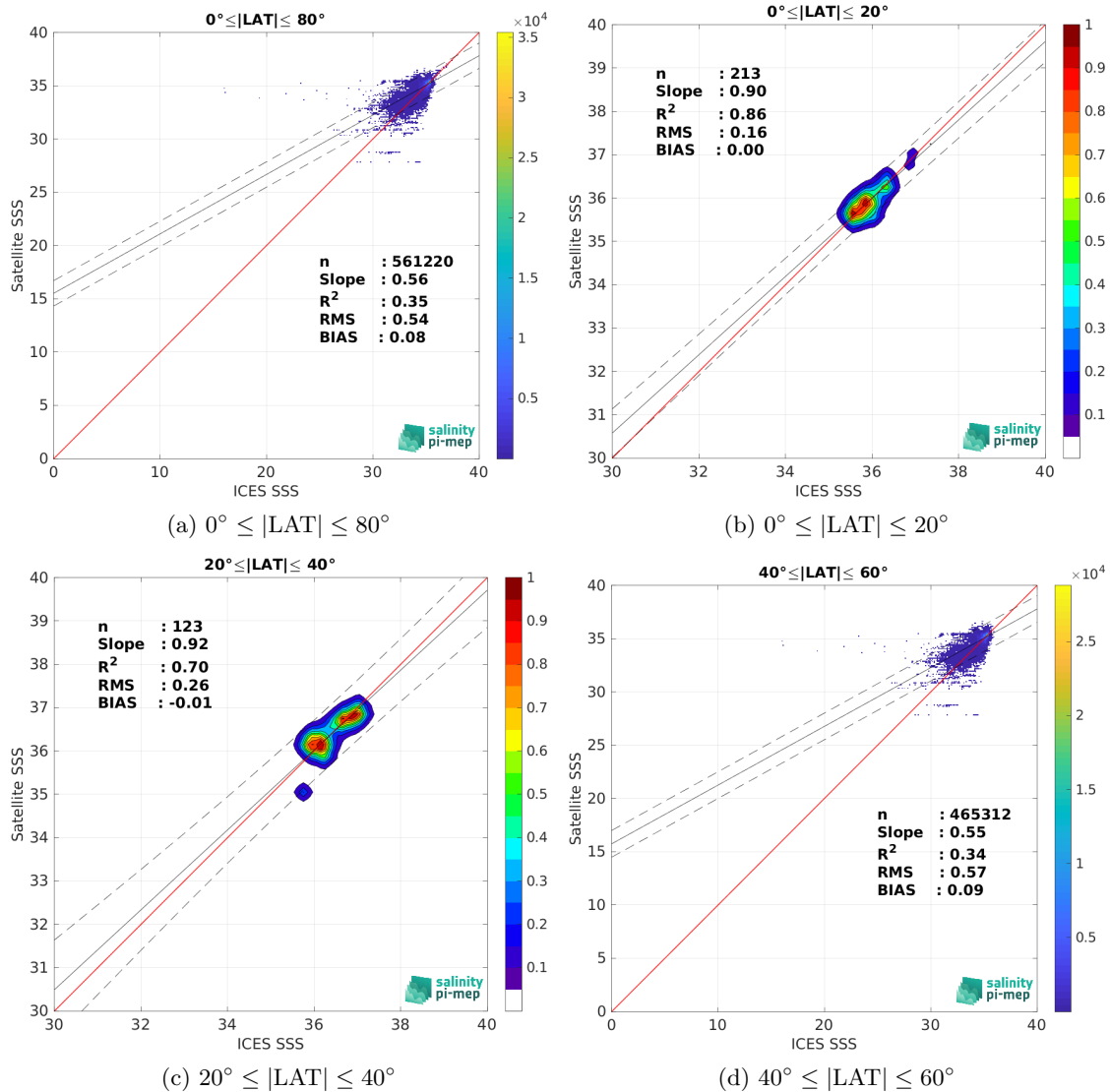
Figure 10: Contour maps of the concentration of CCI SSS L4 Merged-OI v4.41 - 7-day running (ESA) SSS (y-axis) versus ICES SSS (x-axis) at match-up pairs for different latitude bands. For each plot, the red line shows x=y . The black thin and dashed lines indicate a linear fit through the data cloud and the \pm 95\% confidence levels, respectively. The number match-up pairs n , the slope and R^2 coefficient of the linear fit, the root mean square (RMS) and the mean bias between satellite and in situ data are indicated for each latitude band in each plots.
