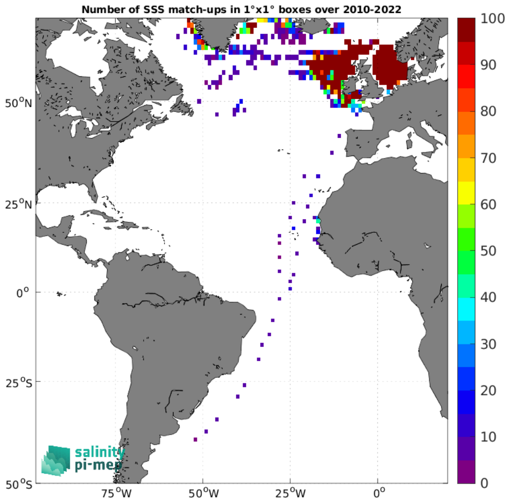
Figure 5: Number of SSS match-ups between ICES SSS and the CCI SSS L4 Merged-OI v4.41 - 7-day running (ESA) SSS product for the Atlantic Ocean Pi-MEP region over 1^\circ \times 1^\circ boxes and for the full satellite product period.
