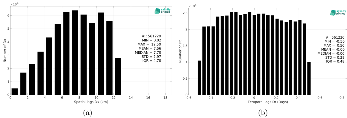
Figure 6: Histograms of the spatial (a) and temporal (b) lags between the location/time of the ICES measurement and the date of the corresponding CCI SSS L4 Merged-OI v4.41 - 7-day running (ESA) SSS pixel.
