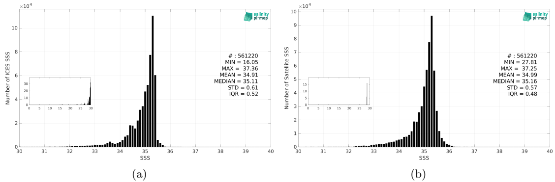
Figure 3: Histograms of SSS from ICES (a) and CCI SSS L4 Merged-OI v4.41 - 7-day running (ESA) (b) considering all match-up pairs per bins of 0.1 over the Atlantic Ocean Pi-MEP region and for the full satellite product period.
