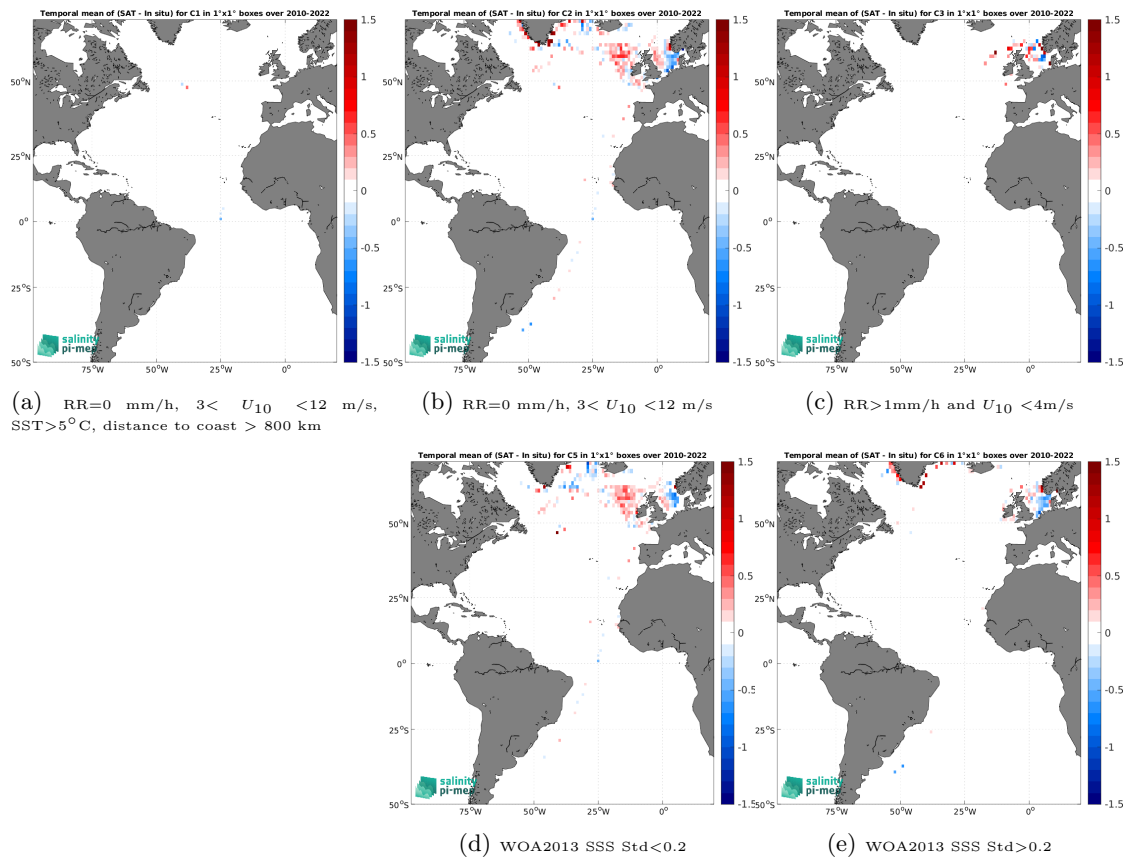
Figure 14: Temporal mean gridded over spatial boxes of size 1^\circ \times 1^\circ of \Delta\text{SSS} (CCI SSS L4 Merged-OI v4.41 - 7-day running (ESA) - ICES) for 5 different subdatasets corresponding to:RR=0 mm/h, 3 < U_{10} < 12 m/s, SST>5°C, distance to coast > 800 km (a), RR=0 mm/h, 3 < U_{10} < 12 m/s (b), RR>1mm/h and U_{10} < 4 m/s (c), WOA2013 SSS Std<0.2 (d), WOA2013 SSS Std>0.2 (e).
