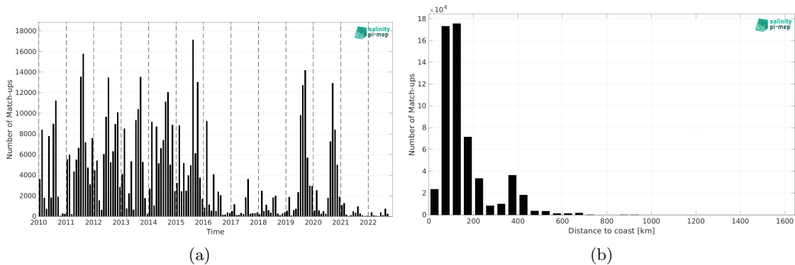
Figure 2: Number of match-ups between ICES and CCI SSS L4 Merged-OI v4.41 - 7-day running (ESA) SSS as a function of time (a) and as function of the distance to coast (b) over the Atlantic Ocean Pi-MEP region and for the full satellite product period.
