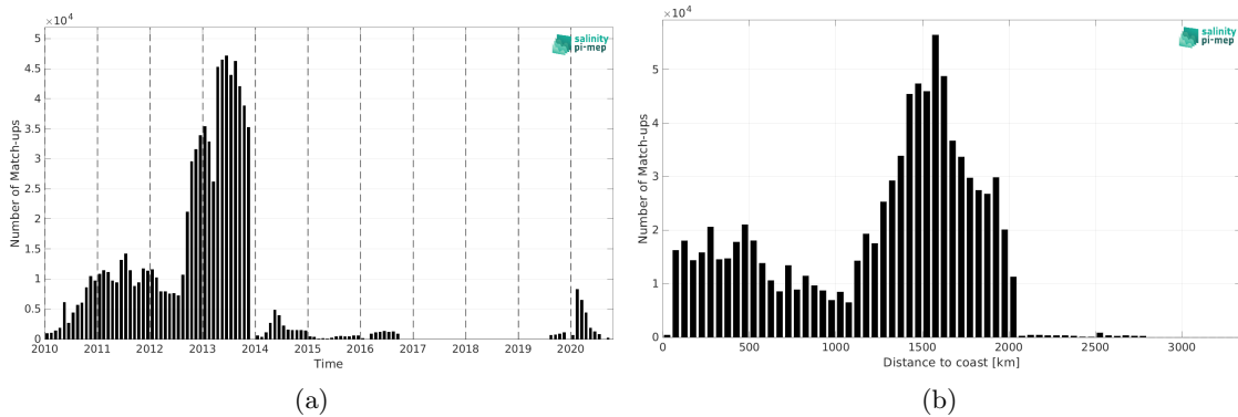
Figure 2: Number of match-ups between Surface drifters and CCI SSS L4 Merged-OI v4.41 - 7-day running (ESA) SSS as a function of time (a) and as function of the distance to coast (b) over the Atlantic Ocean Pi-MEP region and for the full satellite product period.
