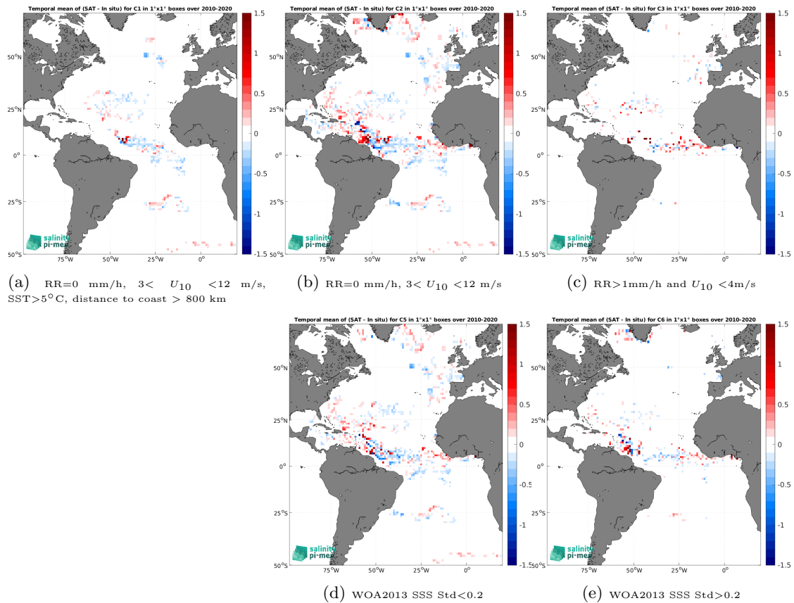
Figure 13: Temporal mean gridded over spatial boxes of size 1^\circ \times 1^\circ of \Delta\text{SSS} (CCI SSS L4 Merged-OI v4.41 - 7-day running (ESA) - Surface drifters) for 5 different subdatasets corresponding to:RR=0 mm/h, 3 < U_{10} < 12 m/s, SST >5^\circ\text{C} , distance to coast > 800 km (a), RR=0 mm/h, 3 < U_{10} < 12 m/s (b), RR >1 mm/h and U_{10} < 4 m/s (c), WOA2013 SSS Std <0.2 (d), WOA2013 SSS Std >0.2 (e).
