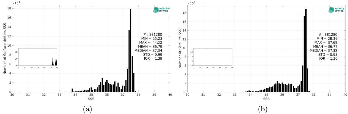
Figure 3: Histograms of SSS from Surface drifters (a) and CCI SSS L4 Merged-OI v4.41 - 7-day running (ESA) (b) considering all match-up pairs per bins of 0.1 over the Atlantic Ocean Pi-MEP region and for the full satellite product period.
