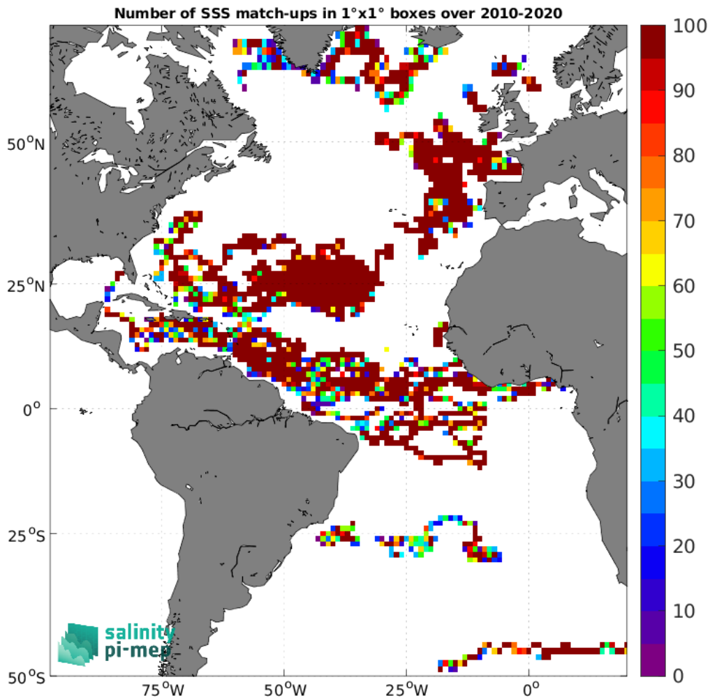
Figure 4: Number of SSS match-ups between Surface drifters SSS and the CCI SSS L4 Merged-OI v4.41 - 7-day running (ESA) SSS product for the Atlantic Ocean Pi-MEP region over 1^\circ \times 1^\circ boxes and for the full satellite product period.
