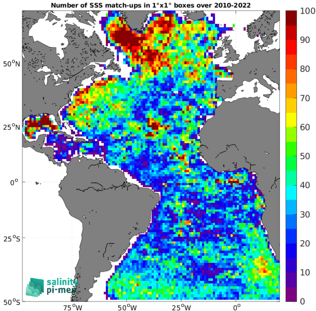
Figure 5: Number of SSS match-ups between Argo SSS and the CCI SSS L4 Merged-OI v4.41 - 7-day running (ESA) SSS product for the Atlantic Ocean Pi-MEP region over 1^\circ \times 1^\circ boxes and for the full satellite product period.
