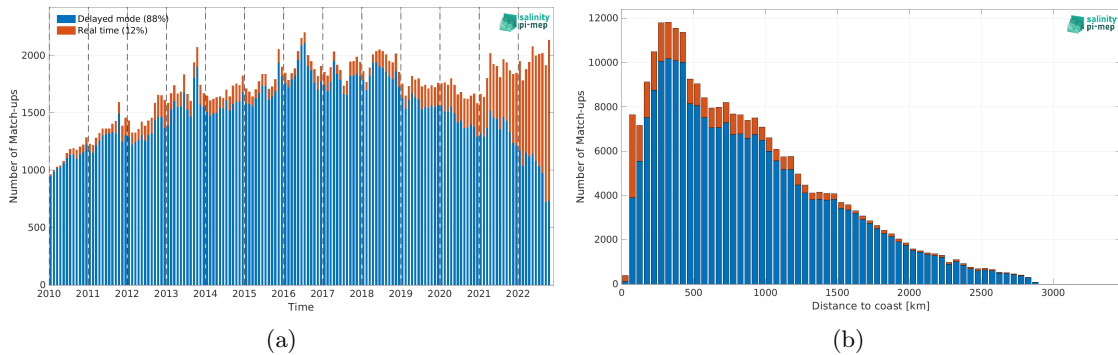
Figure 2: Number of match-ups between Argo and CCI SSS L4 Merged-OI v4.41 - 7-day running (ESA) SSS as a function of time (a) and as function of the distance to coast (b) over the Atlantic Ocean Pi-MEP region and for the full satellite product period.
