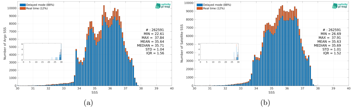
Figure 3: Histograms of SSS from Argo (a) and CCI SSS L4 Merged-OI v4.41 - 7-day running (ESA) (b) considering all match-up pairs per bins of 0.1 over the Atlantic Ocean Pi-MEP region and for the full satellite product period.
