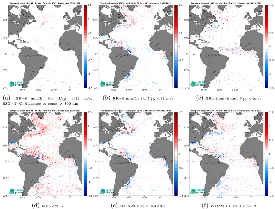
Figure 14: Temporal mean gridded over spatial boxes of size 1^\circ \times 1^\circ of \Delta\text{SSS} (CCI SSS L4 Merged-OI v4.41 - 7-day running (ESA) - Argo) for 6 different subdatasets corresponding to:RR=0 mm/h, 3 < U_{10} < 12 m/s, SST>5°C, distance to coast > 800 km (a), RR=0 mm/h, 3 < U_{10} < 12 m/s (b), RR>1mm/h and U_{10} < 4 m/s (c),MLD<20m (d),WOA2013 SSS Std<0.2 (e),WOA2013 SSS Std>0.2 (f).
