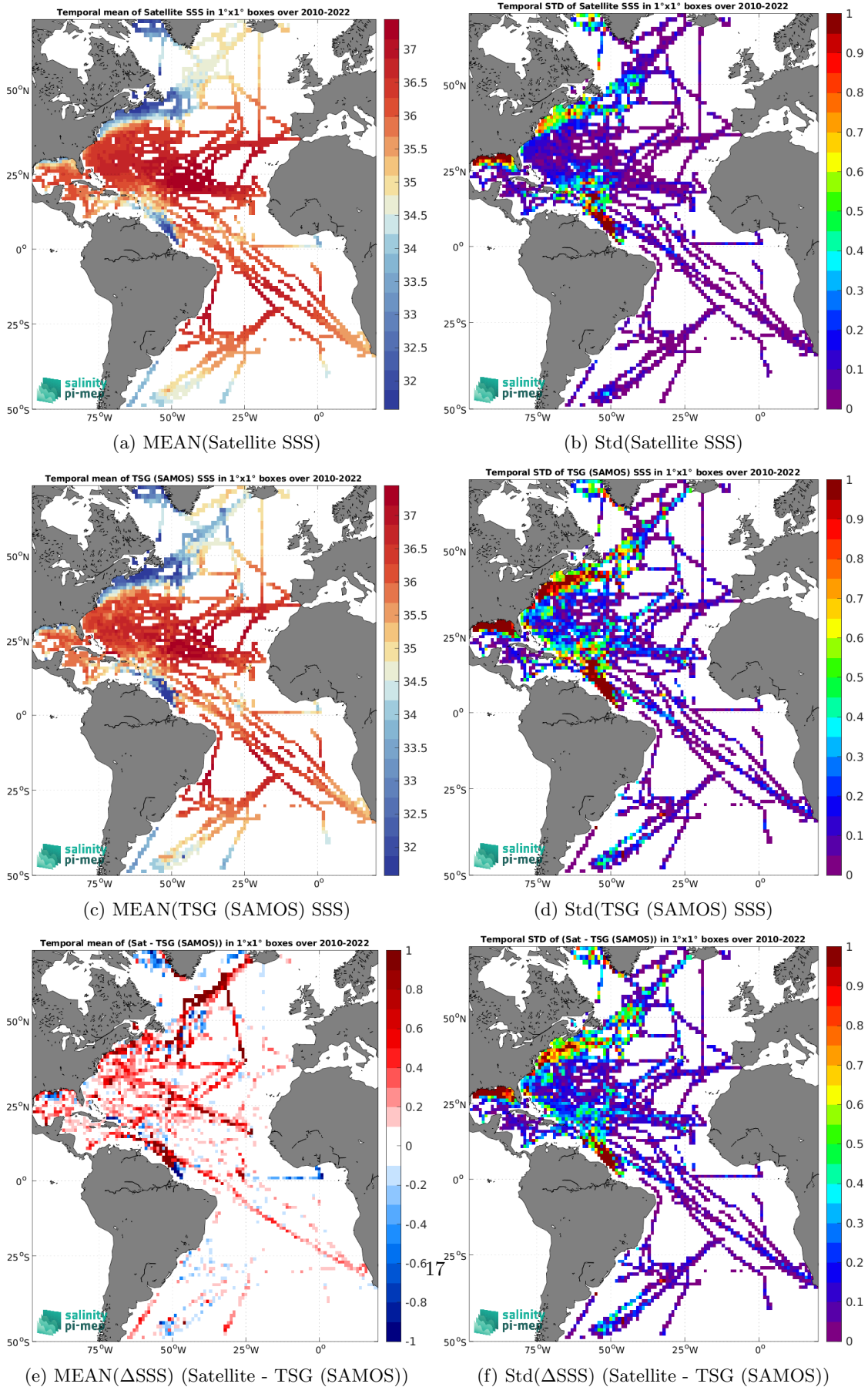
Figure 7: Temporal mean (left) and Std (right) of SSS from CCI SSS L4 Merged-OI v4.41 - 30-day running (ESA) (top), TSG (SAMOS) (middle), and of \Delta SSS (Satellite - TSG (SAMOS)). Only match-up pairs are used to generate these maps.
