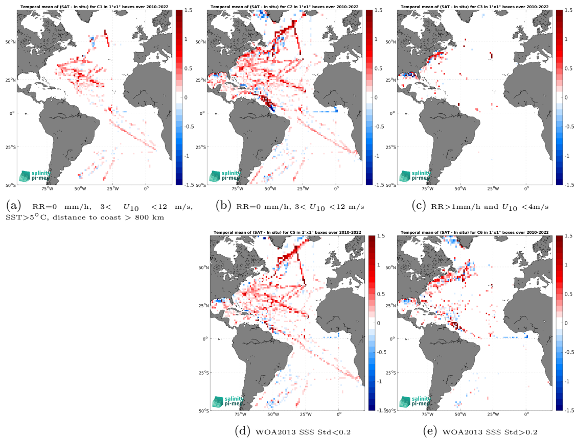
Figure 14: Temporal mean gridded over spatial boxes of size 1^\circ \times 1^\circ of \Delta\text{SSS} (CCI SSS L4 Merged-OI v4.41 - 30-day running (ESA) - TSG (SAMOS)) for 5 different subdatasets corresponding to:RR=0 mm/h, 3 < U_{10} < 12 m/s, SST>5°C, distance to coast > 800 km (a), RR=0 mm/h, 3 < U_{10} < 12 m/s (b), RR>1mm/h and U_{10} < 4 m/s (c), WOA2013 SSS Std<0.2 (d), WOA2013 SSS Std>0.2 (e).
