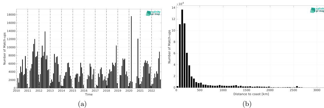
Figure 2: Number of match-ups between TSG (SAMOS) and CCI SSS L4 Merged-OI v4.41 - 30-day running (ESA) SSS as a function of time (a) and as function of the distance to coast (b) over the Atlantic Ocean Pi-MEP region and for the full satellite product period.
