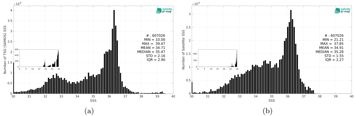
Figure 3: Histograms of SSS from TSG (SAMOS) (a) and CCI SSS L4 Merged-OI v4.41 - 30-day running (ESA) (b) considering all match-up pairs per bins of 0.1 over the Atlantic Ocean Pi-MEP region and for the full satellite product period.
