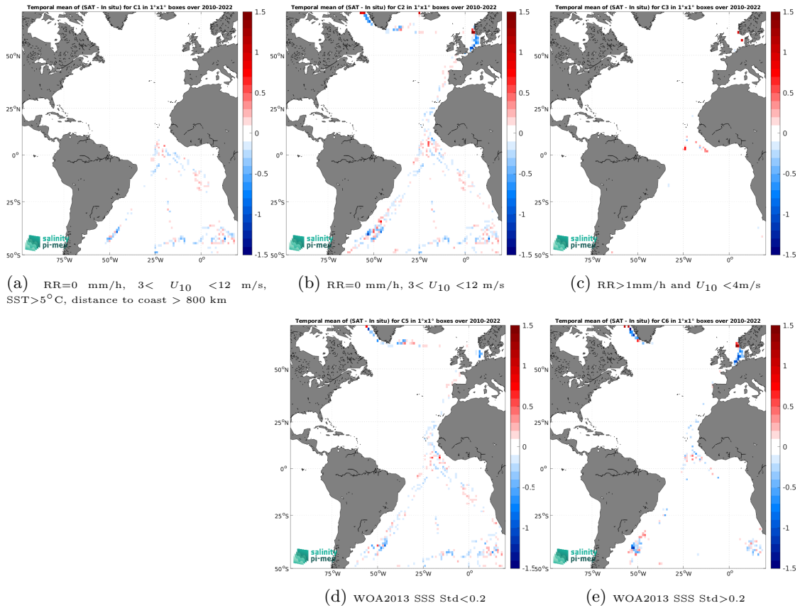
Figure 14: Temporal mean gridded over spatial boxes of size 1^\circ \times 1^\circ of \Delta\text{SSS} (CCI SSS L4 Merged-OI v4.41 - 30-day running (ESA) - TSG (Polarstern)) for 5 different subdatasets corresponding to:RR=0 mm/h, 3 < U_{10} < 12 m/s, SST>5°C, distance to coast > 800 km (a), RR=0 mm/h, 3 < U_{10} < 12 m/s (b), RR>1mm/h and U_{10} < 4 m/s (c), WOA2013 SSS Std<0.2 (d), WOA2013 SSS Std>0.2 (e).
