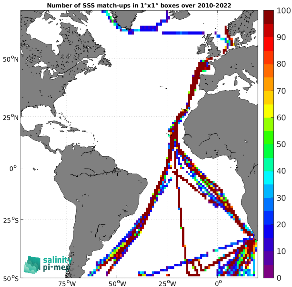
Figure 5: Number of SSS match-ups between TSG (Polarstern) SSS and the CCI SSS L4 Merged-OI v4.41 - 30-day running (ESA) SSS product for the Atlantic Ocean Pi-MEP region over 1°×1° boxes and for the full satellite product period.
