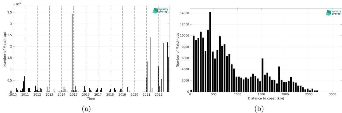
Figure 2: Number of match-ups between TSG (Polarstern) and CCI SSS L4 Merged-OI v4.41 - 30-day running (ESA) SSS as a function of time (a) and as function of the distance to coast (b) over the Atlantic Ocean Pi-MEP region and for the full satellite product period.
