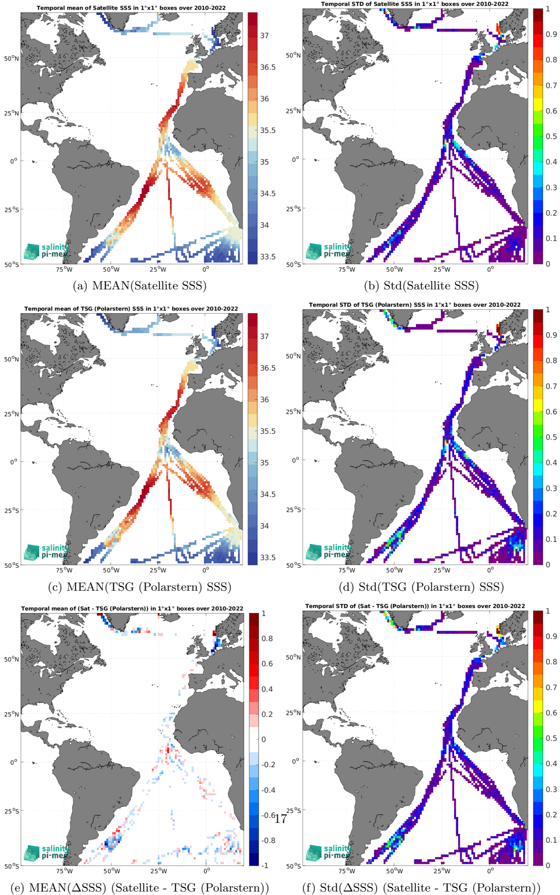
Figure 7: Temporal mean (left) and Std (right) of SSS from CCI SSS L4 Merged-OI v4.41 - 30-day running (ESA) (top), TSG (Polarstern) (middle), and of \Delta SSS (Satellite - TSG (Polarstern)). Only match-up pairs are used to generate these maps.
