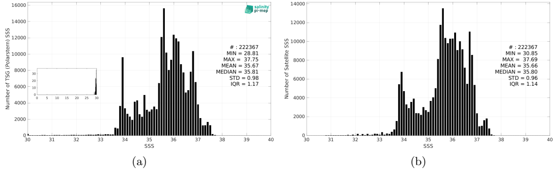
Figure 3: Histograms of SSS from TSG (Polarstern) (a) and CCI SSS L4 Merged-OI v4.41 - 30-day running (ESA) (b) considering all match-up pairs per bins of 0.1 over the Atlantic Ocean Pi-MEP region and for the full satellite product period.
