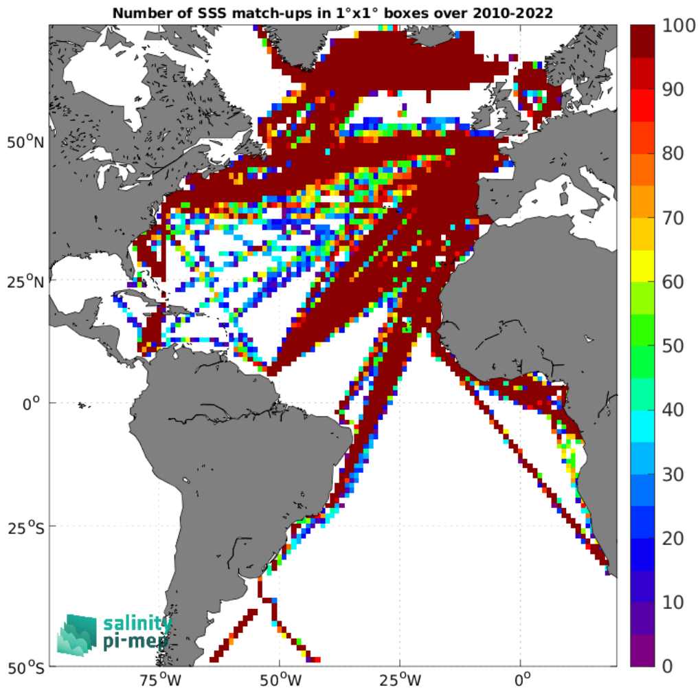
Figure 5: Number of SSS match-ups between TSG (LEGOS-DM) SSS and the CCI SSS L4 Merged-OI v4.41 - 30-day running (ESA) SSS product for the Atlantic Ocean Pi-MEP region over 1^\circ \times 1^\circ boxes and for the full satellite product period.
