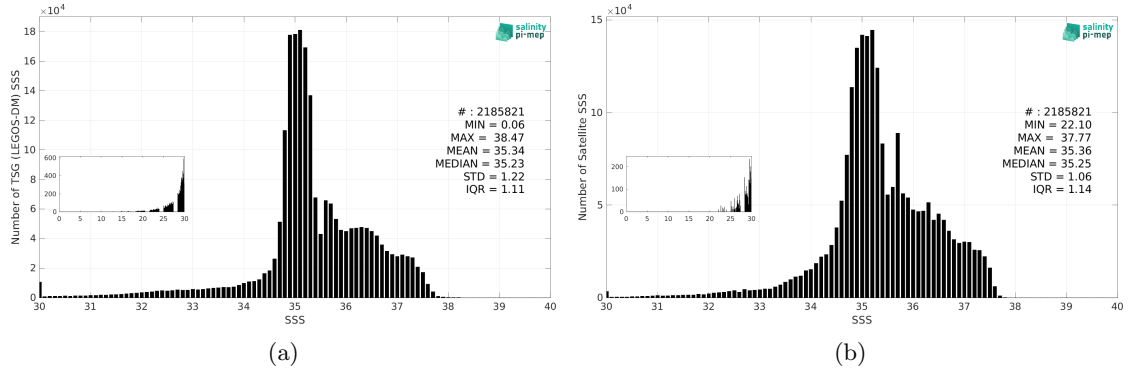
Figure 3: Histograms of SSS from TSG (LEGOS-DM) (a) and CCI SSS L4 Merged-OI v4.41 - 30-day running (ESA) (b) considering all match-up pairs per bins of 0.1 over the Atlantic Ocean Pi-MEP region and for the full satellite product period.
