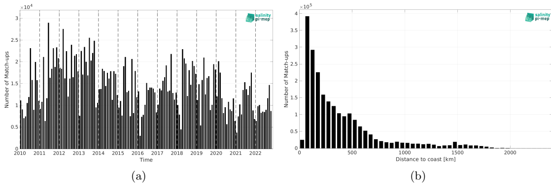
Figure 2: Number of match-ups between TSG (LEGOS-DM) and CCI SSS L4 Merged-OI v4.41 - 30-day running (ESA) SSS as a function of time (a) and as function of the distance to coast (b) over the Atlantic Ocean Pi-MEP region and for the full satellite product period.
