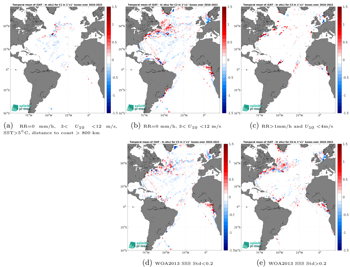
Figure 14: Temporal mean gridded over spatial boxes of size 1^\circ \times 1^\circ of \Delta\text{SSS} (CCI SSS L4 Merged-OI v4.41 - 30-day running (ESA) - TSG (LEGOS-DM)) for 5 different subdatasets corresponding to:RR=0 mm/h, 3 < U_{10} < 12 m/s, SST>5°C, distance to coast > 800 km (a), RR=0 mm/h, 3 < U_{10} < 12 m/s (b), RR>1mm/h and U_{10} < 4 m/s (c), WOA2013 SSS Std<0.2 (d), WOA2013 SSS Std>0.2 (e).
