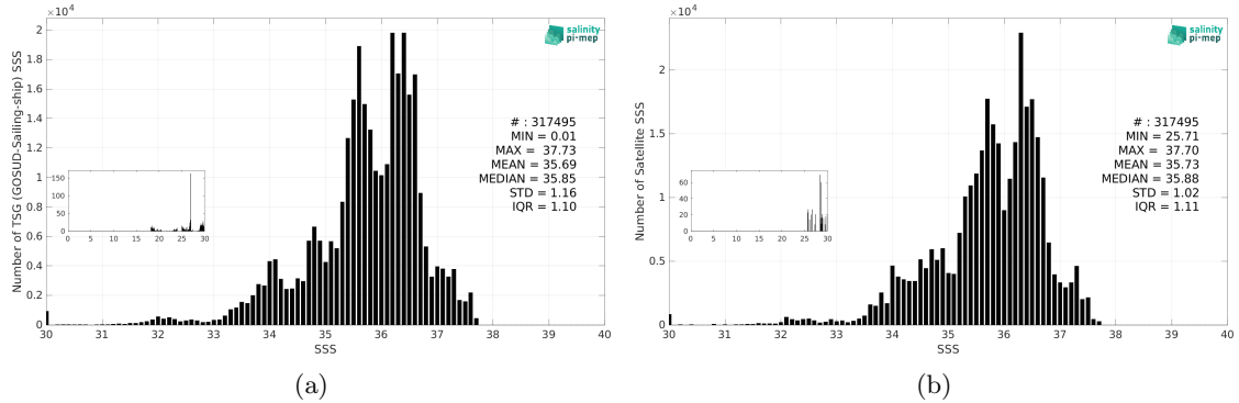
Figure 3: Histograms of SSS from TSG (GOSUD-Sailing-ship) (a) and CCI SSS L4 Merged-OI v4.41 - 30-day running (ESA) (b) considering all match-up pairs per bins of 0.1 over the Atlantic Ocean Pi-MEP region and for the full satellite product period.
