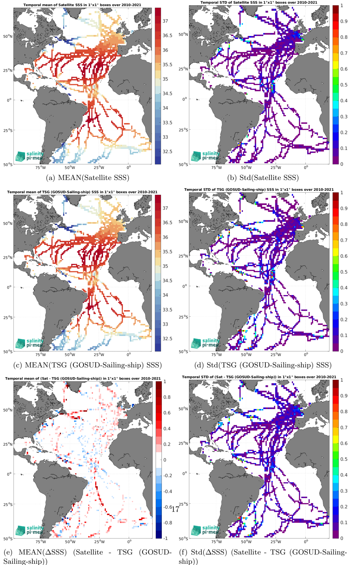
Figure 7: Temporal mean (left) and Std (right) of SSS from CCI SSS L4 Merged-OI v4.41 - 30-day running (ESA) (top), TSG (GOSUD-Sailing-ship) (middle), and of \Delta SSS (Satellite - TSG (GOSUD-Sailing-ship)). Only match-up pairs are used to generate these maps.
