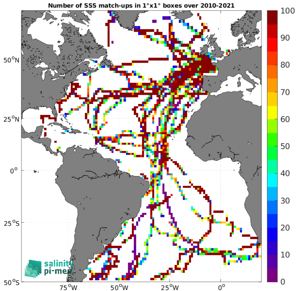
Figure 5: Number of SSS match-ups between TSG (GOSUD-Sailing-ship) SSS and the CCI SSS L4 Merged-OI v4.41 - 30-day running (ESA) SSS product for the Atlantic Ocean Pi-MEP region over 1^\circ \times 1^\circ boxes and for the full satellite product period.
