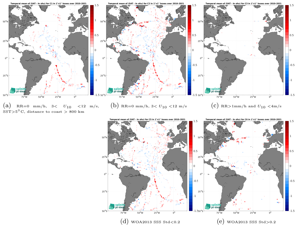
Figure 14: Temporal mean gridded over spatial boxes of size 1^\circ \times 1^\circ of \Delta\text{SSS} (CCI SSS L4 Merged-OI v4.41 - 30-day running (ESA) - TSG (GOSUD-Sailing-ship)) for 5 different subdatasets corresponding to:RR=0 mm/h, 3 < U_{10} < 12 m/s, SST>5°C, distance to coast > 800 km (a), RR=0 mm/h, 3 < U_{10} < 12 m/s (b), RR>1mm/h and U_{10} < 4 m/s (c), WOA2013 SSS Std<0.2 (d), WOA2013 SSS Std>0.2 (e).
