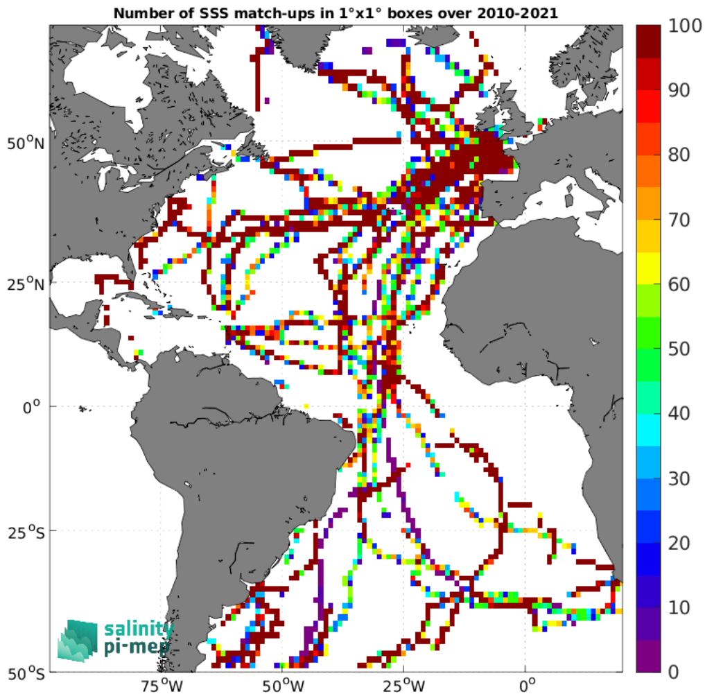
Figure 5: Number of SSS match-ups between TSG (GOSUD-Sailing-ship) SSS and the CCI SSS L4 Merged-OI v4.41 - 30-day running (ESA) SSS product for the Atlantic Ocean Pi-MEP region over 1°x1° boxes and for the full satellite product period.
