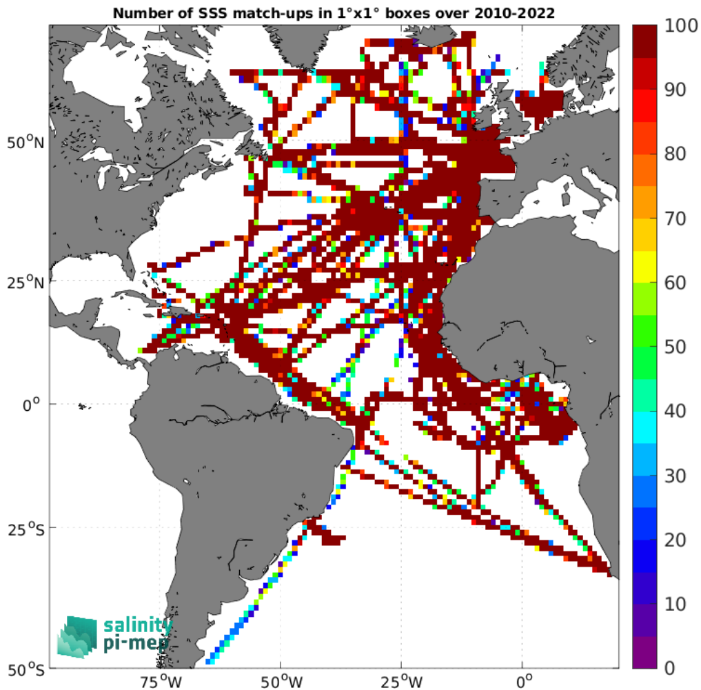
Figure 5: Number of SSS match-ups between TSG (GOSUD-Research-vessel) SSS and the CCI SSS L4 Merged-OI v4.41 - 30-day running (ESA) SSS product for the Atlantic Ocean Pi-MEP region over 1^{\circ} \times 1^{\circ} boxes and for the full satellite product period.
