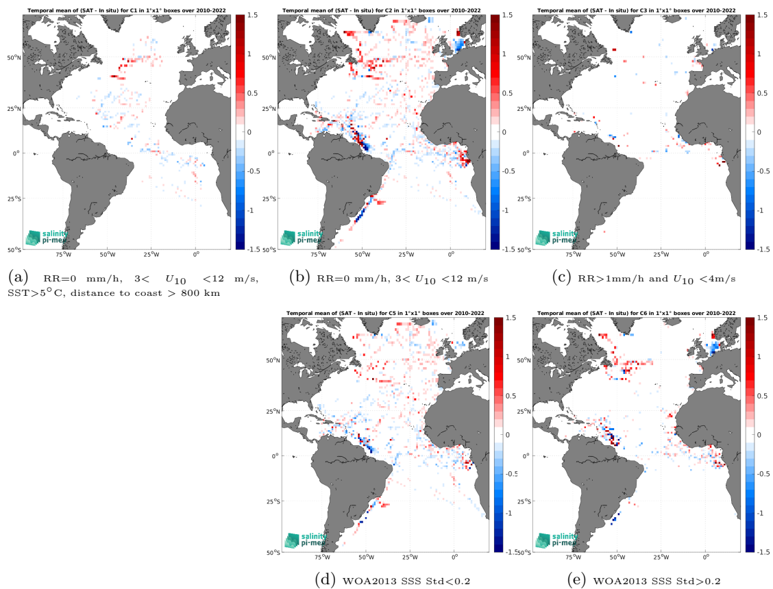
Figure 14: Temporal mean gridded over spatial boxes of size 1^\circ \times 1^\circ of \Delta\text{SSS} (CCI SSS L4 Merged-OI v4.41 - 30-day running (ESA) - TSG (GOSUD-Research-vessel)) for 5 different subdatasets corresponding to:RR=0 mm/h, 3 < U_{10} < 12 m/s, SST>5°C, distance to coast > 800 km (a), RR=0 mm/h, 3 < U_{10} < 12 m/s (b), RR>1mm/h and U_{10} < 4 m/s (c), WOA2013 SSS Std<0.2 (d), WOA2013 SSS Std>0.2 (e).
