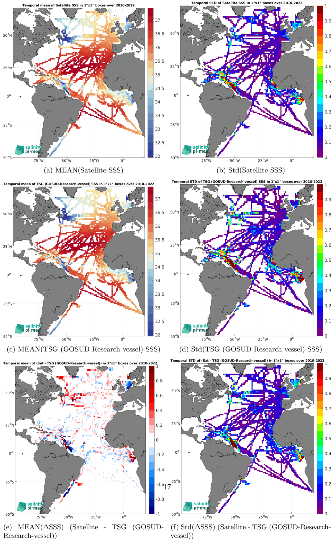
Figure 7: Temporal mean (left) and Std (right) of SSS from CCI SSS L4 Merged-OI v4.41 - 30-day running (ESA) (top), TSG (GOSUD-Research-vessel) (middle), and of \Delta SSS (Satellite - TSG (GOSUD-Research-vessel)). Only match-up pairs are used to generate these maps.
