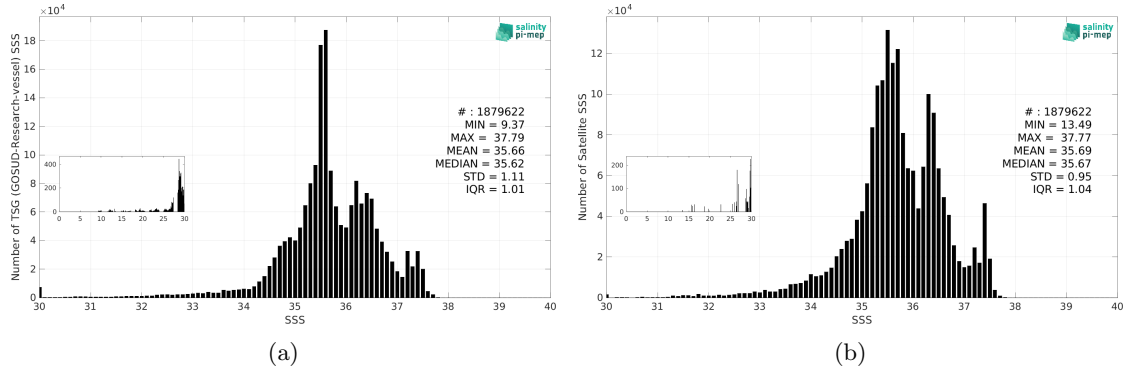
Figure 3: Histograms of SSS from TSG (GOSUD-Research-vessel) (a) and CCI SSS L4 Merged-OI v4.41 - 30-day running (ESA) (b) considering all match-up pairs per bins of 0.1 over the Atlantic Ocean Pi-MEP region and for the full satellite product period.
