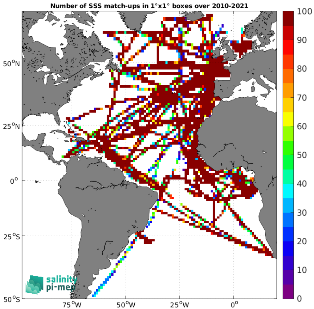
Figure 5: Number of SSS match-ups between TSG (GOSUD-Research-vessel) SSS and the CCI SSS L4 Merged-OI v4.41 - 30-day running (ESA) SSS product for the Atlantic Ocean Pi-MEP region over 1^\circ \times 1^\circ boxes and for the full satellite product period.
