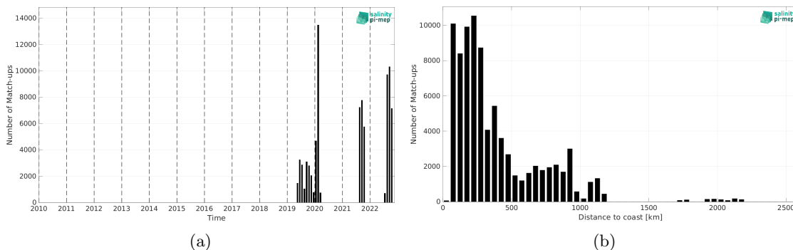
Figure 2: Number of match-ups between Saildrone and CCI SSS L4 Merged-OI v4.41 - 30-day running (ESA) SSS as a function of time (a) and as function of the distance to coast (b) over the Atlantic Ocean Pi-MEP region and for the full satellite product period.
