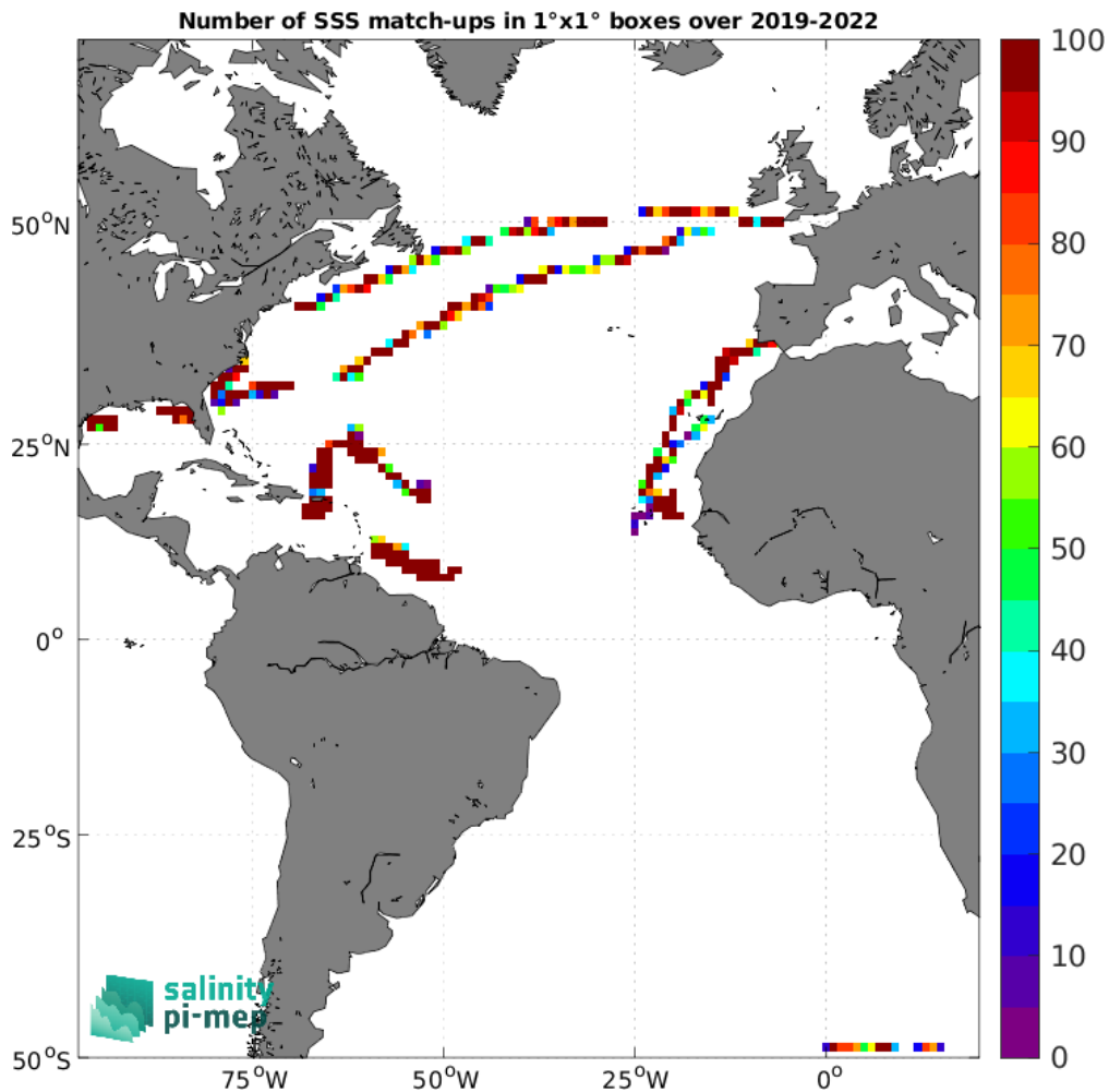
Figure 5: Number of SSS match-ups between Saildrone SSS and the CCI SSS L4 Merged-OI v4.41 - 30-day running (ESA) SSS product for the Atlantic Ocean Pi-MEP region over 1^\circ \times 1^\circ boxes and for the full satellite product period.
