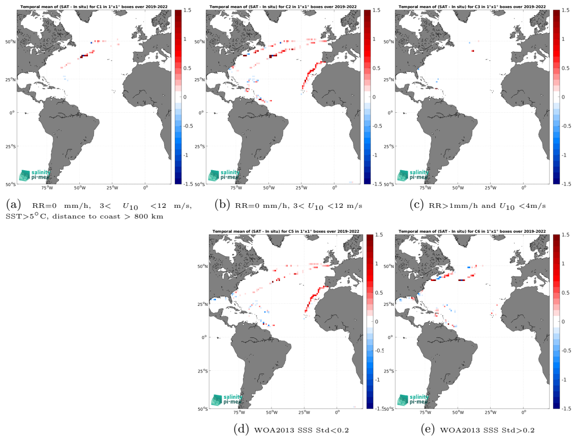
Figure 14: Temporal mean gridded over spatial boxes of size 1^\circ \times 1^\circ of \Delta\text{SSS} (CCI SSS L4 Merged-OI v4.41 - 30-day running (ESA) - Saildrone) for 5 different subdatasets corresponding to:RR=0 mm/h, 3 < U_{10} < 12 m/s, SST>5°C, distance to coast > 800 km (a), RR=0 mm/h, 3 < U_{10} < 12 m/s (b), RR>1mm/h and U_{10} < 4 m/s (c), WOA2013 SSS Std<0.2 (d), WOA2013 SSS Std>0.2 (e).
