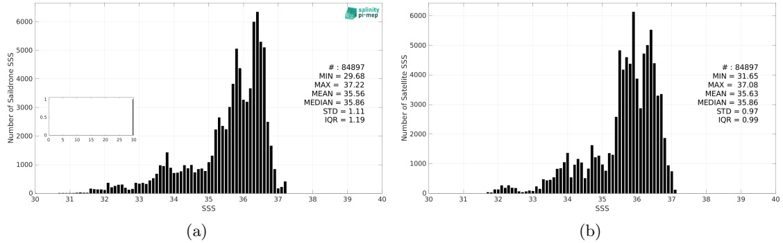
Figure 3: Histograms of SSS from Saiclone (a) and CCI SSS L4 Merged-OI v4.41 - 30-day running (ESA) (b) considering all match-up pairs per bins of 0.1 over the Atlantic Ocean Pi-MEP region and for the full satellite product period.
