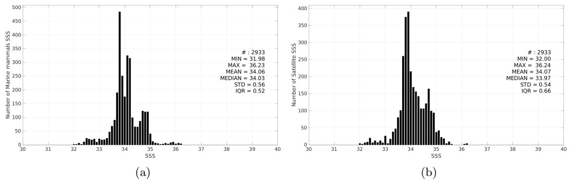
Figure 3: Histograms of SSS from Marine mammals (a) and CCI SSS L4 Merged-OI v4.41 - 30-day running (ESA) (b) considering all match-up pairs per bins of 0.1 over the Atlantic Ocean Pi-MEP region and for the full satellite product period.
