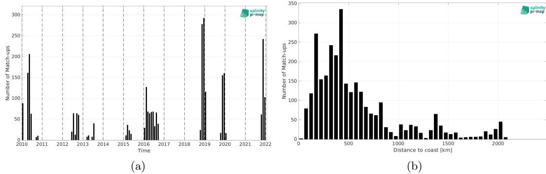
Figure 2: Number of match-ups between Marine mammals and CCI SSS L4 Merged-OI v4.41 - 30-day running (ESA) SSS as a function of time (a) and as function of the distance to coast (b) over the Atlantic Ocean Pi-MEP region and for the full satellite product period.
