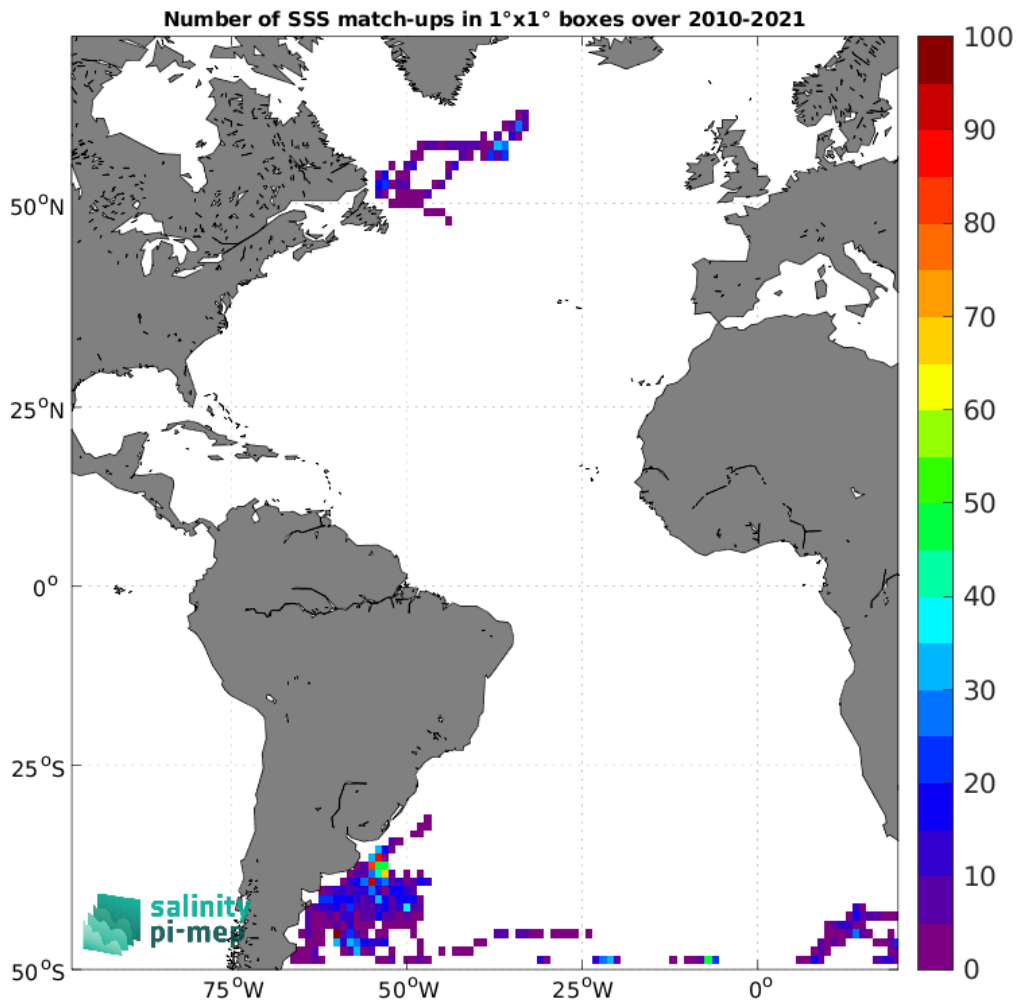
Figure 5: Number of SSS match-ups between Marine mammals SSS and the CCI SSS L4 Merged-OI v4.41 - 30-day running (ESA) SSS product for the Atlantic Ocean Pi-MEP region over 1°×1° boxes and for the full satellite product period.
