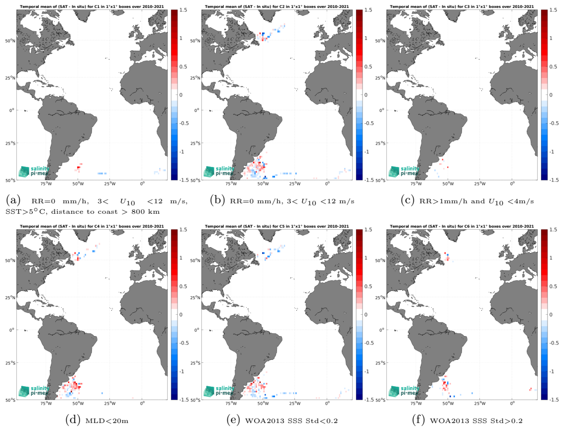
Figure 14: Temporal mean gridded over spatial boxes of size 1^\circ \times 1^\circ of \Delta SSS (CCI SSS L4 Merged-OI v4.41 - 30-day running (ESA) - Marine mammals) for 6 different subdatasets corresponding to:RR=0 mm/h, 3 < U_{10} < 12 m/s, SST >5^\circ C, distance to coast > 800 km (a), RR=0 mm/h, 3 < U_{10} < 12 m/s (b), RR >1 mm/h and U_{10} < 4 m/s (c),MLD <20 m (d),WOA2013 SSS Std <0.2 (e),WOA2013 SSS Std >0.2 (f).
