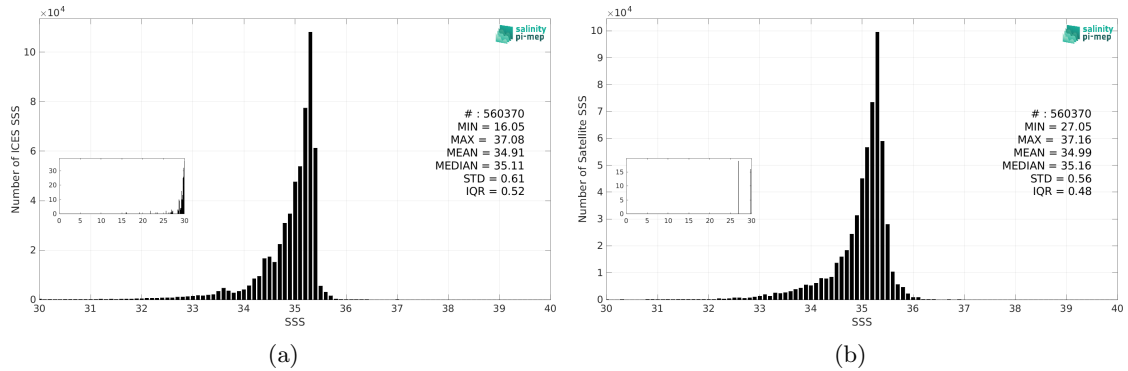
Figure 3: Histograms of SSS from ICES (a) and CCI SSS L4 Merged-OI v4.41 - 30-day running (ESA) (b) considering all match-up pairs per bins of 0.1 over the Atlantic Ocean Pi-MEP region and for the full satellite product period.
