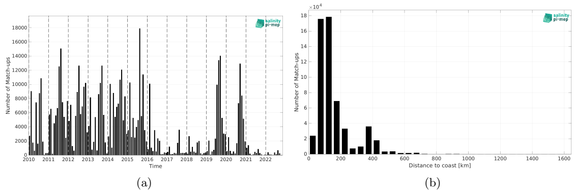
Figure 2: Number of match-ups between ICES and CCI SSS L4 Merged-OI v4.41 - 30-day running (ESA) SSS as a function of time (a) and as function of the distance to coast (b) over the Atlantic Ocean Pi-MEP region and for the full satellite product period.
