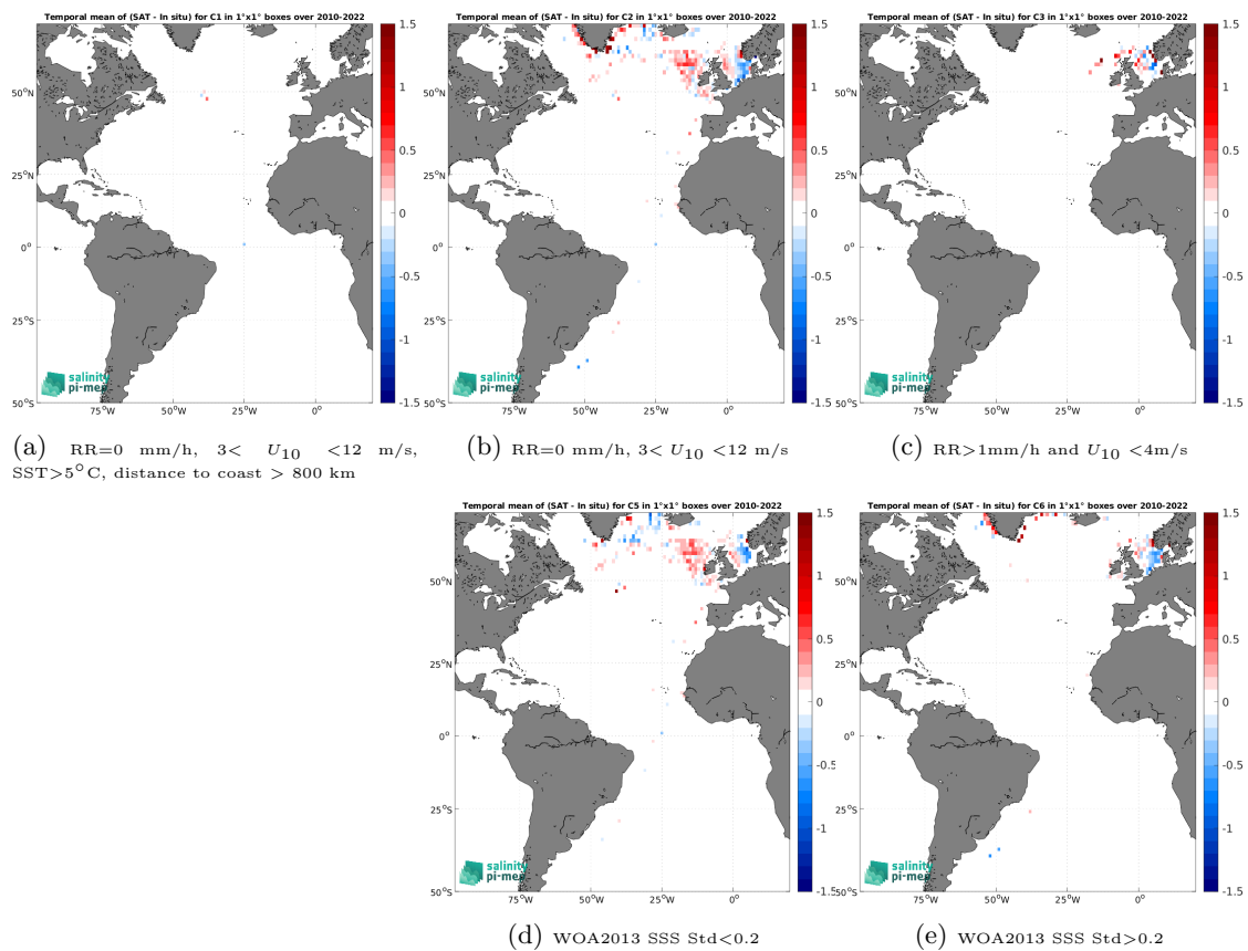
Figure 14: Temporal mean gridded over spatial boxes of size 1^\circ \times 1^\circ of \Delta SSS (CCI SSS L4 Merged-OI v4.41 - 30-day running (ESA) - ICES) for 5 different subdatasets corresponding to:RR=0 mm/h, 3 < U_{10} < 12 m/s, SST >5^\circ\text{C} , distance to coast > 800 km (a), RR=0 mm/h, 3 < U_{10} < 12 m/s (b), RR >1 mm/h and U_{10} < 4 m/s (c), WOA2013 SSS Std <0.2 (d), WOA2013 SSS Std >0.2 (e).
