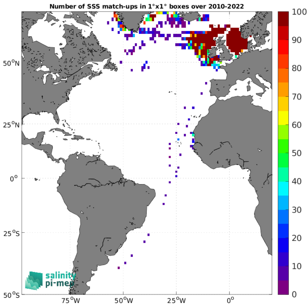
Figure 5: Number of SSS match-ups between ICES SSS and the CCI SSS L4 Merged-OI v4.41 - 30-day running (ESA) SSS product for the Atlantic Ocean Pi-MEP region over 1°×1° boxes and for the full satellite product period.
