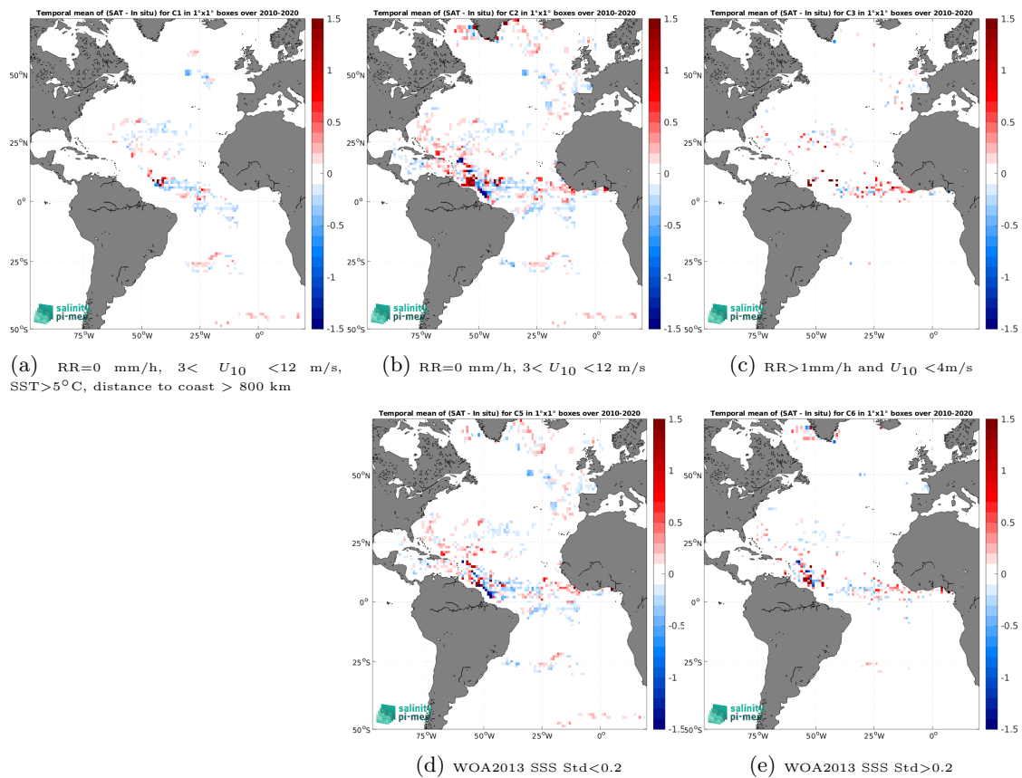
Figure 13: Temporal mean gridded over spatial boxes of size 1^\circ \times 1^\circ of \Delta\text{SSS} (CCI SSS L4 Merged-OI v4.41 - 30-day running (ESA) - Surface drifters) for 5 different subdatasets corresponding to:RR=0 mm/h, 3 < U_{10} < 12 m/s, SST >5^\circ\text{C} , distance to coast > 800 km (a), RR=0 mm/h, 3 < U_{10} < 12 m/s (b), RR >1 mm/h and U_{10} < 4 m/s (c), WOA2013 SSS Std <0.2 (d), WOA2013 SSS Std >0.2 (e).
