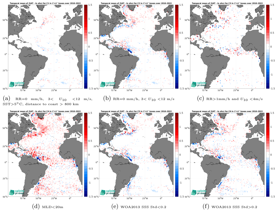
Figure 14: Temporal mean gridded over spatial boxes of size 1^\circ \times 1^\circ of \Delta SSS (CCI SSS L4 Merged-OI v4.41 - 30-day running (ESA) - Argo) for 6 different subdatasets corresponding to:RR=0 mm/h, 3 < U_{10} < 12 m/s, SST >5^\circ C, distance to coast > 800 km (a), RR=0 mm/h, 3 < U_{10} < 12 m/s (b), RR >1 mm/h and U_{10} < 4 m/s (c),MLD <20 m (d),WOA2013 SSS Std <0.2 (e),WOA2013 SSS Std >0.2 (f).
