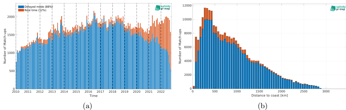
Figure 2: Number of match-ups between Argo and CCI SSS L4 Merged-OI v4.41 - 30-day running (ESA) SSS as a function of time (a) and as function of the distance to coast (b) over the Atlantic Ocean Pi-MEP region and for the full satellite product period.
