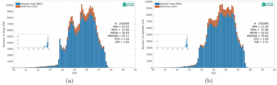
Figure 3: Histograms of SSS from Argo (a) and CCI SSS L4 Merged-OI v4.41 - 30-day running (ESA) (b) considering all match-up pairs per bins of 0.1 over the Atlantic Ocean Pi-MEP region and for the full satellite product period.
