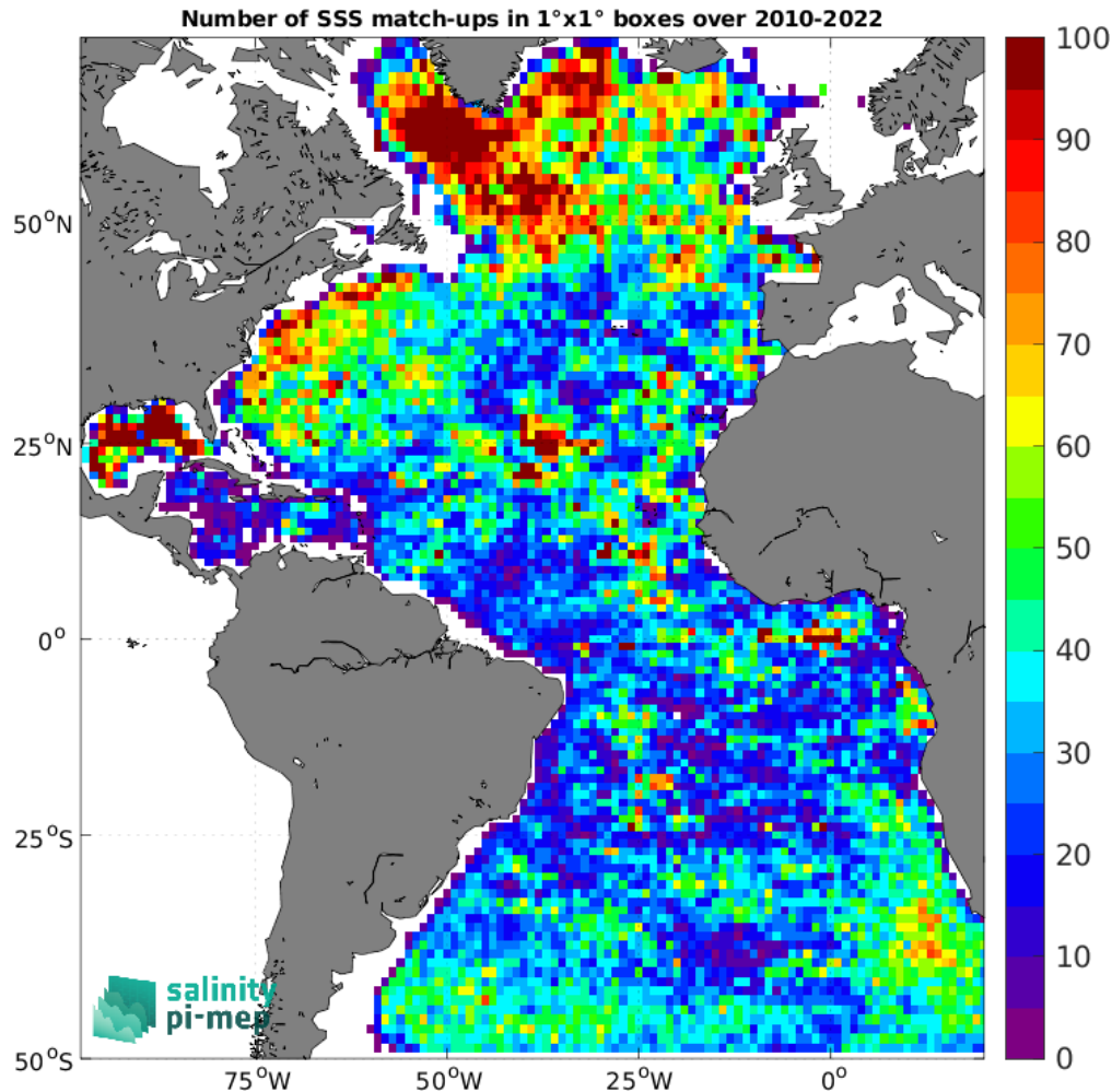
Figure 5: Number of SSS match-ups between Argo SSS and the CCI SSS L4 Merged-OI v4.41 - 30-day running (ESA) SSS product for the Atlantic Ocean Pi-MEP region over 1^\circ \times 1^\circ boxes and for the full satellite product period.
