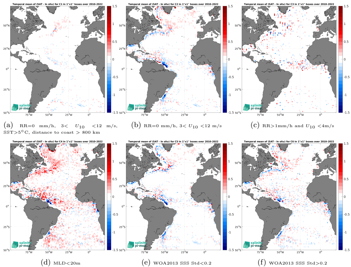
Figure 14: Temporal mean gridded over spatial boxes of size 1^\circ \times 1^\circ of \Delta\text{SSS} (CCI SSS L4 Merged-OI v4.41 - 30-day running (ESA) - Argo) for 6 different subdatasets corresponding to:RR=0 mm/h, 3 < U_{10} < 12 m/s, SST>5°C, distance to coast > 800 km (a), RR=0 mm/h, 3 < U_{10} < 12 m/s (b), RR>1mm/h and U_{10} < 4 m/s (c),MLD<20m (d),WOA2013 SSS Std<0.2 (e),WOA2013 SSS Std>0.2 (f).
