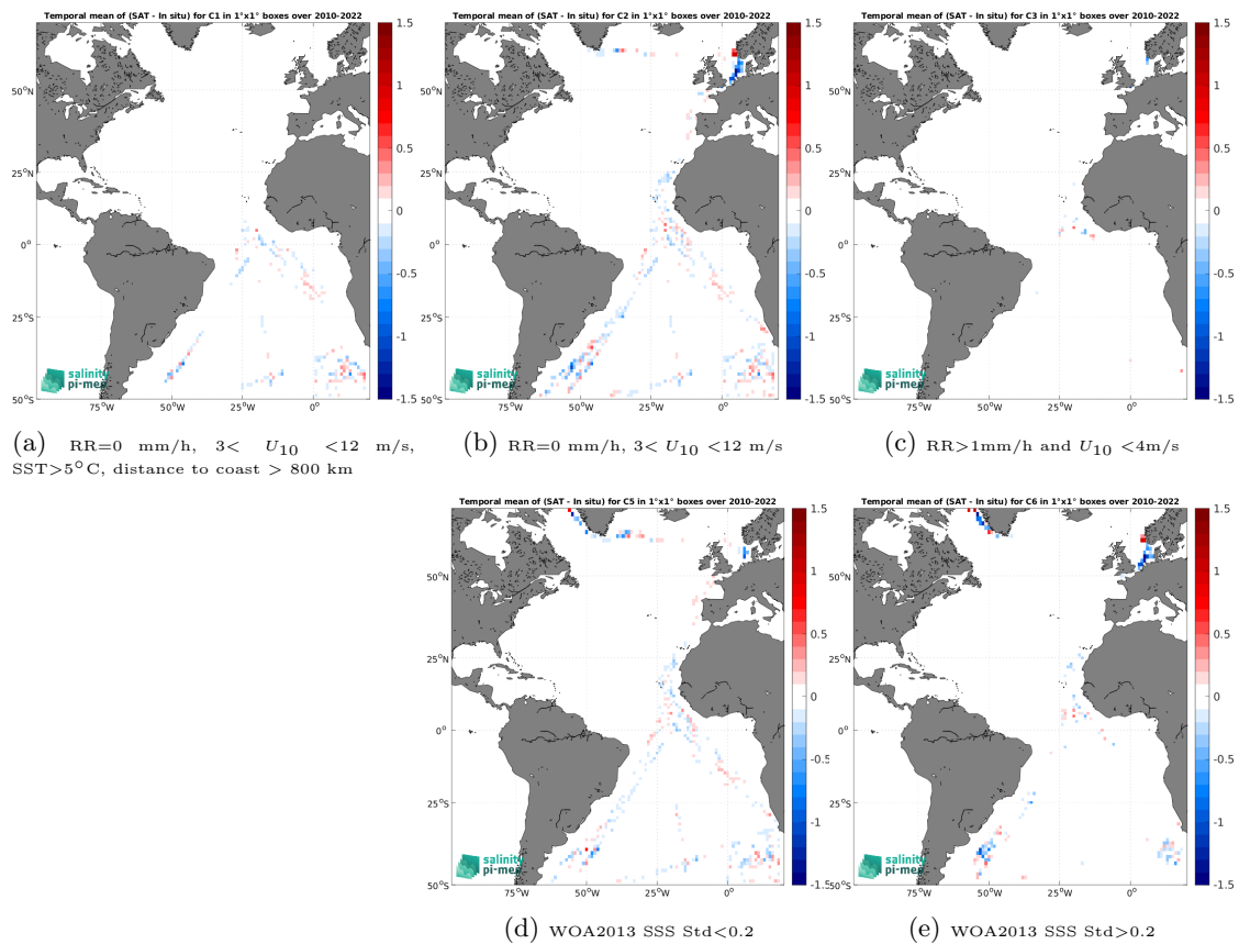
Figure 12: Temporal mean gridded over spatial boxes of size 1^\circ \times 1^\circ of \Delta\text{SSS} (CCI SSS L4 Merged-OI v4.4 - 7-day running (ESA) - TSG (Polarstern)) for 5 different subdatasets corresponding to:RR=0 mm/h, 3 < U_{10} < 12 m/s, SST >5^\circ\text{C} , distance to coast > 800 km (a), RR=0 mm/h, 3 < U_{10} < 12 m/s (b), RR >1 mm/h and U_{10} < 4 m/s (c), WOA2013 SSS Std <0.2 (d), WOA2013 SSS Std >0.2 (e).
