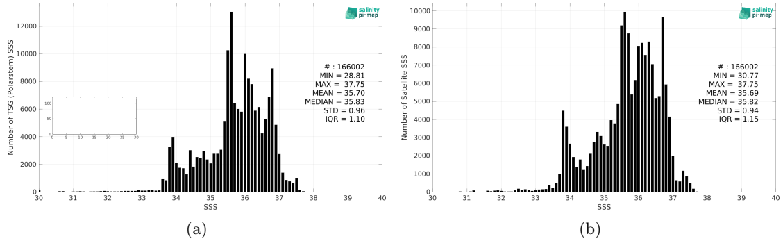
Figure 2: Histograms of SSS from TSG (Polarstern) (a) and CCI SSS L4 Merged-OI v4.4 - 7-day running (ESA) (b) considering all match-up pairs per bins of 0.1 over the Atlantic Ocean Pi-MEP region and for the full satellite product period.
