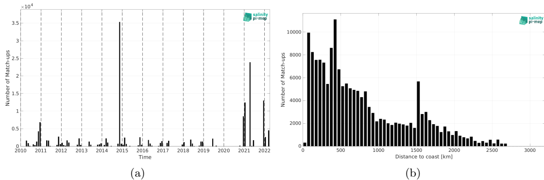
Figure 1: Number of match-ups between TSG (Polarstern) and CCI SSS L4 Merged-OI v4.4 - 7-day running (ESA) SSS as a function of time (a) and as function of the distance to coast (b) over the Atlantic Ocean Pi-MEP region and for the full satellite product period.
