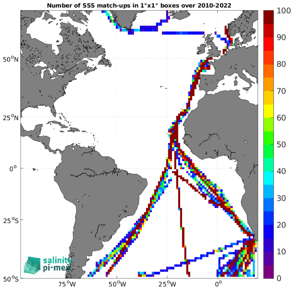
Figure 4: Number of SSS match-ups between TSG (Polarstern) SSS and the CCI SSS L4 Merged-OI v4.4 - 7-day running (ESA) SSS product for the Atlantic Ocean Pi-MEP region over 1°x1° boxes and for the full satellite product period.
