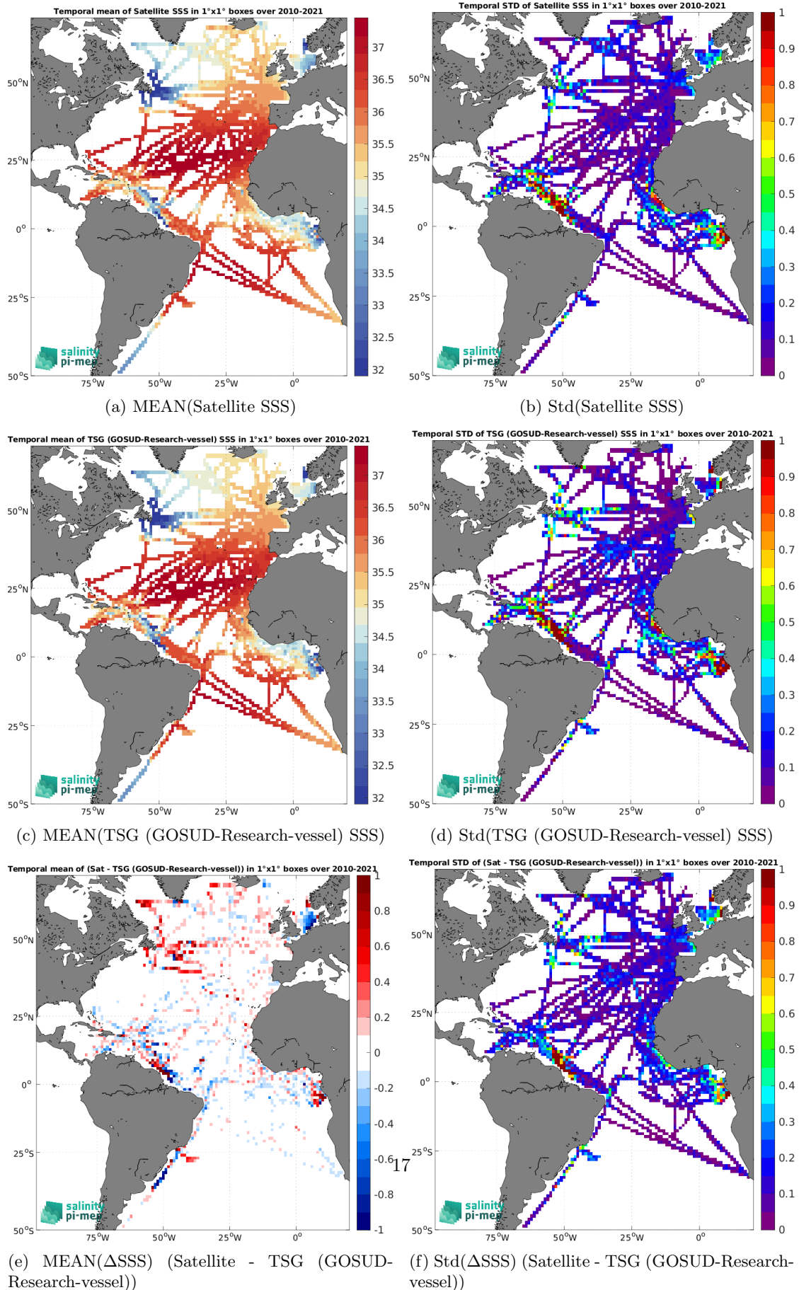
Figure 6: Temporal mean (left) and Std (right) of SSS from CCI SSS L4 Merged-OI v4.4 - 7-day running (ESA) (top), TSG (GOSUD-Research-vessel) (middle), and of \Delta SSS (Satellite - TSG (GOSUD-Research-vessel)). Only match-up pairs are used to generate these maps.
