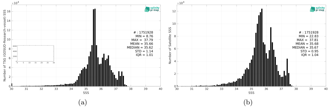
Figure 2: Histograms of SSS from TSG (GOSUD-Research-vessel) (a) and CCI SSS L4 Merged-OI v4.4 - 7-day running (ESA) (b) considering all match-up pairs per bins of 0.1 over the Atlantic Ocean Pi-MEP region and for the full satellite product period.
