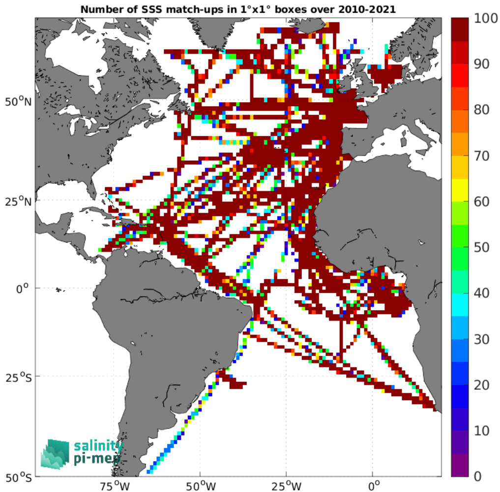
Figure 4: Number of SSS match-ups between TSG (GOSUD-Research-vessel) SSS and the CCI SSS L4 Merged-OI v4.4 - 7-day running (ESA) SSS product for the Atlantic Ocean Pi-MEP region over 1^{\circ} \times 1^{\circ} boxes and for the full satellite product period.
