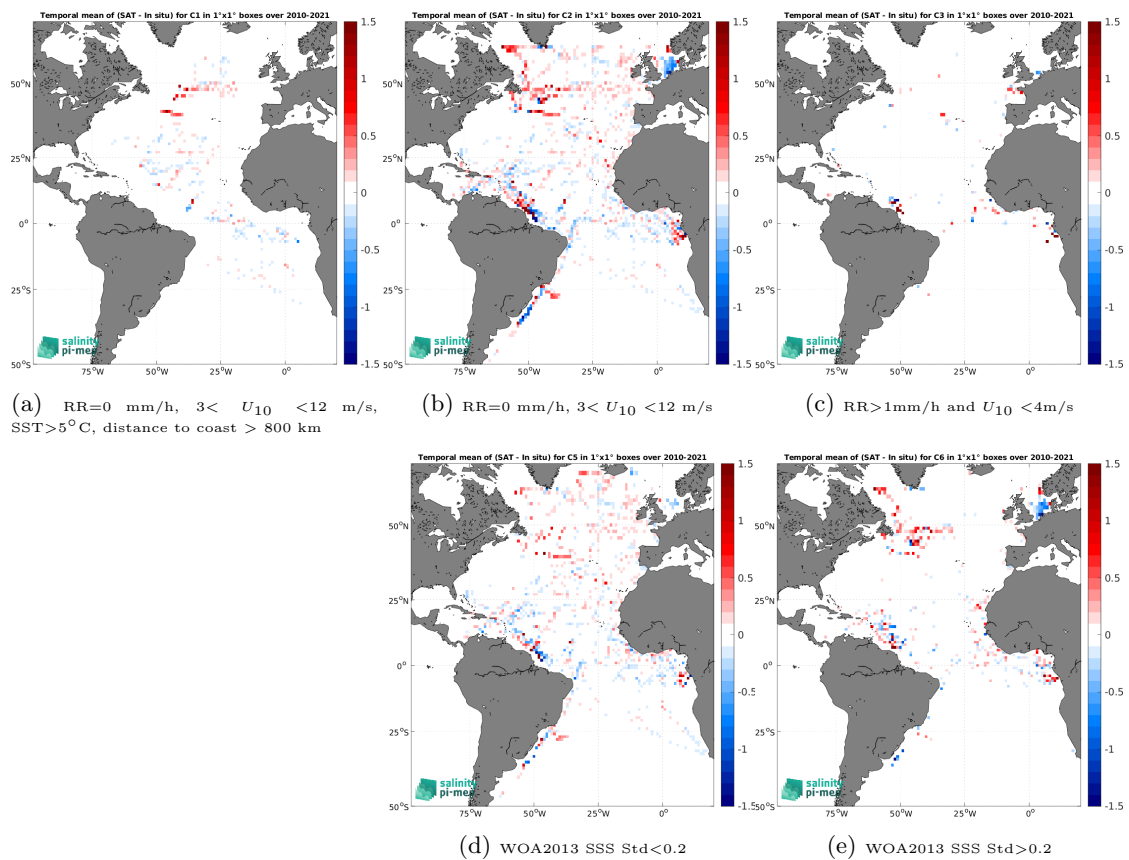
Figure 12: Temporal mean gridded over spatial boxes of size 1^\circ \times 1^\circ of \Delta\text{SSS} (CCI SSS L4 Merged-OI v4.4 - 7-day running (ESA) - TSG (GOSUD-Research-vessel)) for 5 different subdatasets corresponding to:RR=0 mm/h, 3 < U_{10} < 12 m/s, SST >5^\circ\text{C} , distance to coast > 800 km (a), RR=0 mm/h, 3 < U_{10} < 12 m/s (b), RR >1 mm/h and U_{10} < 4 m/s (c), WOA2013 SSS Std <0.2 (d), WOA2013 SSS Std >0.2 (e).
