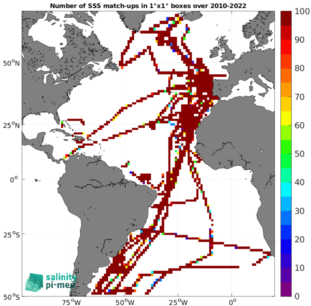
Figure 4: Number of SSS match-ups between TSG (CSIC-UTM) SSS and the CCI SSS L4 Merged-OI v4.4 - 7-day running (ESA) SSS product for the Atlantic Ocean Pi-MEP region over 1^\circ \times 1^\circ boxes and for the full satellite product period.
