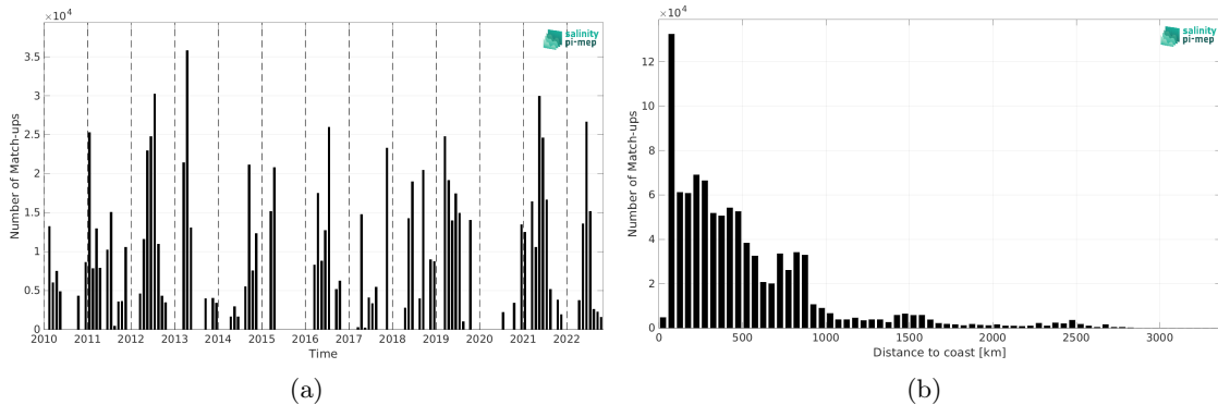
Figure 1: Number of match-ups between TSG (CSIC-UTM) and CCI SSS L4 Merged-OI v4.4 - 7-day running (ESA) SSS as a function of time (a) and as function of the distance to coast (b) over the Atlantic Ocean Pi-MEP region and for the full satellite product period.
