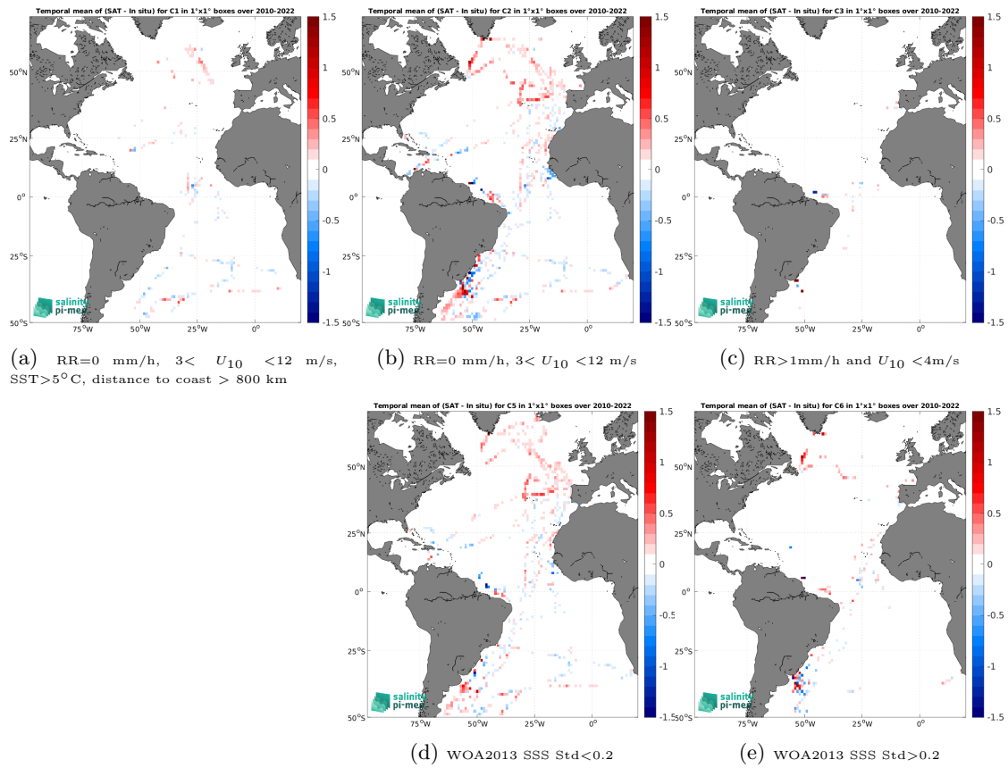
Figure 12: Temporal mean gridded over spatial boxes of size 1^\circ \times 1^\circ of \Delta\text{SSS} (CCI SSS L4 Merged-OI v4.4 - 7-day running (ESA) - TSG (CSIC-UTM)) for 5 different subdatasets corresponding to:RR=0 mm/h, 3 < U_{10} < 12 m/s, SST >5^\circ\text{C} , distance to coast > 800 km (a), RR=0 mm/h, 3 < U_{10} < 12 m/s (b), RR >1 mm/h and U_{10} < 4 m/s (c), WOA2013 SSS Std <0.2 (d), WOA2013 SSS Std >0.2 (e).
