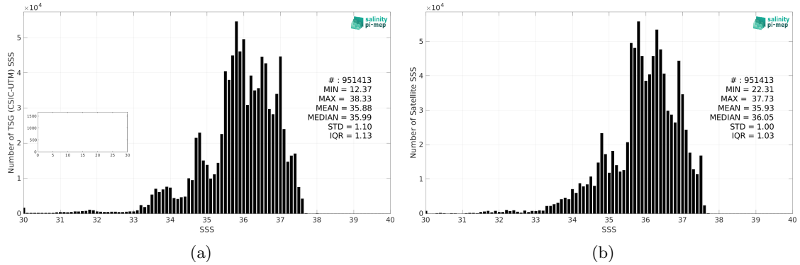
Figure 2: Histograms of SSS from TSG (CSIC-UTM) (a) and CCI SSS L4 Merged-OI v4.4 - 7-day running (ESA) (b) considering all match-up pairs per bins of 0.1 over the Atlantic Ocean Pi-MEP region and for the full satellite product period.
