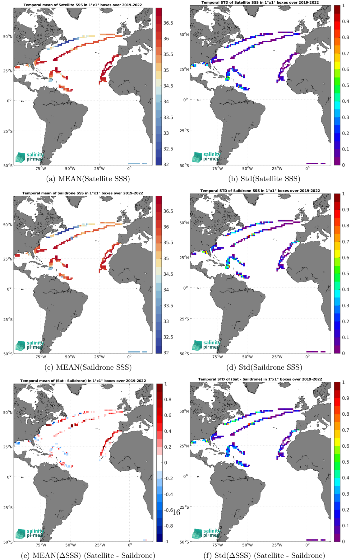
Figure 6: Temporal mean (left) and Std (right) of SSS from CCI SSS L4 Merged-OI v4.4 - 7-day running (ESA) (top), Saildrone (middle), and of \Delta\text{SSS} (Satellite - Saildrone). Only match-up pairs are used to generate these maps.
