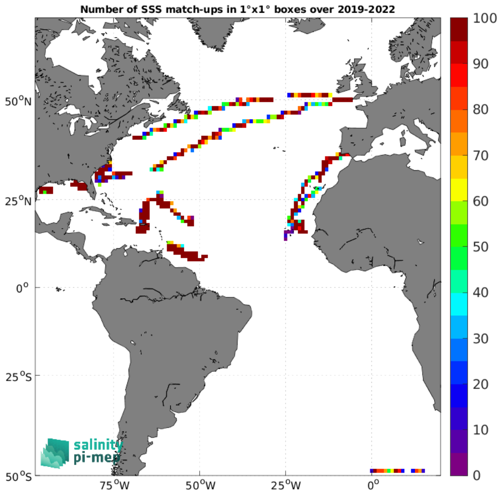
Figure 4: Number of SSS match-ups between Saildrone SSS and the CCI SSS L4 Merged-OI v4.4 - 7-day running (ESA) SSS product for the Atlantic Ocean Pi-MEP region over 1°×1° boxes and for the full satellite product period.
