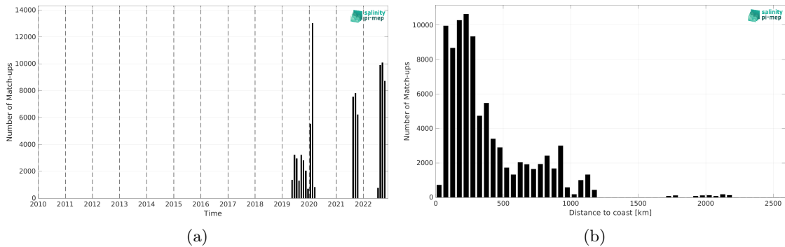
Figure 1: Number of match-ups between Saildrone and CCI SSS L4 Merged-OI v4.4 - 7-day running (ESA) SSS as a function of time (a) and as function of the distance to coast (b) over the Atlantic Ocean Pi-MEP region and for the full satellite product period.
