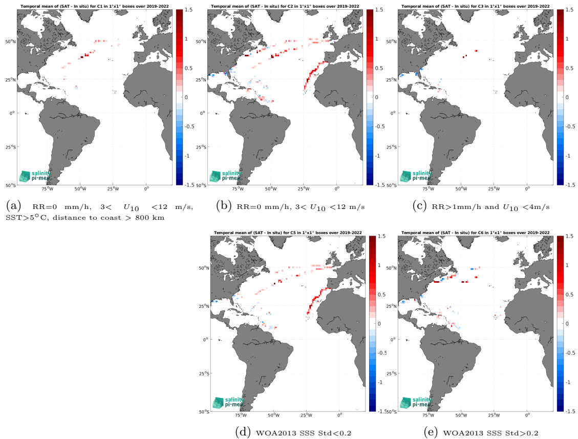
Figure 12: Temporal mean gridded over spatial boxes of size 1^\circ \times 1^\circ of \Delta\text{SSS} (CCI SSS L4 Merged-OI v4.4 - 7-day running (ESA) - Sailability) for 5 different subdatasets corresponding to:RR=0 mm/h, 3 < U_{10} < 12 m/s, SST >5^\circ\text{C} , distance to coast > 800 km (a), RR=0 mm/h, 3 < U_{10} < 12 m/s (b), RR >1 mm/h and U_{10} < 4 m/s (c), WOA2013 SSS Std <0.2 (d), WOA2013 SSS Std >0.2 (e).
