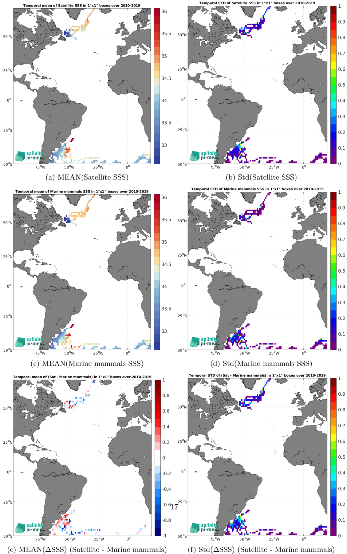
Figure 6: Temporal mean (left) and Std (right) of SSS from CCI SSS L4 Merged-OI v4.4 - 7-day running (ESA) (top), Marine mammals (middle), and of \Delta SSS (Satellite - Marine mammals). Only match-up pairs are used to generate these maps.
