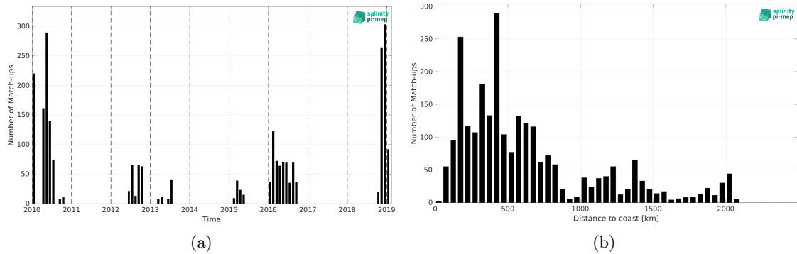
Figure 1: Number of match-ups between Marine mammals and CCI SSS L4 Merged-OI v4.4 - 7-day running (ESA) SSS as a function of time (a) and as function of the distance to coast (b) over the Atlantic Ocean Pi-MEP region and for the full satellite product period.
