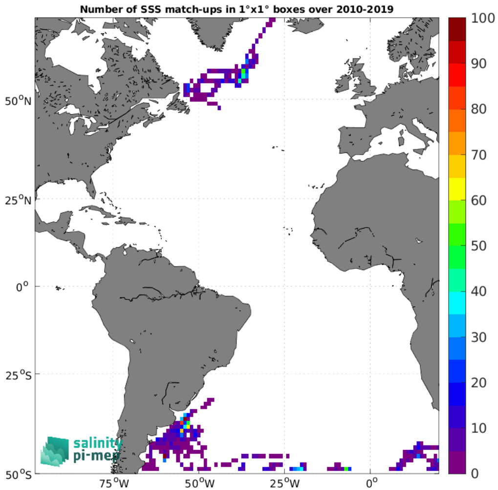
Figure 4: Number of SSS match-ups between Marine mammals SSS and the CCI SSS L4 Merged-OI v4.4 - 7-day running (ESA) SSS product for the Atlantic Ocean Pi-MEP region over 1°x1° boxes and for the full satellite product period.
