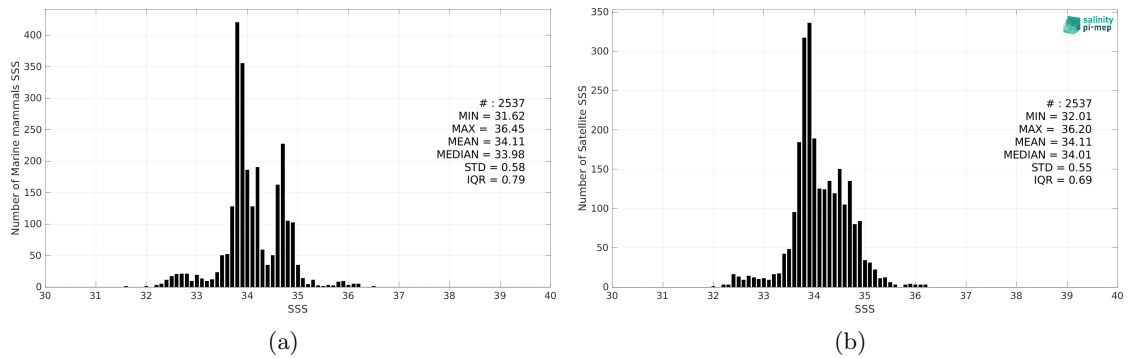
Figure 2: Histograms of SSS from Marine mammals (a) and CCI SSS L4 Merged-OI v4.4 - 7-day running (ESA) (b) considering all match-up pairs per bins of 0.1 over the Atlantic Ocean Pi-MEP region and for the full satellite product period.
