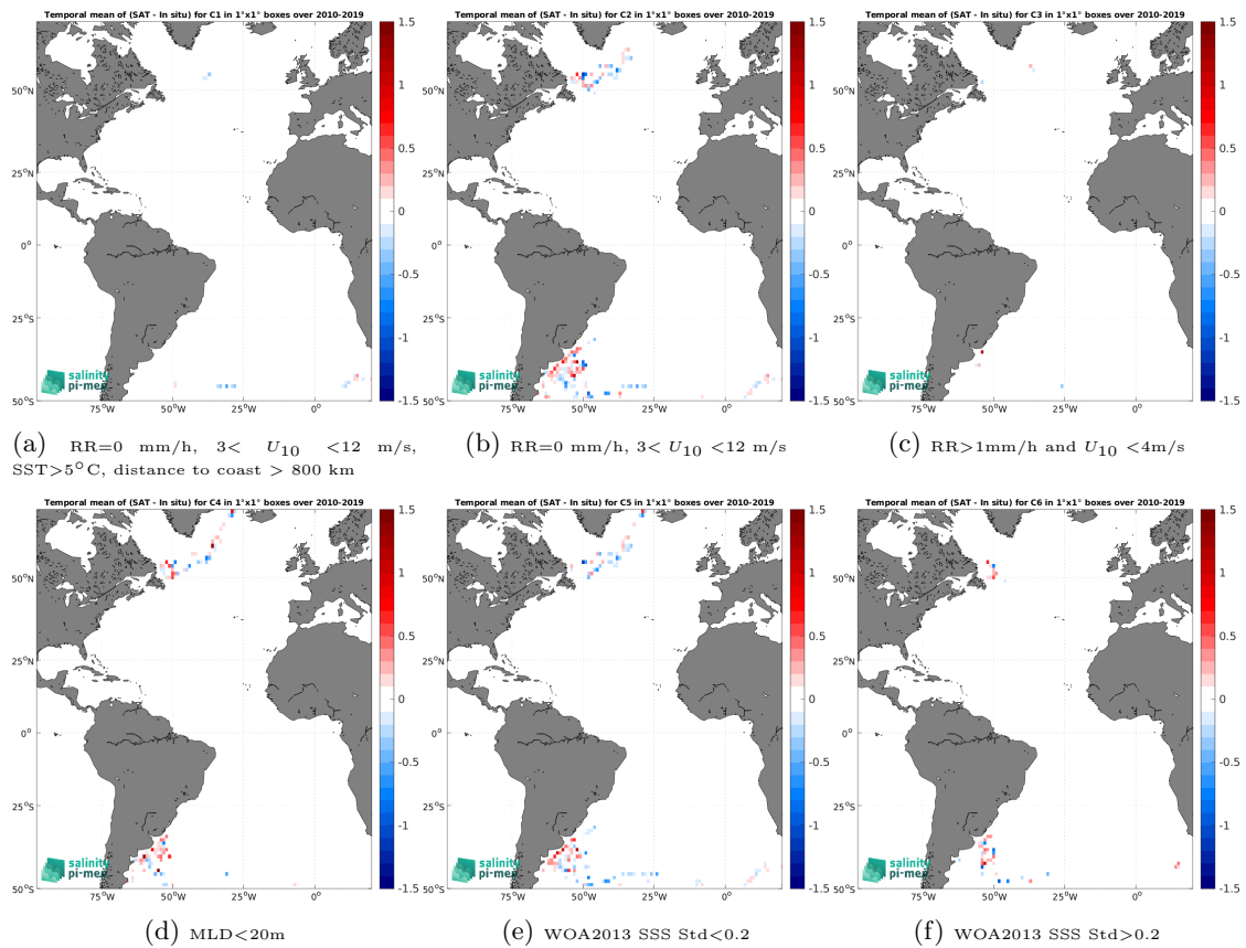
Figure 12: Temporal mean gridded over spatial boxes of size 1^\circ \times 1^\circ of \Delta SSS (CCI SSS L4 Merged-OI v4.4 - 7-day running (ESA) - Marine mammals) for 6 different subdatasets corresponding to:RR=0 mm/h, 3 < U_{10} < 12 m/s, SST > 5^\circ\text{C} , distance to coast > 800 km (a), RR=0 mm/h, 3 < U_{10} < 12 m/s (b), RR > 1 mm/h and U_{10} < 4 m/s (c),MLD < 20 m (d),WOA2013 SSS Std < 0.2 (e),WOA2013 SSS Std > 0.2 (f).
