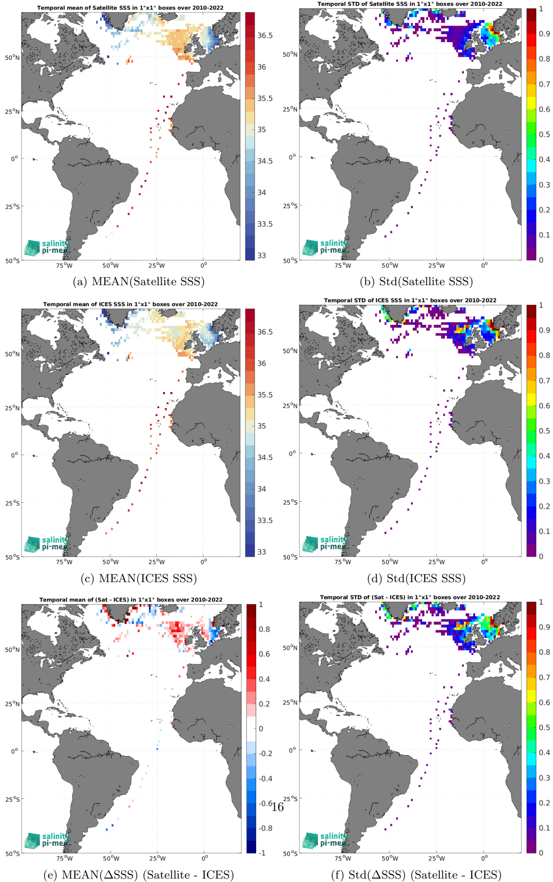
Figure 6: Temporal mean (left) and Std (right) of SSS from CCI SSS L4 Merged-OI v4.4 - 7-day running (ESA) (top), ICES (middle), and of \Delta\text{SSS} (Satellite - ICES). Only match-up pairs are used to generate these maps.
