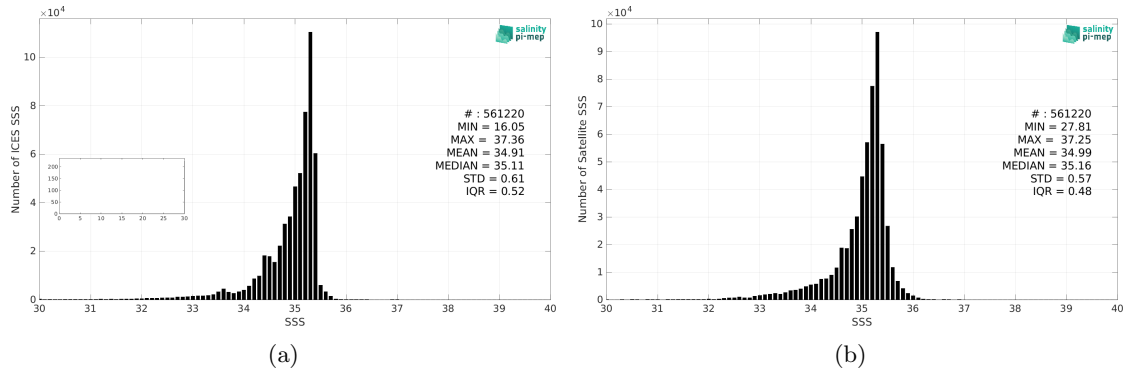
Figure 2: Histograms of SSS from ICES (a) and CCI SSS L4 Merged-OI v4.4 - 7-day running (ESA) (b) considering all match-up pairs per bins of 0.1 over the Atlantic Ocean Pi-MEP region and for the full satellite product period.
