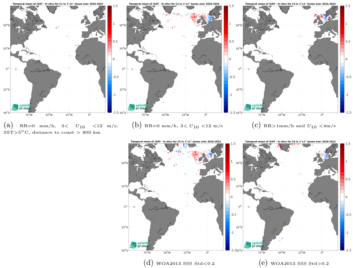
Figure 12: Temporal mean gridded over spatial boxes of size 1^\circ \times 1^\circ of \Delta\text{SSS} (CCI SSS L4 Merged-OI v4.4 - 7-day running (ESA) - ICES) for 5 different subdatasets corresponding to:RR=0 mm/h, 3 < U_{10} < 12 m/s, SST >5^\circ\text{C} , distance to coast > 800 km (a), RR=0 mm/h, 3 < U_{10} < 12 m/s (b), RR >1 mm/h and U_{10} < 4 m/s (c), WOA2013 SSS Std <0.2 (d), WOA2013 SSS Std >0.2 (e).
