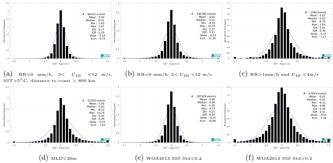
Figure 13: Normalized histogram of \Delta\text{SSS} (CCI SSS L4 Merged-OI v4.4 - 7-day running (ESA) - Argo) for 6 different subdatasets corresponding to: RR=0 mm/h, 3 < U_{10} < 12 m/s, SST>5°C, distance to coast > 800 km (a), RR=0 mm/h, 3 < U_{10} < 12 m/s (b), RR>1mm/h and U_{10} < 4 m/s (c), MLD<20m (d), WOA2013 SSS Std<0.2 (e), WOA2013 SSS Std>0.2 (f).
