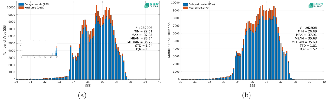
Figure 2: Histograms of SSS from Argo (a) and CCI SSS L4 Merged-OI v4.4 - 7-day running (ESA) (b) considering all match-up pairs per bins of 0.1 over the Atlantic Ocean Pi-MEP region and for the full satellite product period.
