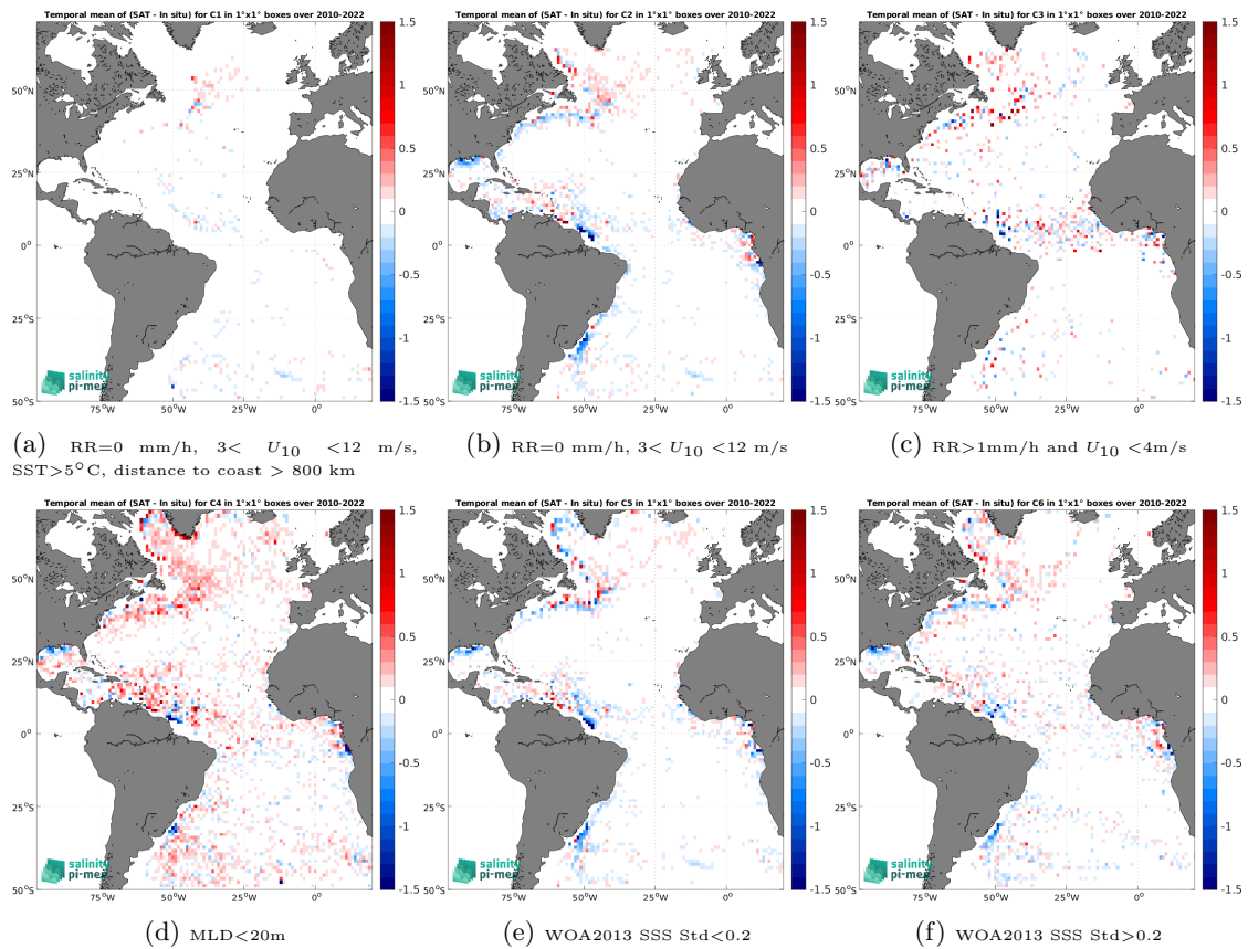
Figure 12: Temporal mean gridded over spatial boxes of size 1^\circ \times 1^\circ of \Delta SSS (CCI SSS L4 Merged-OI v4.4 - 7-day running (ESA) - Argo) for 6 different subdatasets corresponding to:RR=0 mm/h, 3 < U_{10} < 12 m/s, SST > 5^\circ\text{C} , distance to coast > 800 km (a), RR=0 mm/h, 3 < U_{10} < 12 m/s (b), RR > 1 mm/h and U_{10} < 4 m/s (c),MLD < 20 m (d),WOA2013 SSS Std < 0.2 (e),WOA2013 SSS Std > 0.2 (f).
