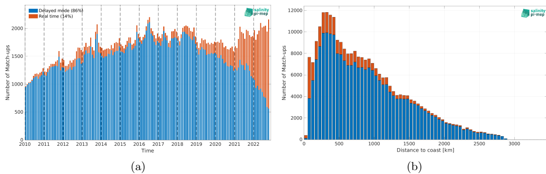
Figure 1: Number of match-ups between Argo and CCI SSS L4 Merged-OI v4.4 - 7-day running (ESA) SSS as a function of time (a) and as function of the distance to coast (b) over the Atlantic Ocean Pi-MEP region and for the full satellite product period.
