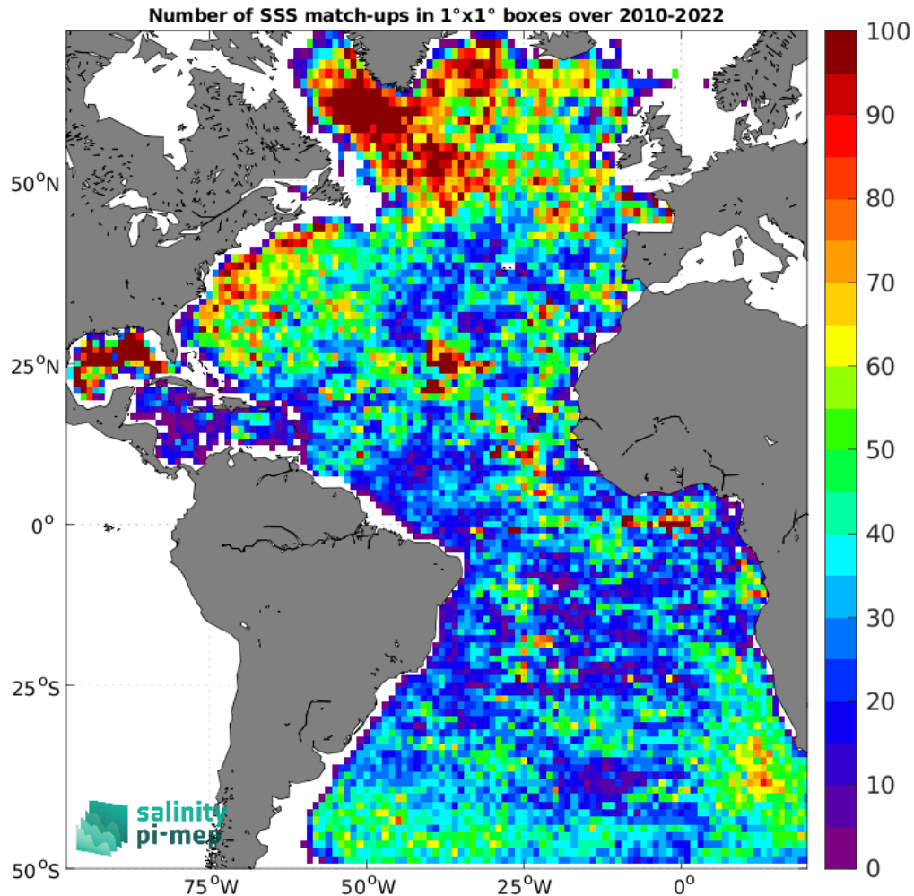
Figure 4: Number of SSS match-ups between Argo SSS and the CCI SSS L4 Merged-OI v4.4 - 7-day running (ESA) SSS product for the Atlantic Ocean Pi-MEP region over 1^\circ \times 1^\circ boxes and for the full satellite product period.
