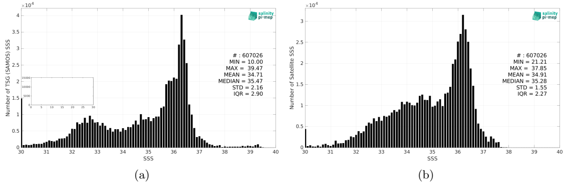
Figure 2: Histograms of SSS from TSG (SAMOS) (a) and CCI SSS L4 Merged-OI v4.4 - 30-day running (ESA) (b) considering all match-up pairs per bins of 0.1 over the Atlantic Ocean Pi-MEP region and for the full satellite product period.
