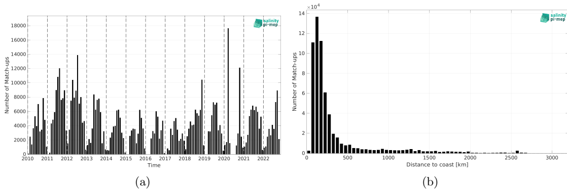
Figure 1: Number of match-ups between TSG (SAMOS) and CCI SSS L4 Merged-OI v4.4 - 30-day running (ESA) SSS as a function of time (a) and as function of the distance to coast (b) over the Atlantic Ocean Pi-MEP region and for the full satellite product period.
