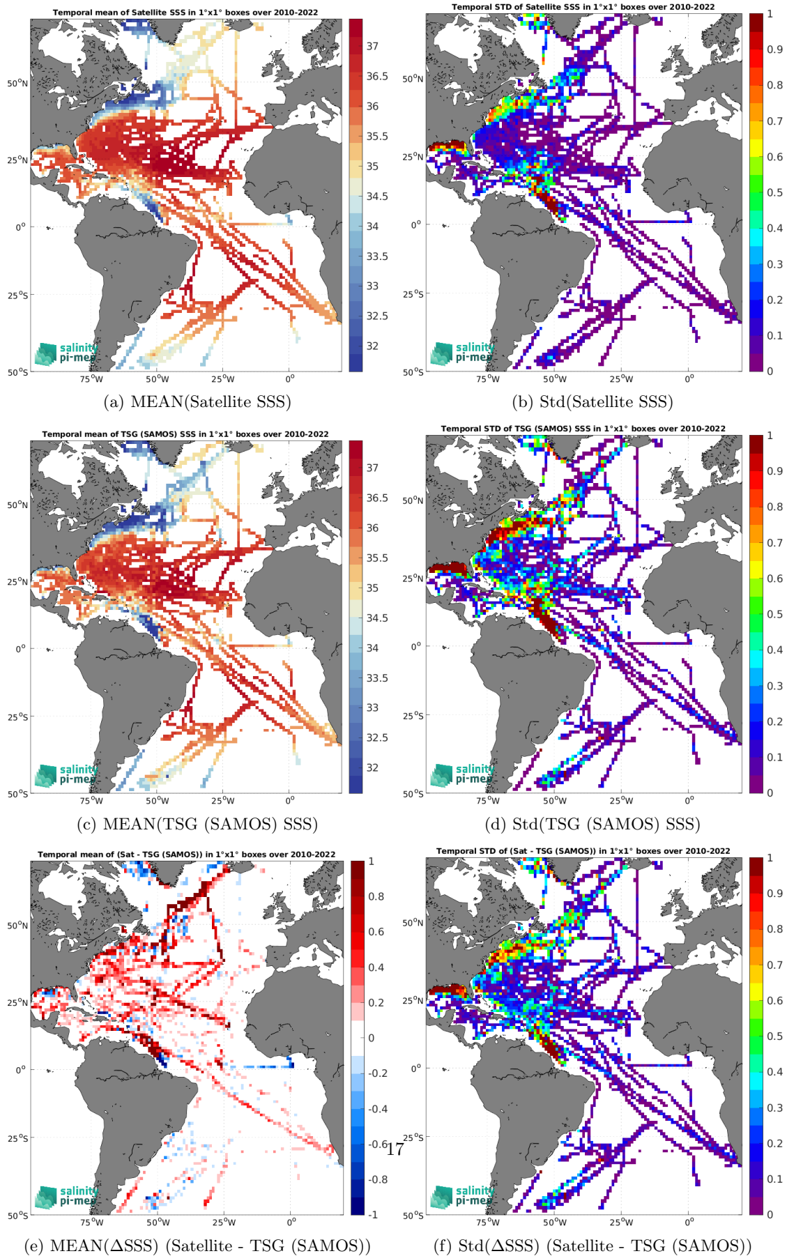
Figure 6: Temporal mean (left) and Std (right) of SSS from CCI SSS L4 Merged-OI v4.4 - 30-day running (ESA) (top), TSG (SAMOS) (middle), and of \Delta SSS (Satellite - TSG (SAMOS)). Only match-up pairs are used to generate these maps.
