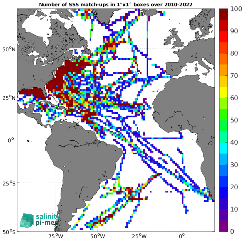
Figure 4: Number of SSS match-ups between TSG (SAMOS) SSS and the CCI SSS L4 Merged-OI v4.4 - 30-day running (ESA) SSS product for the Atlantic Ocean Pi-MEP region over 1^\circ \times 1^\circ boxes and for the full satellite product period.
