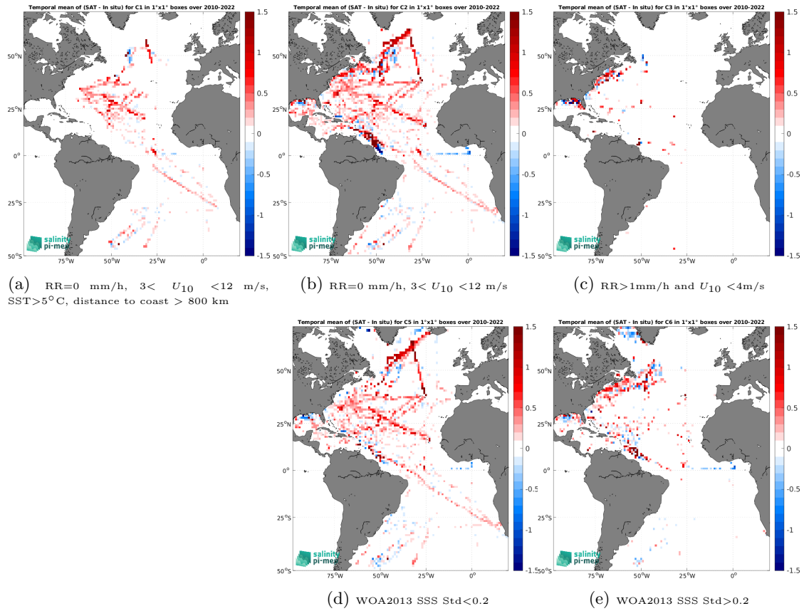
Figure 12: Temporal mean gridded over spatial boxes of size 1^\circ \times 1^\circ of \Delta\text{SSS} (CCI SSS L4 Merged-OI v4.4 - 30-day running (ESA) - TSG (SAMOS)) for 5 different subdatasets corresponding to:RR=0 mm/h, 3 < U_{10} < 12 m/s, SST >5^\circ\text{C} , distance to coast > 800 km (a), RR=0 mm/h, 3 < U_{10} < 12 m/s (b), RR >1 mm/h and U_{10} < 4 m/s (c), WOA2013 SSS Std <0.2 (d), WOA2013 SSS Std >0.2 (e).
