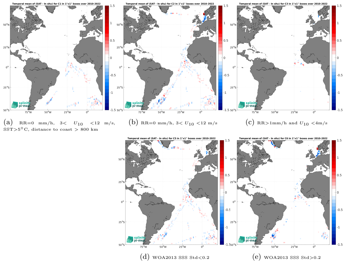
Figure 12: Temporal mean gridded over spatial boxes of size 1^\circ \times 1^\circ of \Delta\text{SSS} (CCI SSS L4 Merged-OI v4.4 - 30-day running (ESA) - TSG (Polarstern)) for 5 different subdatasets corresponding to:RR=0 mm/h, 3 < U_{10} < 12 m/s, SST >5^\circ\text{C} , distance to coast > 800 km (a), RR=0 mm/h, 3 < U_{10} < 12 m/s (b), RR >1 mm/h and U_{10} < 4 m/s (c), WOA2013 SSS Std <0.2 (d), WOA2013 SSS Std >0.2 (e).
