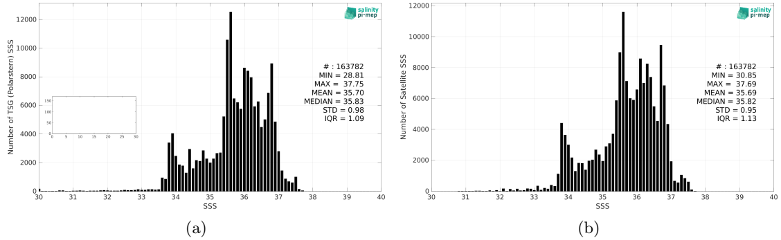
Figure 2: Histograms of SSS from TSG (Polarstern) (a) and CCI SSS L4 Merged-OI v4.4 - 30-day running (ESA) (b) considering all match-up pairs per bins of 0.1 over the Atlantic Ocean Pi-MEP region and for the full satellite product period.
