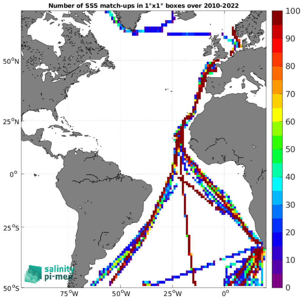
Figure 4: Number of SSS match-ups between TSG (Polarstern) SSS and the CCI SSS L4 Merged-OI v4.4 - 30-day running (ESA) SSS product for the Atlantic Ocean Pi-MEP region over 1°x1° boxes and for the full satellite product period.
