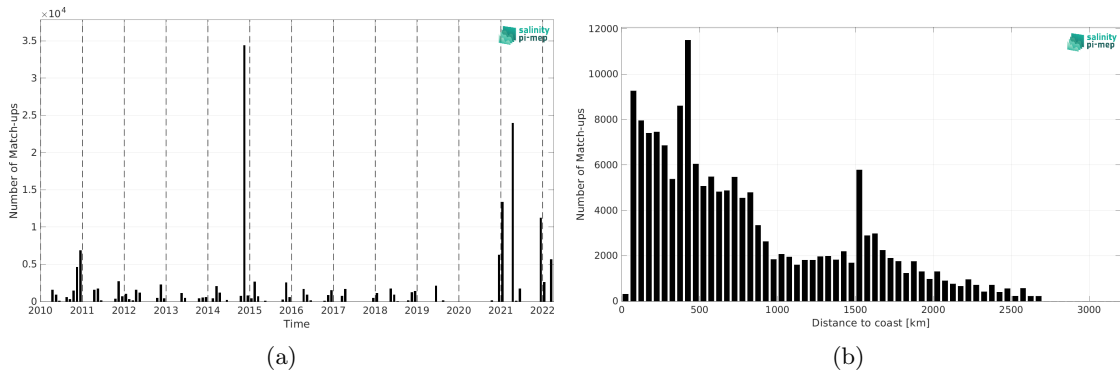
Figure 1: Number of match-ups between TSG (Polarstern) and CCI SSS L4 Merged-OI v4.4 - 30-day running (ESA) SSS as a function of time (a) and as function of the distance to coast (b) over the Atlantic Ocean Pi-MEP region and for the full satellite product period.
