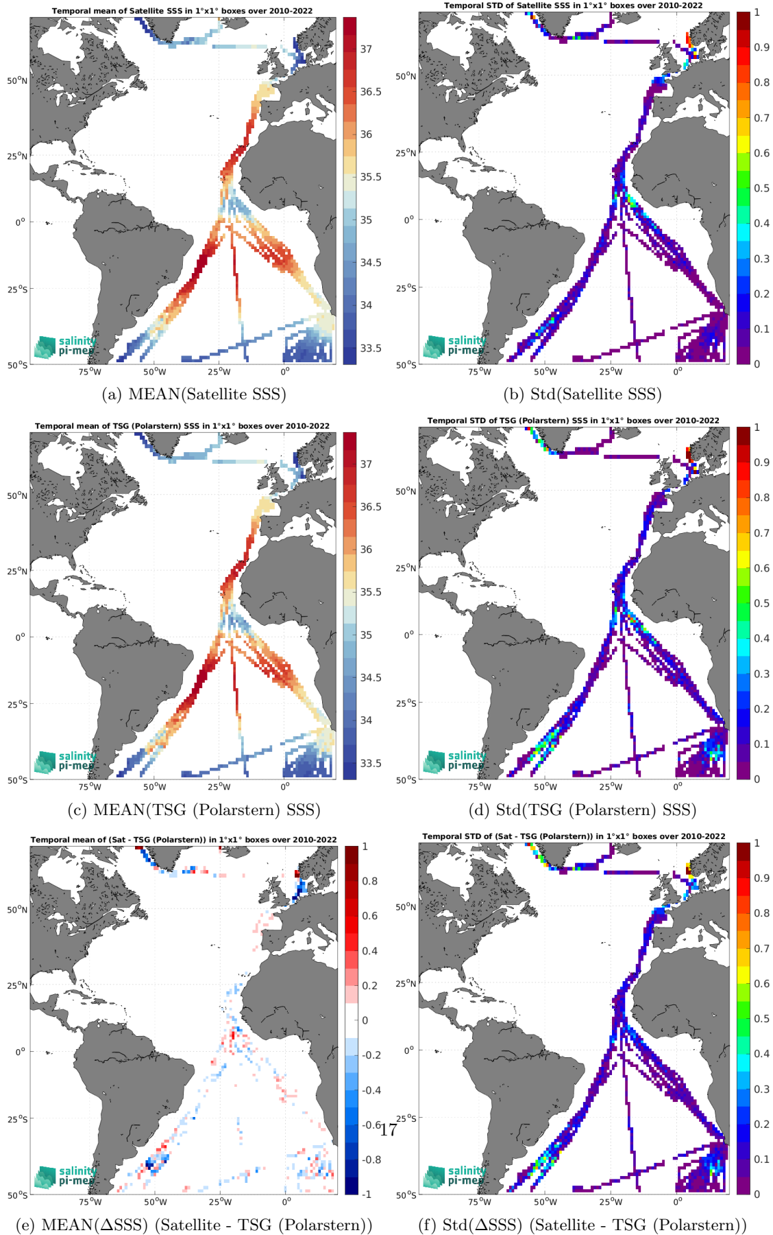
Figure 6: Temporal mean (left) and Std (right) of SSS from CCI SSS L4 Merged-OI v4.4 - 30-day running (ESA) (top), TSG (Polarstern) (middle), and of \Delta SSS (Satellite - TSG (Polarstern)). Only match-up pairs are used to generate these maps.
