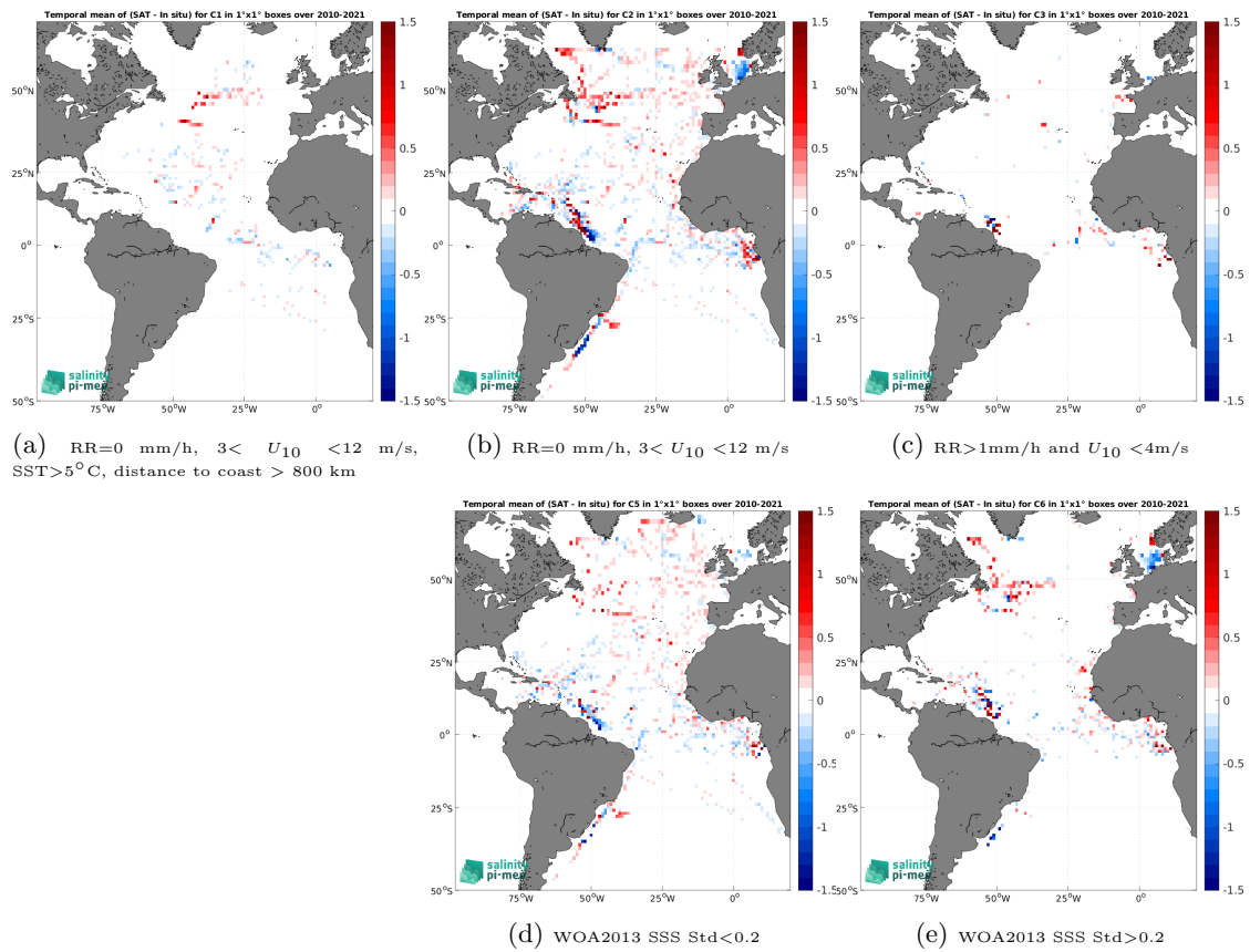
Figure 12: Temporal mean gridded over spatial boxes of size 1^\circ \times 1^\circ of \Delta\text{SSS} (CCI SSS L4 Merged-OI v4.4 - 30-day running (ESA) - TSG (GOSUD-Research-vessel)) for 5 different subdatasets corresponding to:RR=0 mm/h, 3 < U_{10} < 12 m/s, SST>5°C, distance to coast > 800 km (a), RR=0 mm/h, 3 < U_{10} < 12 m/s (b), RR>1mm/h and U_{10} < 4 m/s (c), WOA2013 SSS Std<0.2 (d), WOA2013 SSS Std>0.2 (e).
