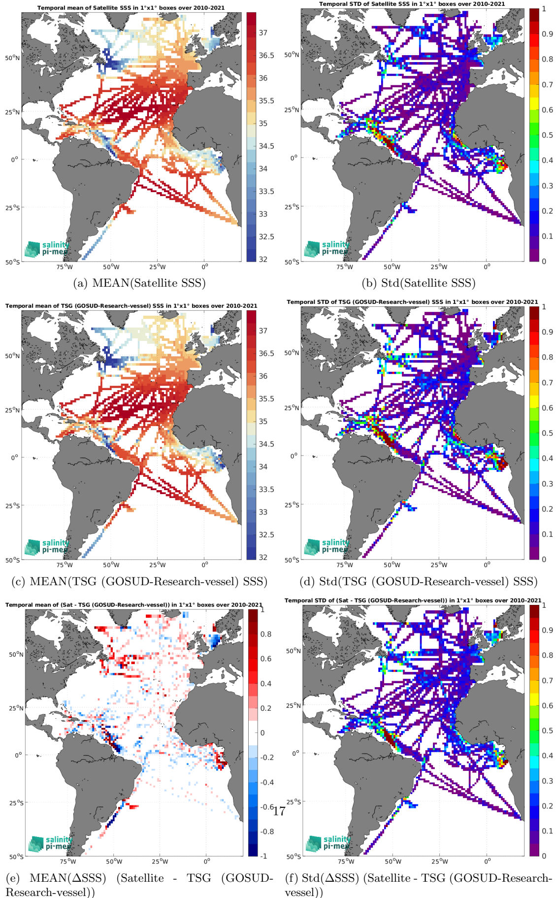
Figure 6: Temporal mean (left) and Std (right) of SSS from CCI SSS L4 Merged-OI v4.4 - 30-day running (ESA) (top), TSG (GOSUD-Research-vessel) (middle), and of \Delta SSS (Satellite - TSG (GOSUD-Research-vessel)). Only match-up pairs are used to generate these maps.
