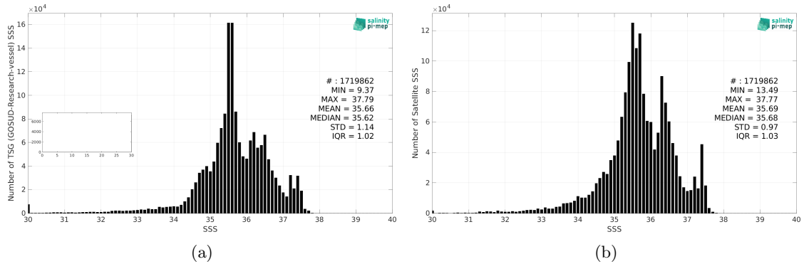
Figure 2: Histograms of SSS from TSG (GOSUD-Research-vessel) (a) and CCI SSS L4 Merged-OI v4.4 - 30-day running (ESA) (b) considering all match-up pairs per bins of 0.1 over the Atlantic Ocean Pi-MEP region and for the full satellite product period.
