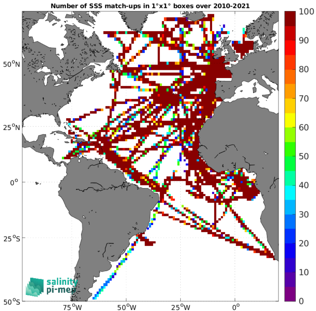
Figure 4: Number of SSS match-ups between TSG (GOSUD-Research-vessel) SSS and the CCI SSS L4 Merged-OI v4.4 - 30-day running (ESA) SSS product for the Atlantic Ocean Pi-MEP region over 1°×1° boxes and for the full satellite product period.
