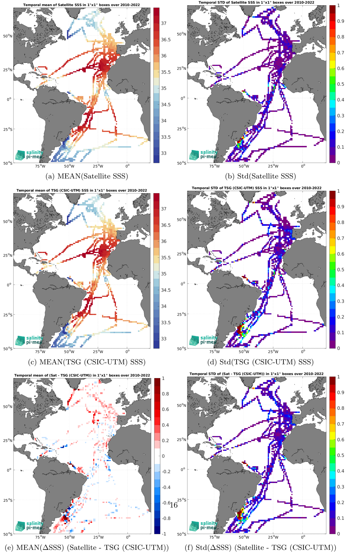
Figure 6: Temporal mean (left) and Std (right) of SSS from CCI SSS L4 Merged-OI v4.4 - 30-day running (ESA) (top), TSG (CSIC-UTM) (middle), and of \Delta SSS (Satellite - TSG (CSIC-UTM)). Only match-up pairs are used to generate these maps.
