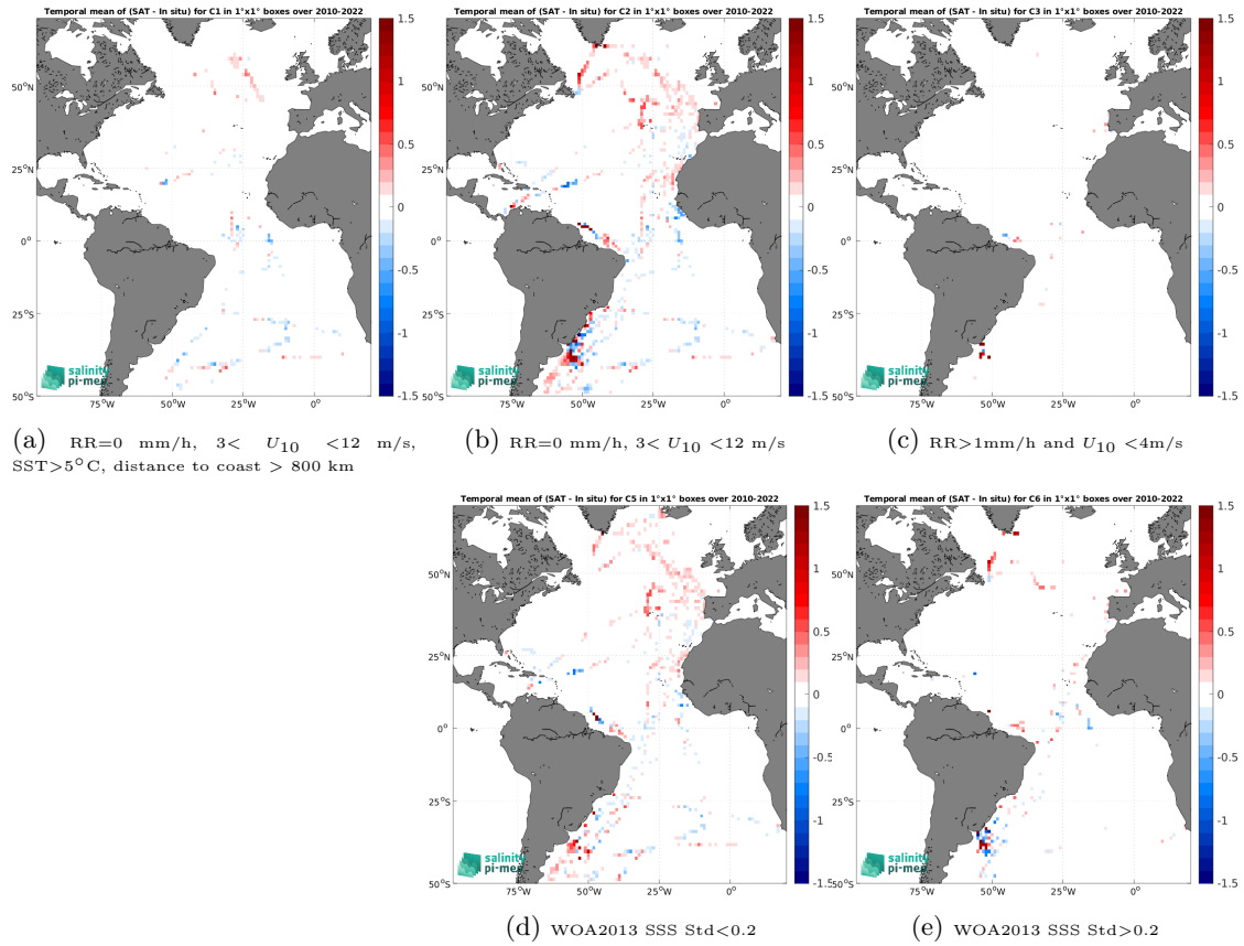
Figure 12: Temporal mean gridded over spatial boxes of size 1^\circ \times 1^\circ of \Delta SSS (CCI SSS L4 Merged-OI v4.4 - 30-day running (ESA) - TSG (CSIC-UTM)) for 5 different subdatasets corresponding to:RR=0 mm/h, 3 < U_{10} < 12 m/s, SST >5^\circ\text{C} , distance to coast > 800 km (a), RR=0 mm/h, 3 < U_{10} < 12 m/s (b), RR >1 mm/h and U_{10} < 4 m/s (c), WOA2013 SSS Std <0.2 (d), WOA2013 SSS Std >0.2 (e).
