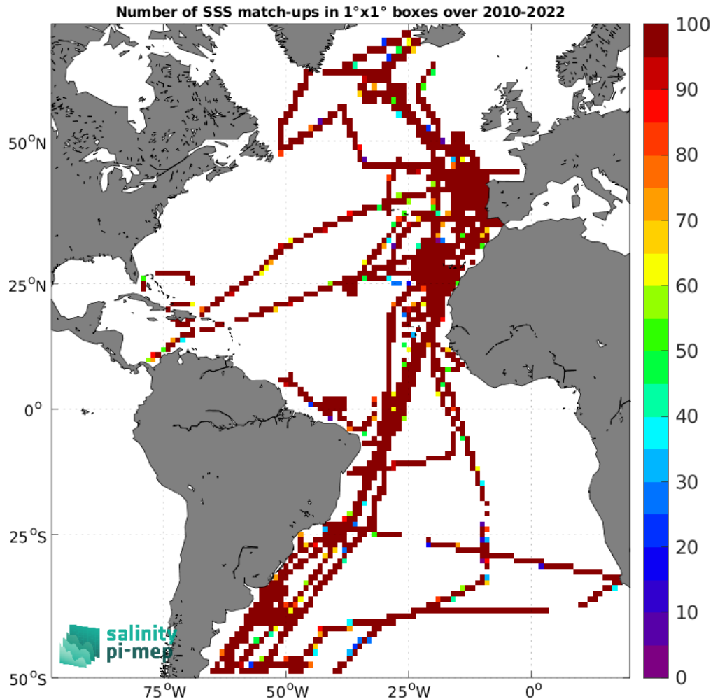
Figure 4: Number of SSS match-ups between TSG (CSIC-UTM) SSS and the CCI SSS L4 Merged-OI v4.4 - 30-day running (ESA) SSS product for the Atlantic Ocean Pi-MEP region over 1^\circ \times 1^\circ boxes and for the full satellite product period.
