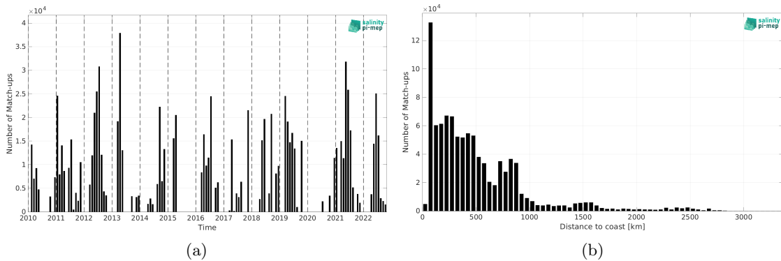
Figure 1: Number of match-ups between TSG (CSIC-UTM) and CCI SSS L4 Merged-OI v4.4 - 30-day running (ESA) SSS as a function of time (a) and as function of the distance to coast (b) over the Atlantic Ocean Pi-MEP region and for the full satellite product period.
