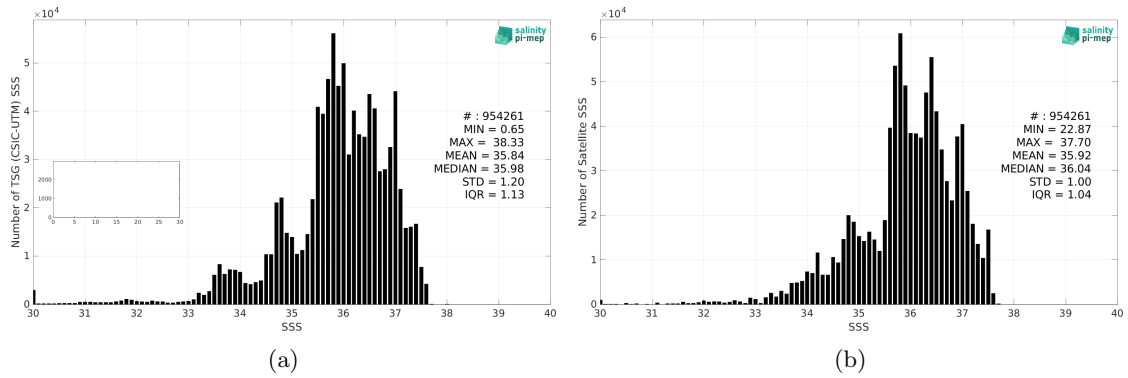
Figure 2: Histograms of SSS from TSG (CSIC-UTM) (a) and CCI SSS L4 Merged-OI v4.4 - 30-day running (ESA) (b) considering all match-up pairs per bins of 0.1 over the Atlantic Ocean Pi-MEP region and for the full satellite product period.
