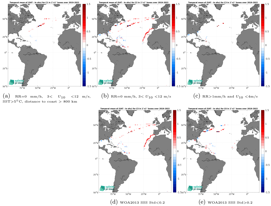
Figure 12: Temporal mean gridded over spatial boxes of size 1^\circ \times 1^\circ of \Delta\text{SSS} (CCI SSS L4 Merged-OI v4.4 - 30-day running (ESA) - Saildrone) for 5 different subdatasets corresponding to:RR=0 mm/h, 3 < U_{10} < 12 m/s, SST >5^\circ\text{C} , distance to coast > 800 km (a), RR=0 mm/h, 3 < U_{10} < 12 m/s (b), RR >1 mm/h and U_{10} < 4 m/s (c), WOA2013 SSS Std <0.2 (d), WOA2013 SSS Std >0.2 (e).
