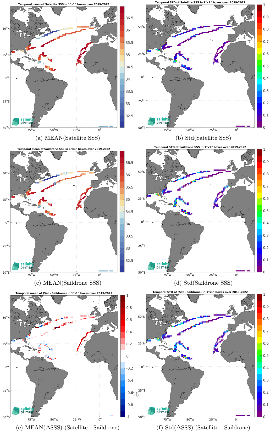
Figure 6: Temporal mean (left) and Std (right) of SSS from CCI SSS L4 Merged-OI v4.4 - 30-day running (ESA) (top), Saildrone (middle), and of \Delta SSS (Satellite - Saildrone). Only match-up pairs are used to generate these maps.
