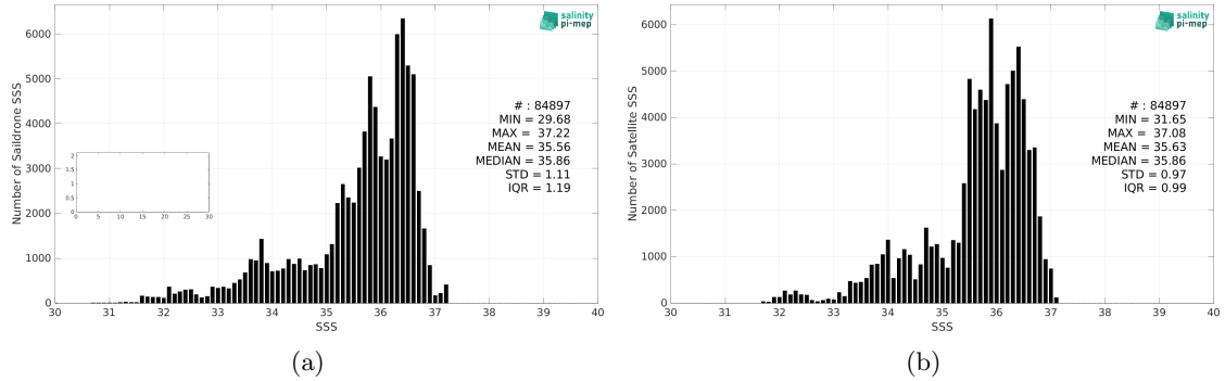
Figure 2: Histograms of SSS from Saildrone (a) and CCI SSS L4 Merged-OI v4.4 - 30-day running (ESA) (b) considering all match-up pairs per bins of 0.1 over the Atlantic Ocean Pi-MEP region and for the full satellite product period.
