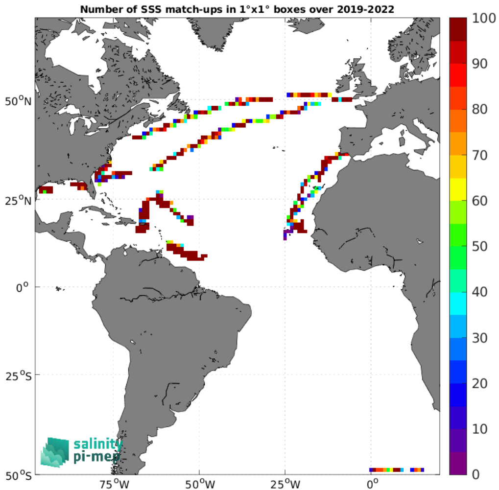
Figure 4: Number of SSS match-ups between Saildrone SSS and the CCI SSS L4 Merged-OI v4.4 - 30-day running (ESA) SSS product for the Atlantic Ocean Pi-MEP region over 1^\circ \times 1^\circ boxes and for the full satellite product period.
