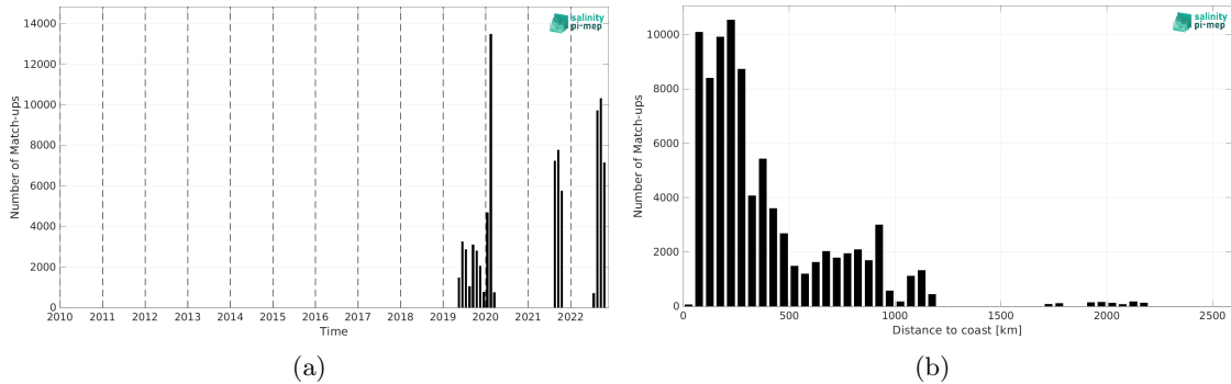
Figure 1: Number of match-ups between Saildrone and CCI SSS L4 Merged-OI v4.4 - 30-day running (ESA) SSS as a function of time (a) and as function of the distance to coast (b) over the Atlantic Ocean Pi-MEP region and for the full satellite product period.
