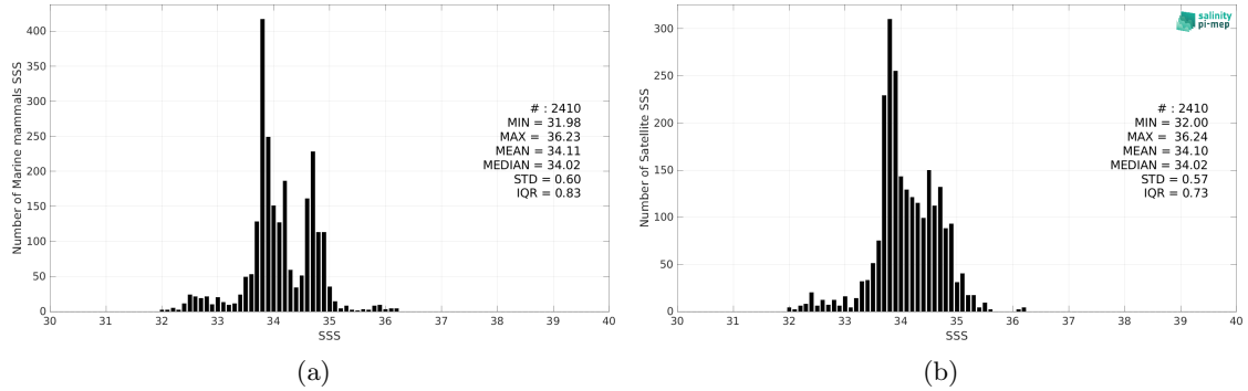
Figure 2: Histograms of SSS from Marine mammals (a) and CCI SSS L4 Merged-OI v4.4 - 30-day running (ESA) (b) considering all match-up pairs per bins of 0.1 over the Atlantic Ocean Pi-MEP region and for the full satellite product period.
