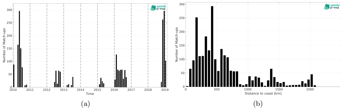
Figure 1: Number of match-ups between Marine mammals and CCI SSS L4 Merged-OI v4.4 - 30-day running (ESA) SSS as a function of time (a) and as function of the distance to coast (b) over the Atlantic Ocean Pi-MEP region and for the full satellite product period.
