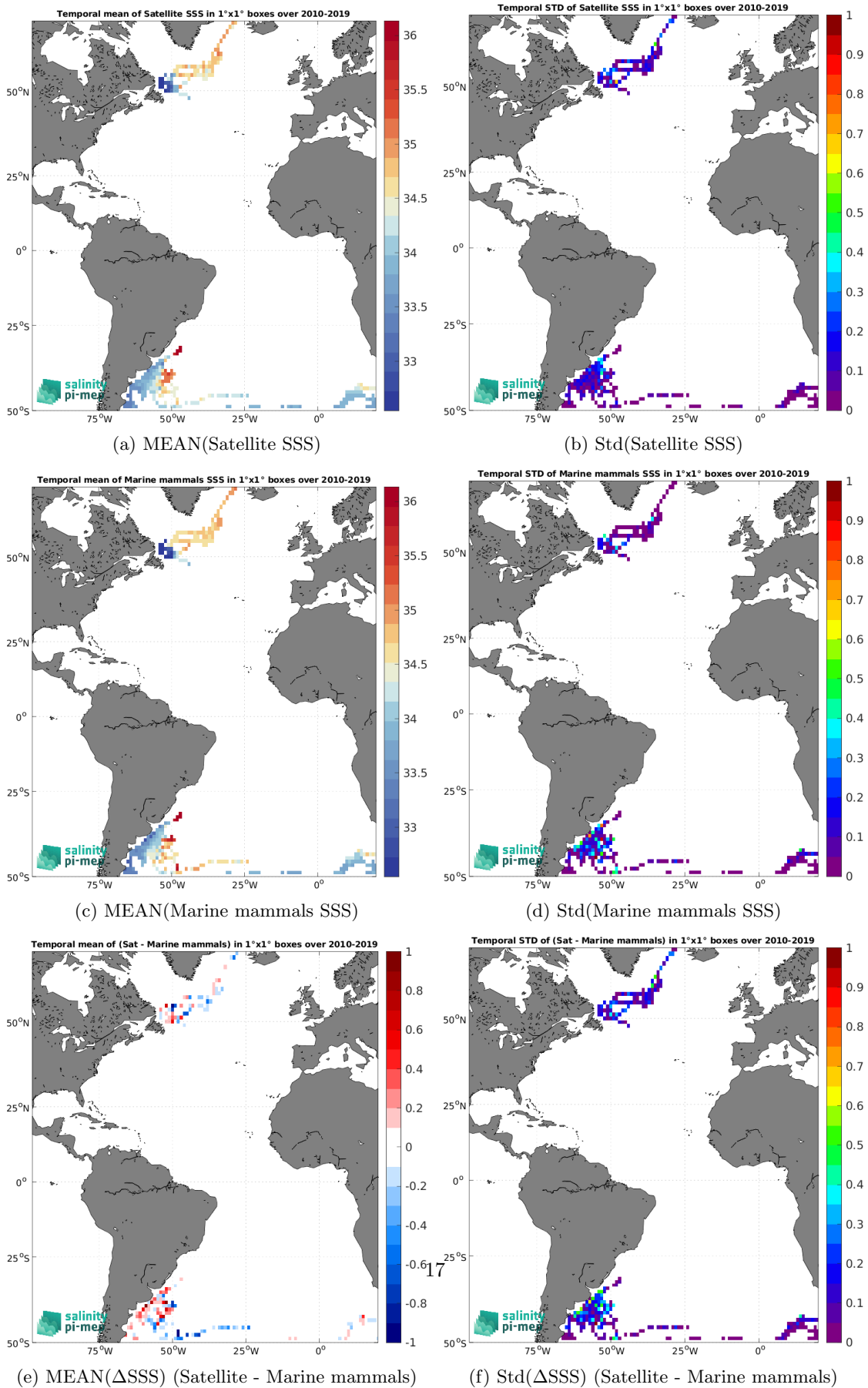
Figure 6: Temporal mean (left) and Std (right) of SSS from CCI SSS L4 Merged-OI v4.4 - 30-day running (ESA) (top), Marine mammals (middle), and of \Delta SSS (Satellite - Marine mammals). Only match-up pairs are used to generate these maps.
