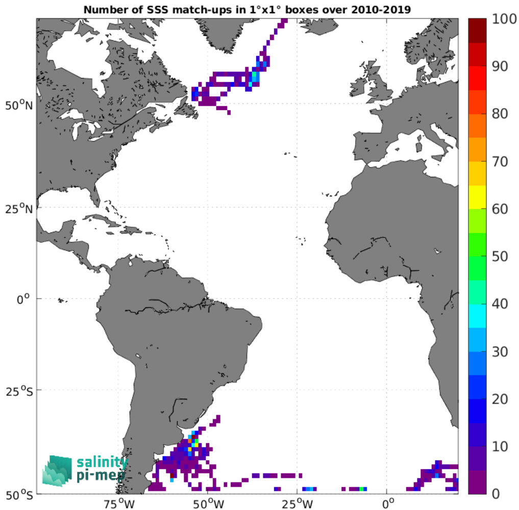
Figure 4: Number of SSS match-ups between Marine mammals SSS and the CCI SSS L4 Merged-OI v4.4 - 30-day running (ESA) SSS product for the Atlantic Ocean Pi-MEP region over 1°x1° boxes and for the full satellite product period.
