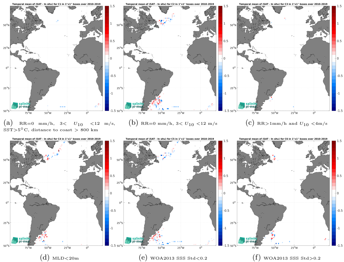
Figure 12: Temporal mean gridded over spatial boxes of size 1^\circ \times 1^\circ of \Delta SSS (CCI SSS L4 Merged-OI v4.4 - 30-day running (ESA) - Marine mammals) for 6 different subdatasets corresponding to:RR=0 mm/h, 3 < U_{10} < 12 m/s, SST >5^\circ C, distance to coast > 800 km (a), RR=0 mm/h, 3 < U_{10} < 12 m/s (b), RR >1 mm/h and U_{10} < 4 m/s (c),MLD <20 m (d),WOA2013 SSS Std <0.2 (e),WOA2013 SSS Std >0.2 (f).
