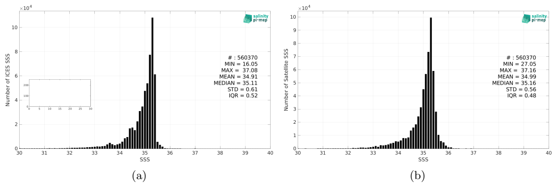
Figure 2: Histograms of SSS from ICES (a) and CCI SSS L4 Merged-OI v4.4 - 30-day running (ESA) (b) considering all match-up pairs per bins of 0.1 over the Atlantic Ocean Pi-MEP region and for the full satellite product period.
