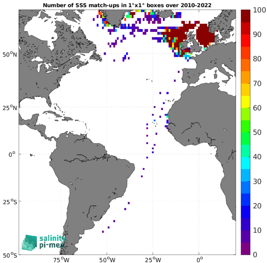
Figure 4: Number of SSS match-ups between ICES SSS and the CCI SSS L4 Merged-OI v4.4 - 30-day running (ESA) SSS product for the Atlantic Ocean Pi-MEP region over 1^\circ \times 1^\circ boxes and for the full satellite product period.
