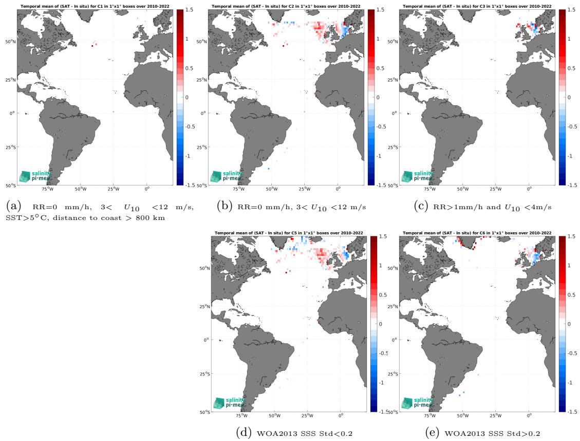
Figure 12: Temporal mean gridded over spatial boxes of size 1^\circ \times 1^\circ of \Delta\text{SSS} (CCI SSS L4 Merged-OI v4.4 - 30-day running (ESA) - ICES) for 5 different subdatasets corresponding to:RR=0 mm/h, 3 < U_{10} < 12 m/s, SST >5^\circ\text{C} , distance to coast > 800 km (a), RR=0 mm/h, 3 < U_{10} < 12 m/s (b), RR >1 mm/h and U_{10} < 4 m/s (c), WOA2013 SSS Std <0.2 (d), WOA2013 SSS Std >0.2 (e).
