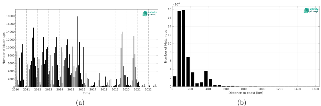
Figure 1: Number of match-ups between ICES and CCI SSS L4 Merged-OI v4.4 - 30-day running (ESA) SSS as a function of time (a) and as function of the distance to coast (b) over the Atlantic Ocean Pi-MEP region and for the full satellite product period.
