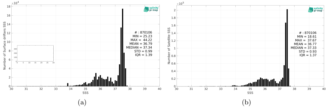
Figure 2: Histograms of SSS from Surface drifters (a) and CCI SSS L4 Merged-OI v4.4 - 30-day running (ESA) (b) considering all match-up pairs per bins of 0.1 over the Atlantic Ocean Pi-MEP region and for the full satellite product period.
