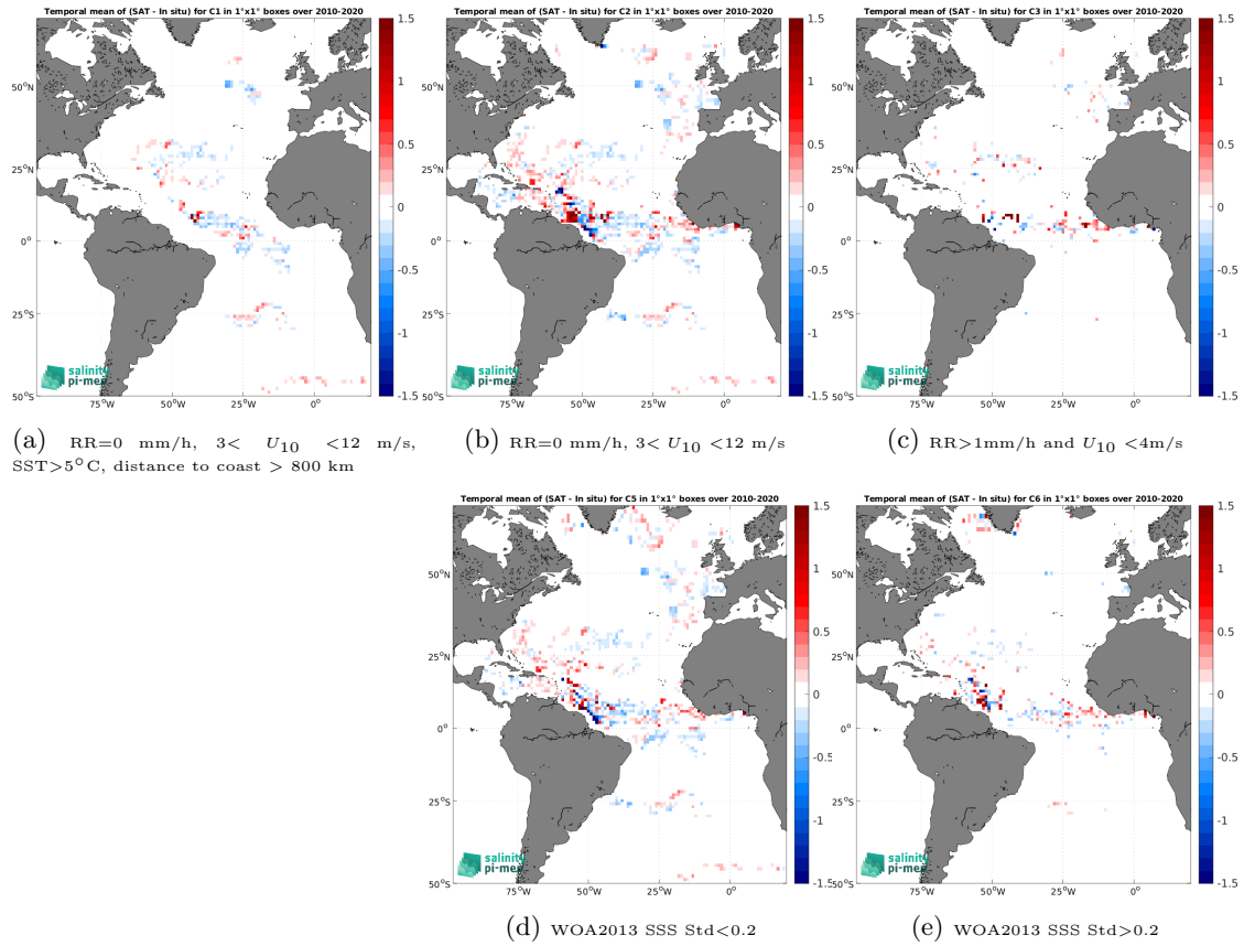
Figure 11: Temporal mean gridded over spatial boxes of size 1^\circ \times 1^\circ of \Delta\text{SSS} (CCI SSS L4 Merged-OI v4.4 - 30-day running (ESA) - Surface drifters) for 5 different subdatasets corresponding to:RR=0 mm/h, 3 < U_{10} < 12 m/s, SST >5^\circ\text{C} , distance to coast > 800 km (a), RR=0 mm/h, 3 < U_{10} < 12 m/s (b), RR >1 mm/h and U_{10} < 4 m/s (c), WOA2013 SSS Std <0.2 (d), WOA2013 SSS Std >0.2 (e).
