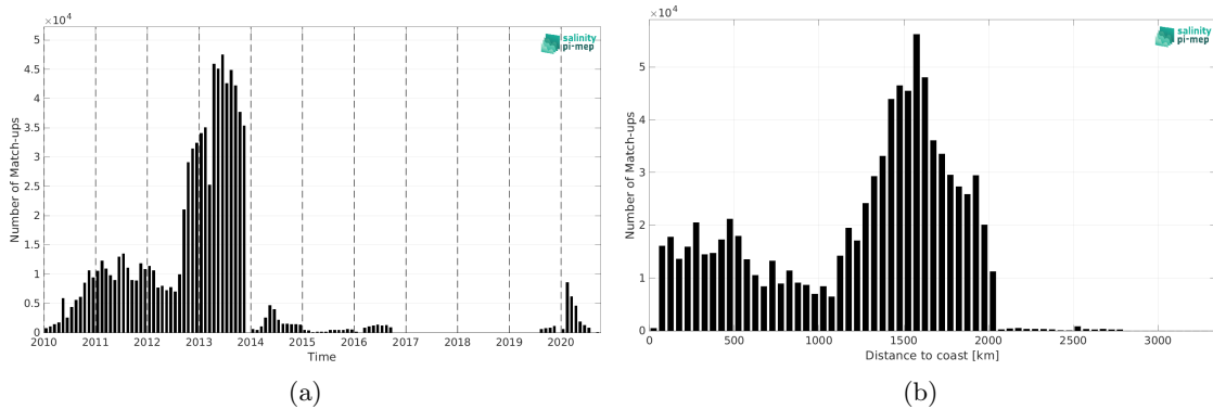
Figure 1: Number of match-ups between Surface drifters and CCI SSS L4 Merged-OI v4.4 - 30-day running (ESA) SSS as a function of time (a) and as function of the distance to coast (b) over the Atlantic Ocean Pi-MEP region and for the full satellite product period.
