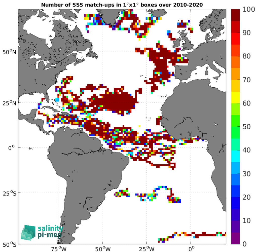
Figure 3: Number of SSS match-ups between Surface drifters SSS and the CCI SSS L4 Merged-OI v4.4 - 30-day running (ESA) SSS product for the Atlantic Ocean Pi-MEP region over 1^\circ \times 1^\circ boxes and for the full satellite product period.
