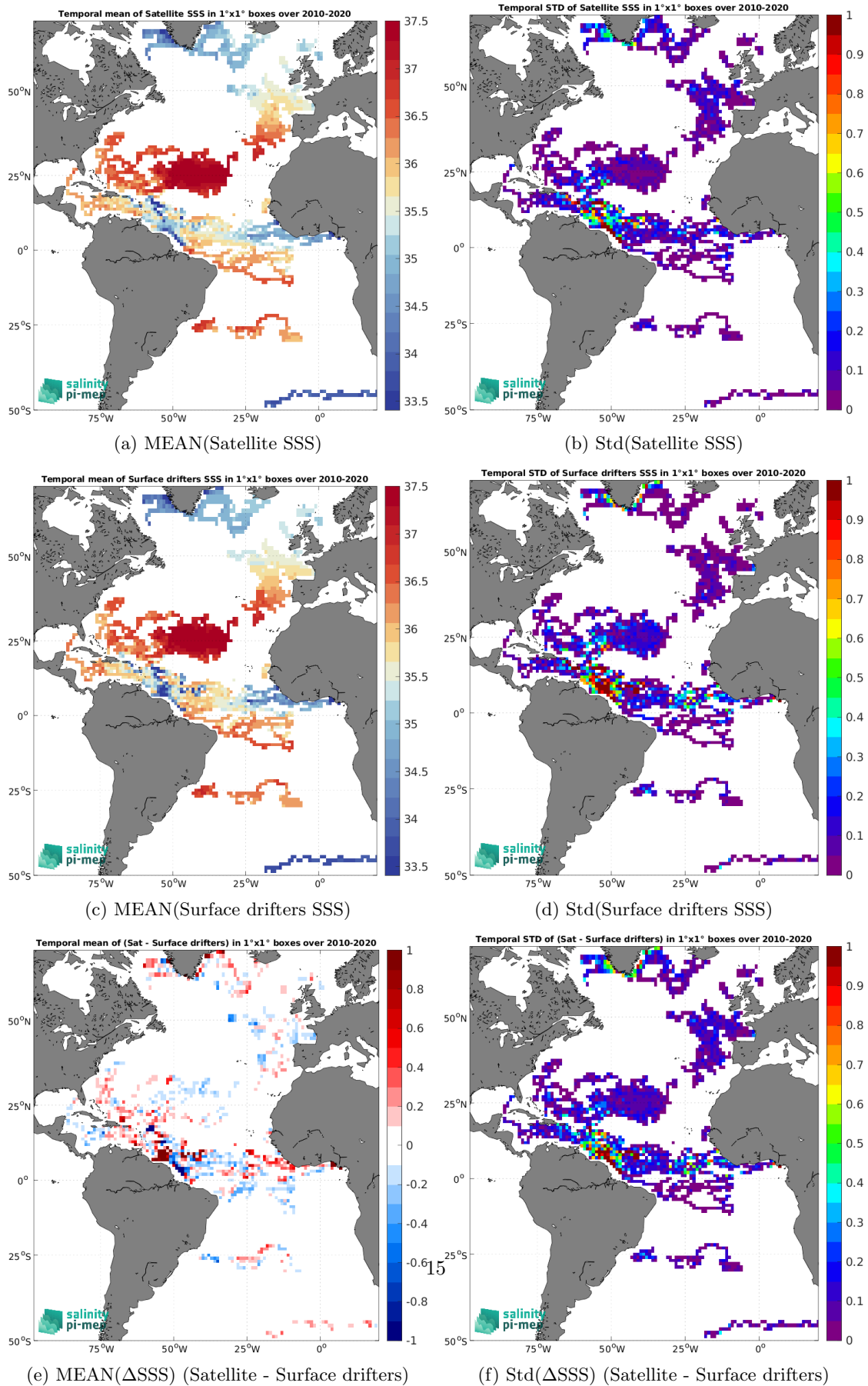
Figure 5: Temporal mean (left) and Std (right) of SSS from CCI SSS L4 Merged-OI v4.4 - 30-day running (ESA) (top), Surface drifters (middle), and of \Delta SSS (Satellite - Surface drifters). Only match-up pairs are used to generate these maps.
