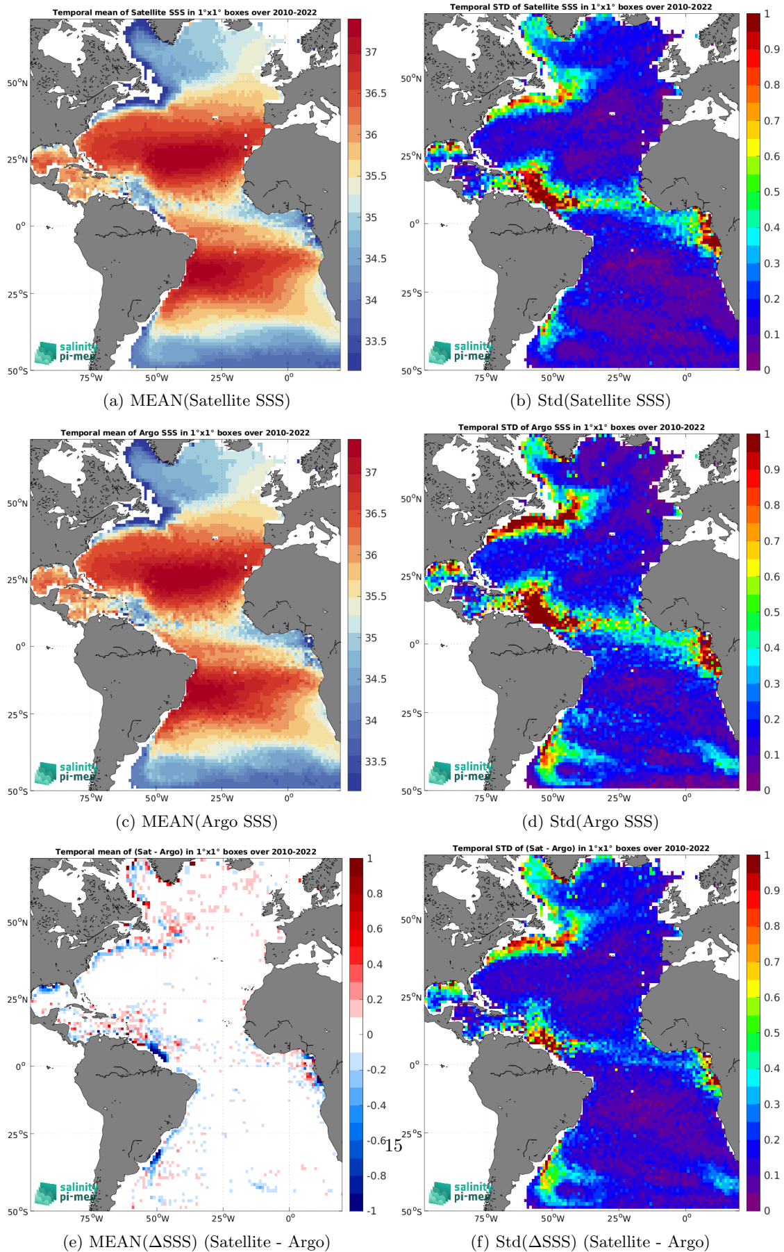
Figure 6: Temporal mean (left) and Std (right) of SSS from CCI SSS L4 Merged-OI v4.4 - 30-day running (ESA) (top), Argo (middle), and of \Delta SSS (Satellite - Argo). Only match-up pairs are used to generate these maps.
