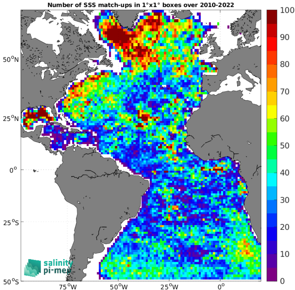
Figure 4: Number of SSS match-ups between Argo SSS and the CCI SSS L4 Merged-OI v4.4 - 30-day running (ESA) SSS product for the Atlantic Ocean Pi-MEP region over 1^\circ \times 1^\circ boxes and for the full satellite product period.
