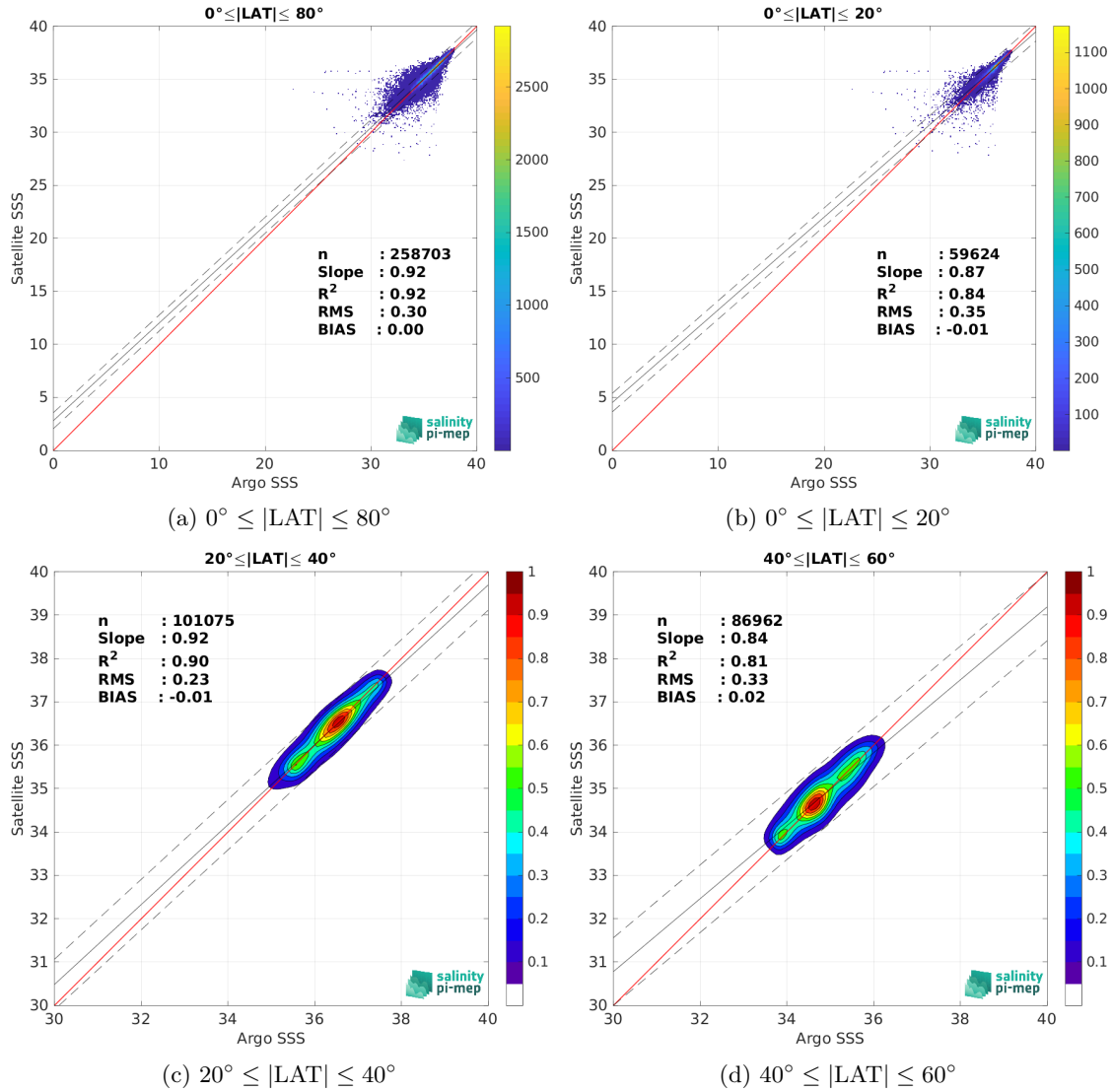
Figure 9: Contour maps of the concentration of CCI SSS L4 Merged-OI v4.4 - 30-day running (ESA) SSS (y-axis) versus Argo SSS (x-axis) at match-up pairs for different latitude bands. For each plot, the red line shows x=y . The black thin and dashed lines indicate a linear fit through the data cloud and the \pm 95\% confidence levels, respectively. The number match-up pairs n , the slope and R^2 coefficient of the linear fit, the root mean square (RMS) and the mean bias between satellite and in situ data are indicated for each latitude band in each plots.
