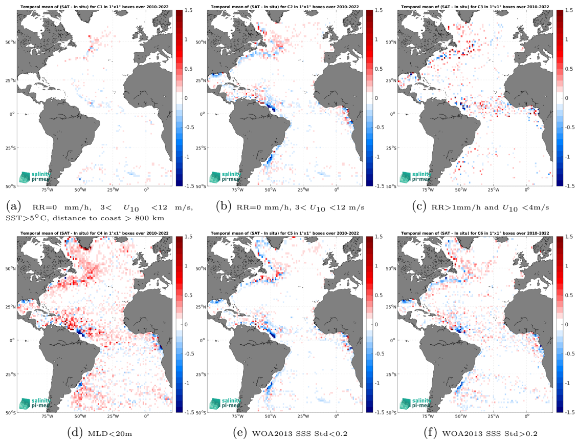
Figure 12: Temporal mean gridded over spatial boxes of size 1^\circ \times 1^\circ of \Delta SSS (CCI SSS L4 Merged-OI v4.4 - 30-day running (ESA) - Argo) for 6 different subdatasets corresponding to:RR=0 mm/h, 3 < U_{10} < 12 m/s, SST >5^\circ C, distance to coast > 800 km (a), RR=0 mm/h, 3 < U_{10} < 12 m/s (b), RR >1 mm/h and U_{10} < 4 m/s (c),MLD <20 m (d),WOA2013 SSS Std <0.2 (e),WOA2013 SSS Std >0.2 (f).
