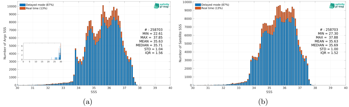
Figure 2: Histograms of SSS from Argo (a) and CCI SSS L4 Merged-OI v4.4 - 30-day running (ESA) (b) considering all match-up pairs per bins of 0.1 over the Atlantic Ocean Pi-MEP region and for the full satellite product period.
