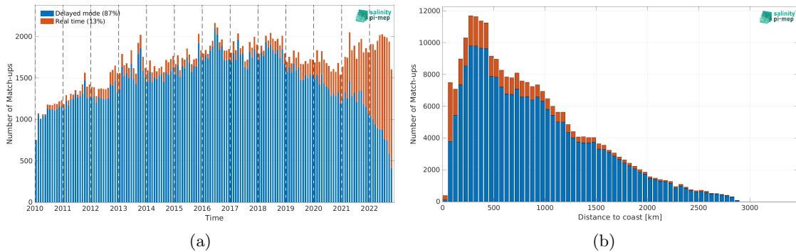
Figure 1: Number of match-ups between Argo and CCI SSS L4 Merged-OI v4.4 - 30-day running (ESA) SSS as a function of time (a) and as function of the distance to coast (b) over the Atlantic Ocean Pi-MEP region and for the full satellite product period.
