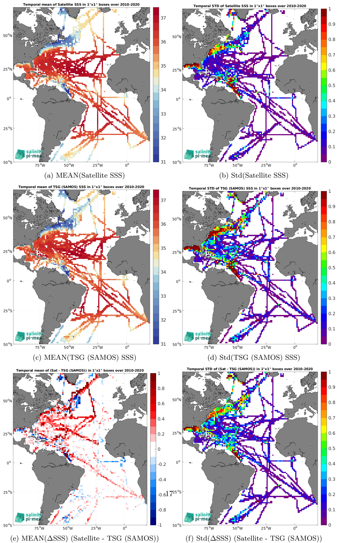
Figure 6: Temporal mean (left) and Std (right) of SSS from CCI SSS L4 Merged-OI v3.2 - 7-day running (ESA) (top), TSG (SAMOS) (middle), and of \Delta SSS (Satellite - TSG (SAMOS)). Only match-up pairs are used to generate these maps.
