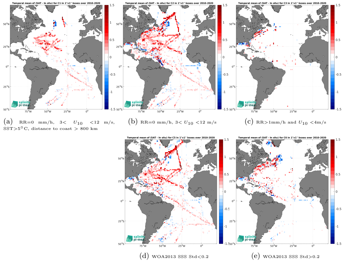
Figure 12: Temporal mean gridded over spatial boxes of size 1^\circ \times 1^\circ of \Delta\text{SSS} (CCI SSS L4 Merged-OI v3.2 - 7-day running (ESA) - TSG (SAMOS)) for 5 different subdatasets corresponding to:RR=0 mm/h, 3 < U_{10} < 12 m/s, SST >5^\circ\text{C} , distance to coast > 800 km (a), RR=0 mm/h, 3 < U_{10} < 12 m/s (b), RR >1 mm/h and U_{10} < 4 m/s (c), WOA2013 SSS Std <0.2 (d), WOA2013 SSS Std >0.2 (e).
