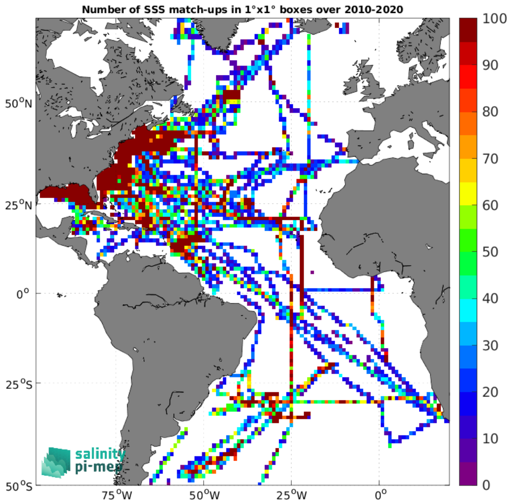
Figure 4: Number of SSS match-ups between TSG (SAMOS) SSS and the CCI SSS L4 Merged-OI v3.2 - 7-day running (ESA) SSS product for the Atlantic Ocean Pi-MEP region over 1°x1° boxes and for the full satellite product period.
