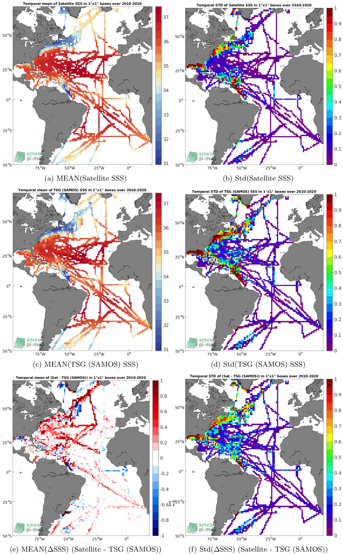
(e) MEAN( \Delta SSS) (Satellite - TSG (SAMOS)) (f) Std( \Delta SSS) (Satellite - TSG (SAMOS)) Figure 6: Temporal mean (left) and Std (right) of SSS from CCI SSS L4 Merged-OI v3.2 - 7-day running (ESA) (top), TSG (SAMOS) (middle), and of \Delta SSS (Satellite - TSG (SAMOS)). Only match-up pairs are used to generate these maps.
