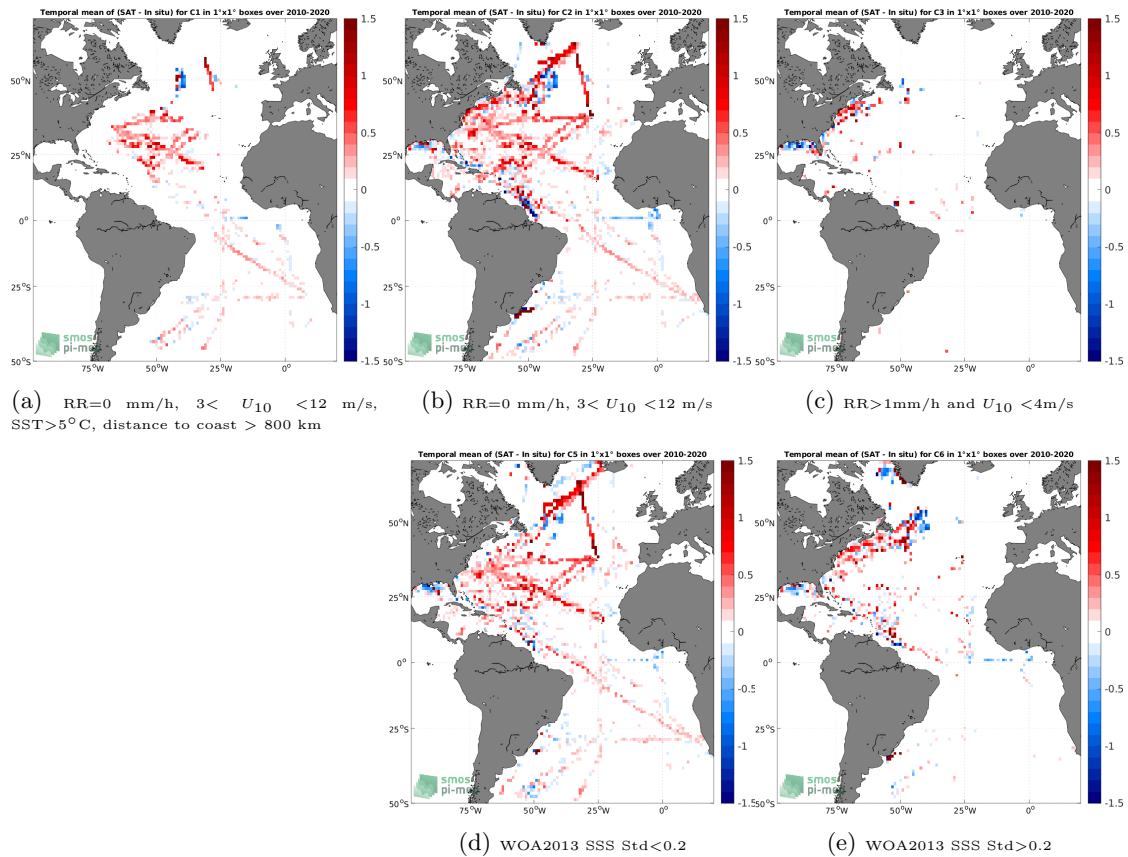
Figure 12: Temporal mean gridded over spatial boxes of size 1^\circ \times 1^\circ of \Delta SSS (CCI SSS L4 Merged-OI v3.2 - 7-day running (ESA) - TSG (SAMOS)) for 5 different subdatasets corresponding to:RR=0 mm/h, 3 < U_{10} < 12 m/s, SST >5^\circ\text{C} , distance to coast > 800 km (a), RR=0 mm/h, 3 < U_{10} < 12 m/s (b), RR >1 mm/h and U_{10} < 4 m/s (c), WOA2013 SSS Std <0.2 (d), WOA2013 SSS Std >0.2 (e).
