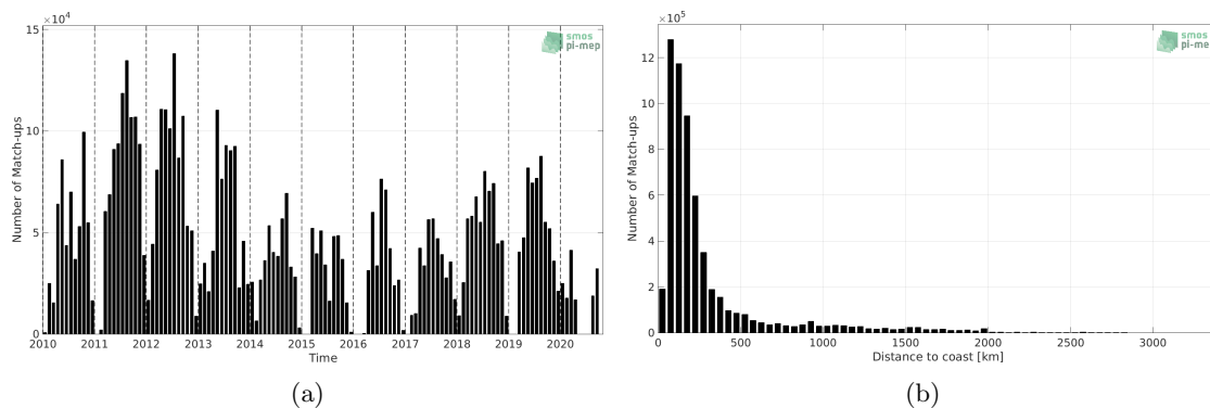
Figure 1: Number of match-ups between TSG (SAMOS) and CCI SSS L4 Merged-OI v3.2 - 7-day running (ESA) SSS as a function of time (a) and as function of the distance to coast (b) over the Atlantic Ocean Pi-MEP region and for the full satellite product period.
