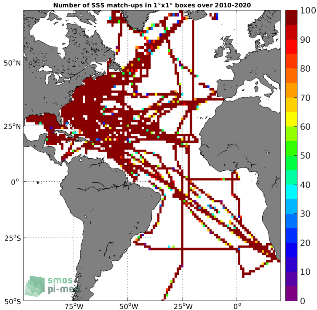
Figure 4: Number of SSS match-ups between TSG (SAMOS) SSS and the CCI SSS L4 Merged-OI v3.2 - 7-day running (ESA) SSS product for the Atlantic Ocean Pi-MEP region over 1^\circ \times 1^\circ boxes and for the full satellite product period.
