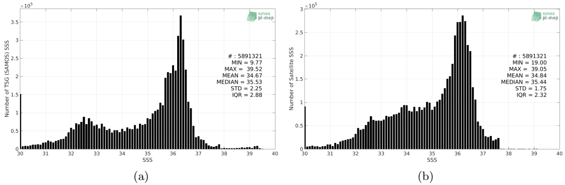
Figure 2: Histograms of SSS from TSG (SAMOS) (a) and CCI SSS L4 Merged-OI v3.2 - 7-day running (ESA) (b) considering all match-up pairs per bins of 0.1 over the Atlantic Ocean Pi-MEP region and for the full satellite product period.
