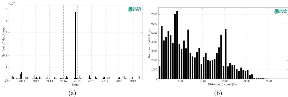
Figure 1: Number of match-ups between TSG (Polarstern) and CCI SSS L4 Merged-OI v3.2 - 7-day running (ESA) SSS as a function of time (a) and as function of the distance to coast (b) over the Atlantic Ocean Pi-MEP region and for the full satellite product period.
