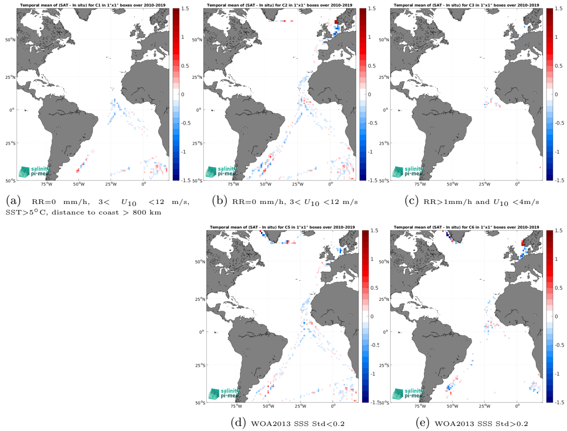
Figure 12: Temporal mean gridded over spatial boxes of size 1^\circ \times 1^\circ of \Delta SSS (CCI SSS L4 Merged-OI v3.2 - 7-day running (ESA) - TSG (Polarstern)) for 5 different subdatasets corresponding to:RR=0 mm/h, 3 < U_{10} < 12 m/s, SST >5^\circ\text{C} , distance to coast > 800 km (a), RR=0 mm/h, 3 < U_{10} < 12 m/s (b), RR >1 mm/h and U_{10} < 4 m/s (c), WOA2013 SSS Std <0.2 (d), WOA2013 SSS Std >0.2 (e).
