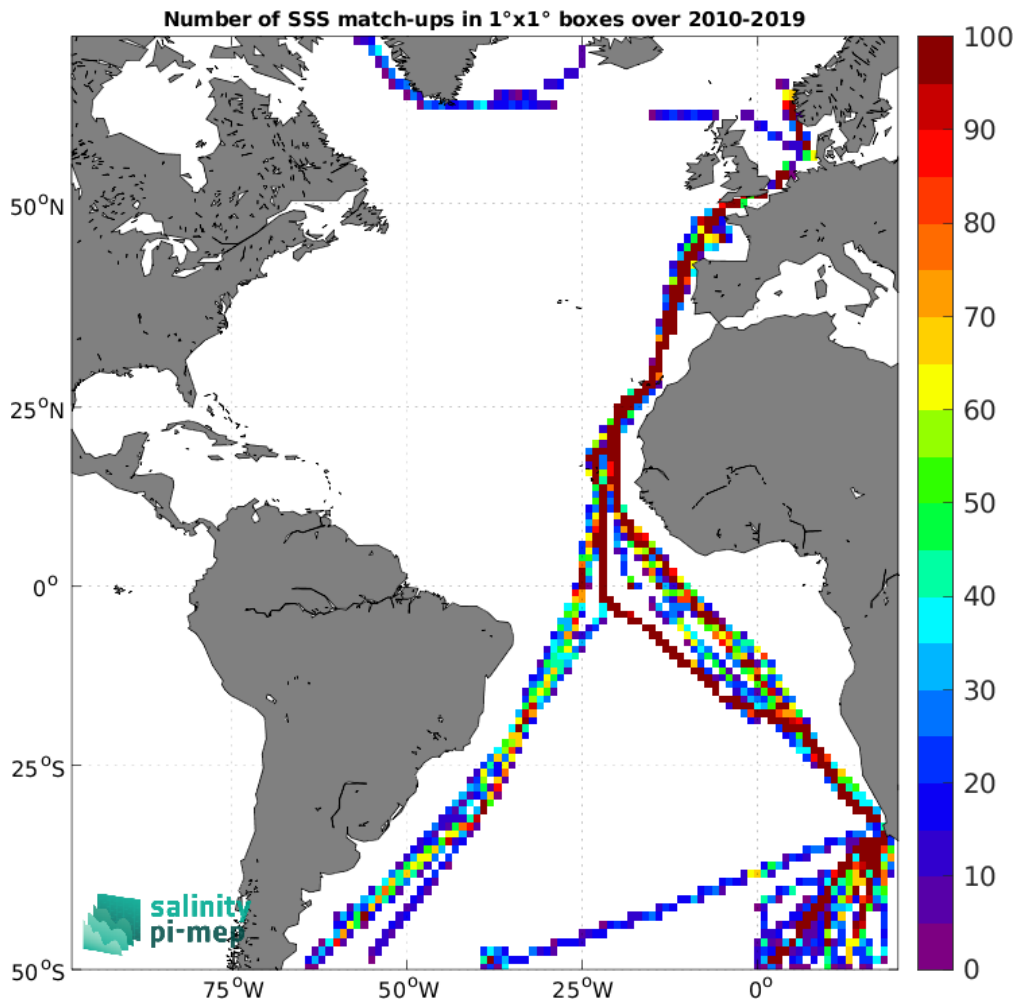
Figure 4: Number of SSS match-ups between TSG (Polarstern) SSS and the CCI SSS L4 Merged-OI v3.2 - 7-day running (ESA) SSS product for the Atlantic Ocean Pi-MEP region over 1°x1° boxes and for the full satellite product period.
