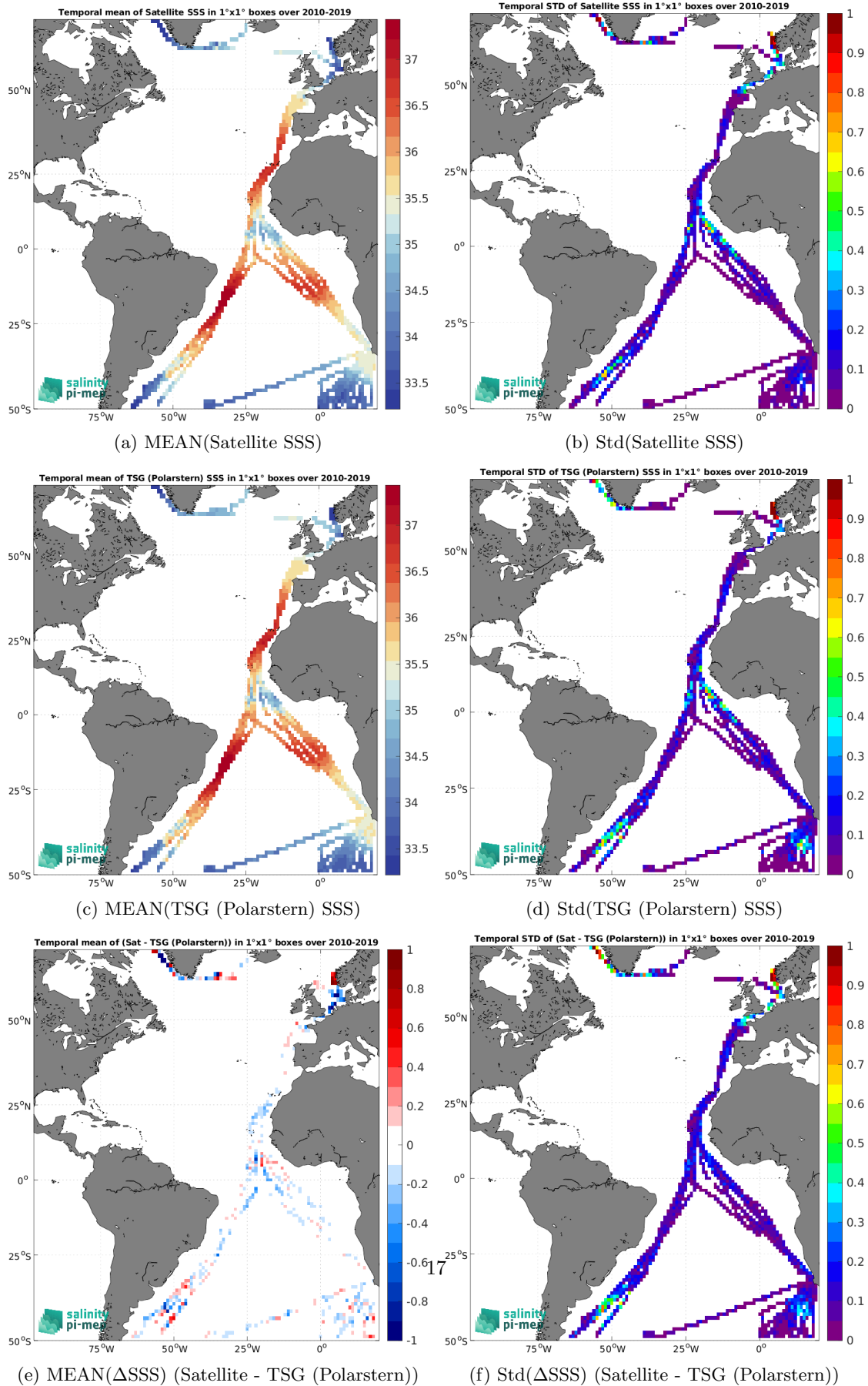
Figure 6: Temporal mean (left) and Std (right) of SSS from CCI SSS L4 Merged-OI v3.2 - 7-day running (ESA) (top), TSG (Polarstern) (middle), and of \Delta SSS (Satellite - TSG (Polarstern)). Only match-up pairs are used to generate these maps.
