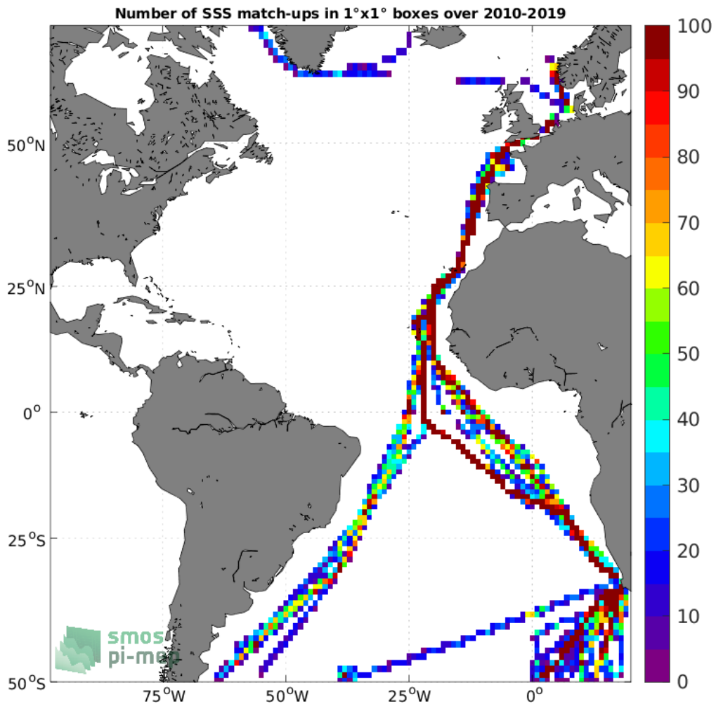
Figure 4: Number of SSS match-ups between TSG (Polarstern) SSS and the CCI SSS L4 Merged-OI v3.2 - 7-day running (ESA) SSS product for the Atlantic Ocean Pi-MEP region over 1°×1° boxes and for the full satellite product period.
