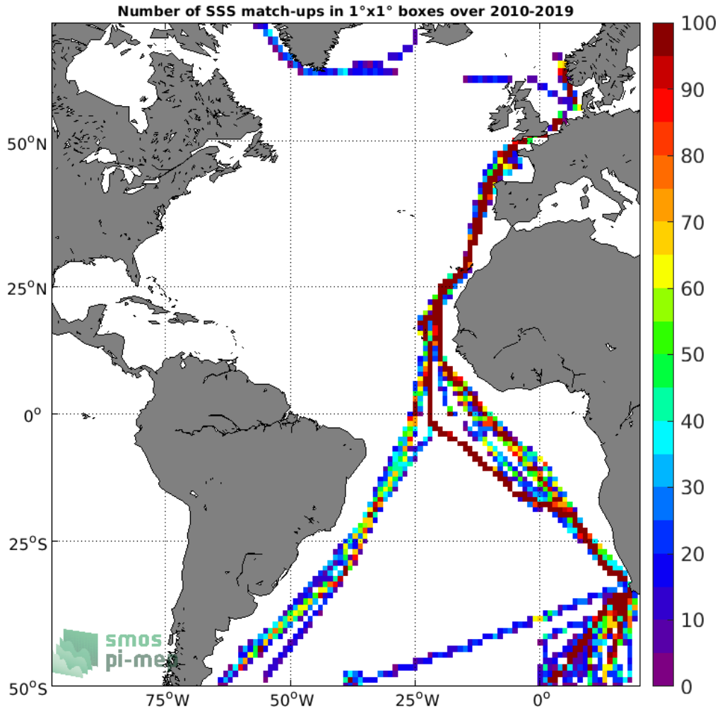
Figure 4: Number of SSS match-ups between TSG (Polarstern) SSS and the CCI SSS L4 Merged-OI v3.2 - 7-day running (ESA) SSS product for the Atlantic Ocean Pi-MEP region over 1^\circ \times 1^\circ boxes and for the full satellite product period.
