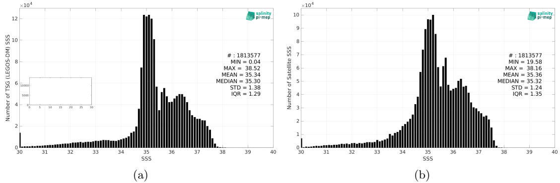
Figure 2: Histograms of SSS from TSG (LEGOS-DM) (a) and CCI SSS L4 Merged-OI v3.2 - 7-day running (ESA) (b) considering all match-up pairs per bins of 0.1 over the Atlantic Ocean Pi-MEP region and for the full satellite product period.
