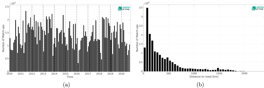
Figure 1: Number of match-ups between TSG (LEGOS-DM) and CCI SSS L4 Merged-OI v3.2 - 7-day running (ESA) SSS as a function of time (a) and as function of the distance to coast (b) over the Atlantic Ocean Pi-MEP region and for the full satellite product period.
