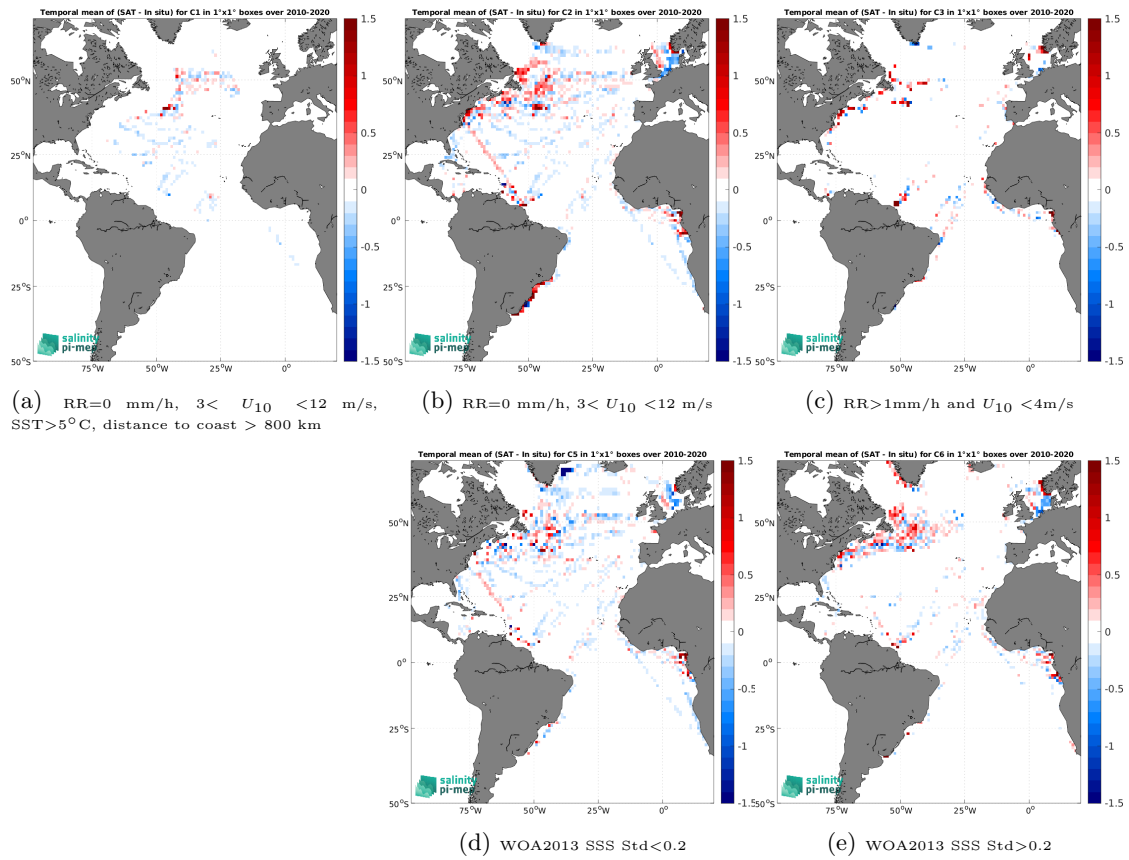
Figure 12: Temporal mean gridded over spatial boxes of size 1^\circ \times 1^\circ of \Delta\text{SSS} (CCI SSS L4 Merged-OI v3.2 - 7-day running (ESA) - TSG (LEGOS-DM)) for 5 different subdatasets corresponding to:RR=0 mm/h, 3 < U_{10} < 12 m/s, SST >5^\circ\text{C} , distance to coast > 800 km (a), RR=0 mm/h, 3 < U_{10} < 12 m/s (b), RR >1 mm/h and U_{10} < 4 m/s (c), WOA2013 SSS Std <0.2 (d), WOA2013 SSS Std >0.2 (e).
