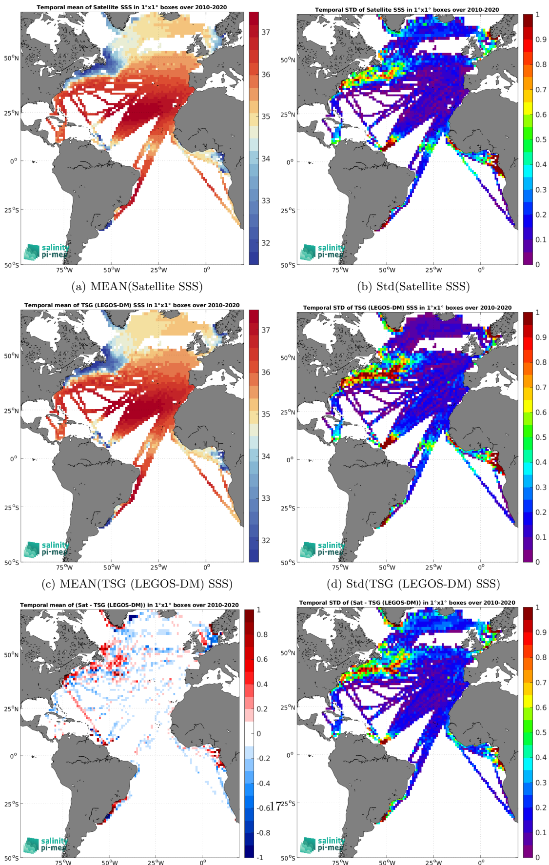
Figure 6: Temporal mean (left) and Std (right) of SSS from CCI SSS L4 Merged-OI v3.2 - 7-day running (ESA) (top), TSG (LEGOS-DM) (middle), and of \Delta SSS (Satellite - TSG (LEGOS-DM)). Only match-up pairs are used to generate these maps.
