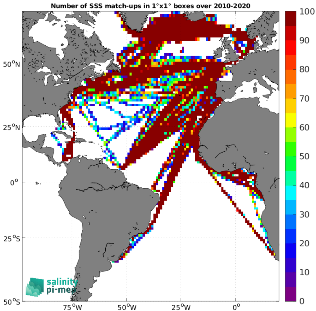
Figure 4: Number of SSS match-ups between TSG (LEGOS-DM) SSS and the CCI SSS L4 Merged-OI v3.2 - 7-day running (ESA) SSS product for the Atlantic Ocean Pi-MEP region over 1^\circ \times 1^\circ boxes and for the full satellite product period.
