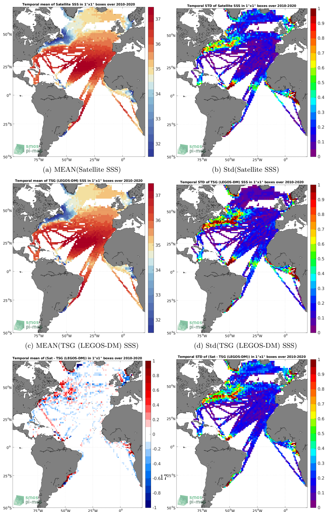
(e) MEAN( \Delta SSS) (Satellite - TSG (LEGOS-DM)) (f) Std( \Delta SSS) (Satellite - TSG (LEGOS-DM)) Figure 6: Temporal mean (left) and Std (right) of SSS from CCI SSS L4 Merged-OI v3.2 - 7-day running (ESA) (top), TSG (LEGOS-DM) (middle), and of \Delta SSS (Satellite - TSG (LEGOS-DM)). Only match-up pairs are used to generate these maps.
