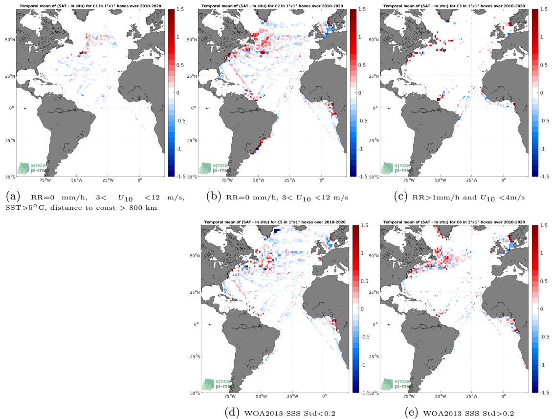
Figure 12: Temporal mean gridded over spatial boxes of size 1^\circ \times 1^\circ of \Delta SSS (CCI SSS L4 Merged-OI v3.2 - 7-day running (ESA) - TSG (LEGOS-DM)) for 5 different subdatasets corresponding to:RR=0 mm/h, 3 < U_{10} < 12 m/s, SST >5^\circ\text{C} , distance to coast > 800 km (a), RR=0 mm/h, 3 < U_{10} < 12 m/s (b), RR >1 mm/h and U_{10} < 4 m/s (c), WOA2013 SSS Std <0.2 (d), WOA2013 SSS Std >0.2 (e).
