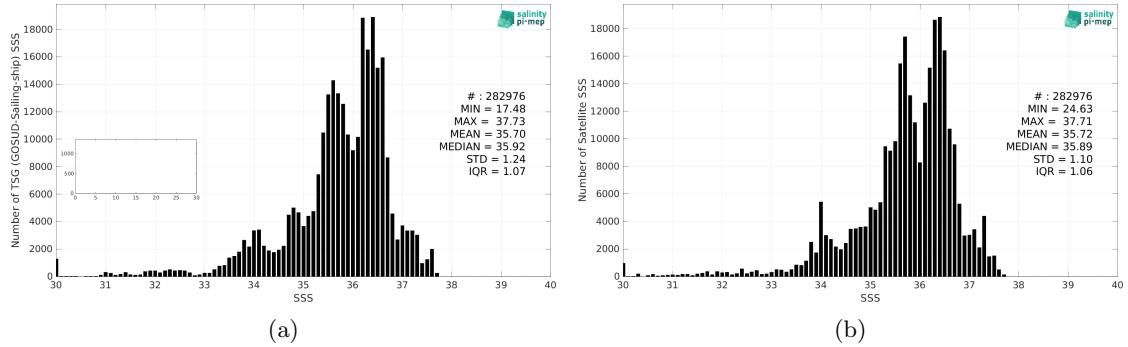
Figure 2: Histograms of SSS from TSG (GOSUD-Sailing-ship) (a) and CCI SSS L4 Merged-OI v3.2 - 7-day running (ESA) (b) considering all match-up pairs per bins of 0.1 over the Atlantic Ocean Pi-MEP region and for the full satellite product period.
