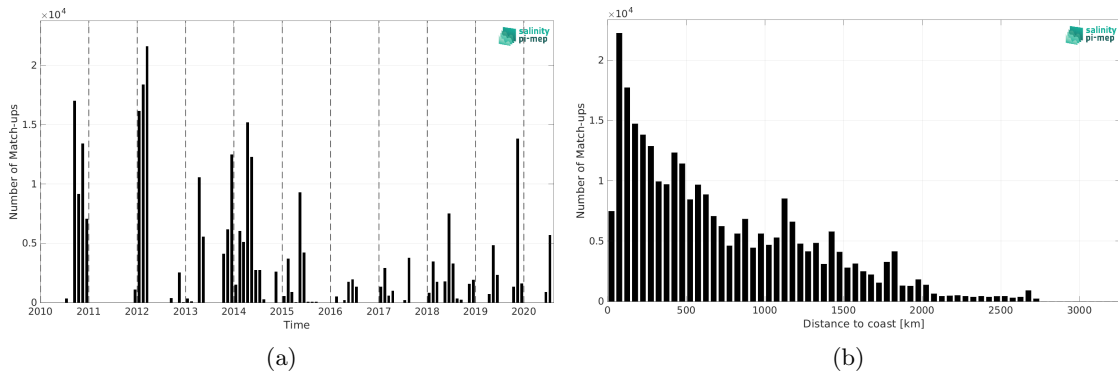
Figure 1: Number of match-ups between TSG (GOSUD-Sailing-ship) and CCI SSS L4 Merged-OI v3.2 - 7-day running (ESA) SSS as a function of time (a) and as function of the distance to coast (b) over the Atlantic Ocean Pi-MEP region and for the full satellite product period.
