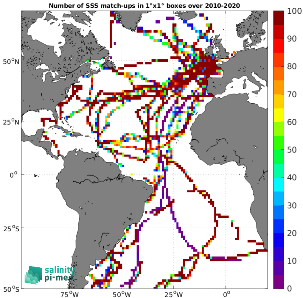
Figure 4: Number of SSS match-ups between TSG (GOSUD-Sailing-ship) SSS and the CCI SSS L4 Merged-OI v3.2 - 7-day running (ESA) SSS product for the Atlantic Ocean Pi-MEP region over 1^\circ \times 1^\circ boxes and for the full satellite product period.
