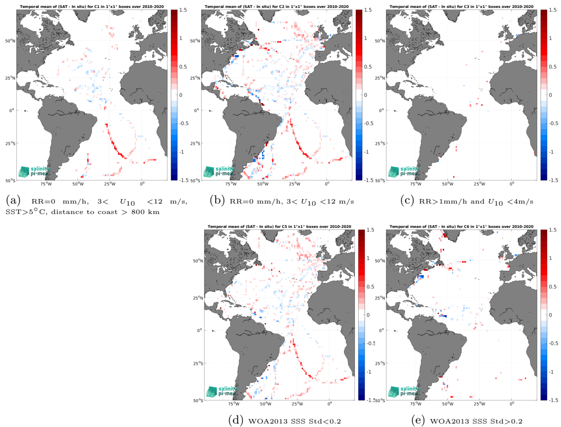
Figure 12: Temporal mean gridded over spatial boxes of size 1^\circ \times 1^\circ of \Delta\text{SSS} (CCI SSS L4 Merged-OI v3.2 - 7-day running (ESA) - TSG (GOSUD-Sailing-ship)) for 5 different subdatasets corresponding to:RR=0 mm/h, 3 < U_{10} < 12 m/s, SST>5°C, distance to coast > 800 km (a), RR=0 mm/h, 3 < U_{10} < 12 m/s (b), RR>1mm/h and U_{10} < 4 m/s (c), WOA2013 SSS Std<0.2 (d), WOA2013 SSS Std>0.2 (e).
