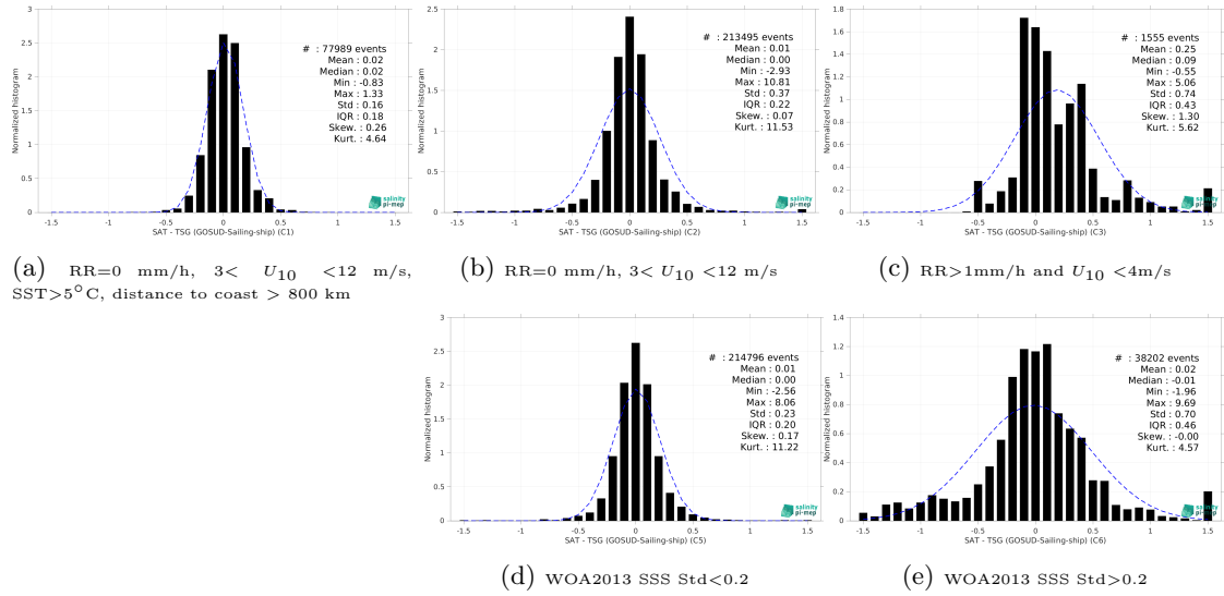
Figure 13: Normalized histogram of \Delta\text{SSS} (CCI SSS L4 Merged-OI v3.2 - 7-day running (ESA) - TSG (GOSUD-Sailing-ship)) for 5 different subdatasets corresponding to: RR=0 mm/h, 3 < U_{10} < 12 m/s, SST>5°C, distance to coast > 800 km (a), RR=0 mm/h, 3 < U_{10} < 12 m/s (b), RR>1mm/h and U_{10} < 4 m/s (c), WOA2013 SSS Std<0.2 (d), WOA2013 SSS Std>0.2 (e).
