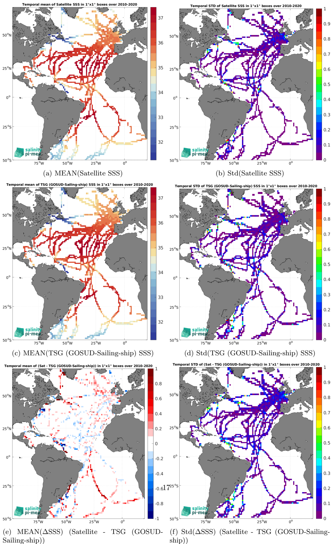
Figure 6: Temporal mean (left) and Std (right) of SSS from CCI SSS L4 Merged-OI v3.2 - 7-day running (ESA) (top), TSG (GOSUD-Sailing-ship) (middle), and of \Delta SSS (Satellite - TSG (GOSUD-Sailing-ship)). Only match-up pairs are used to generate these maps.
