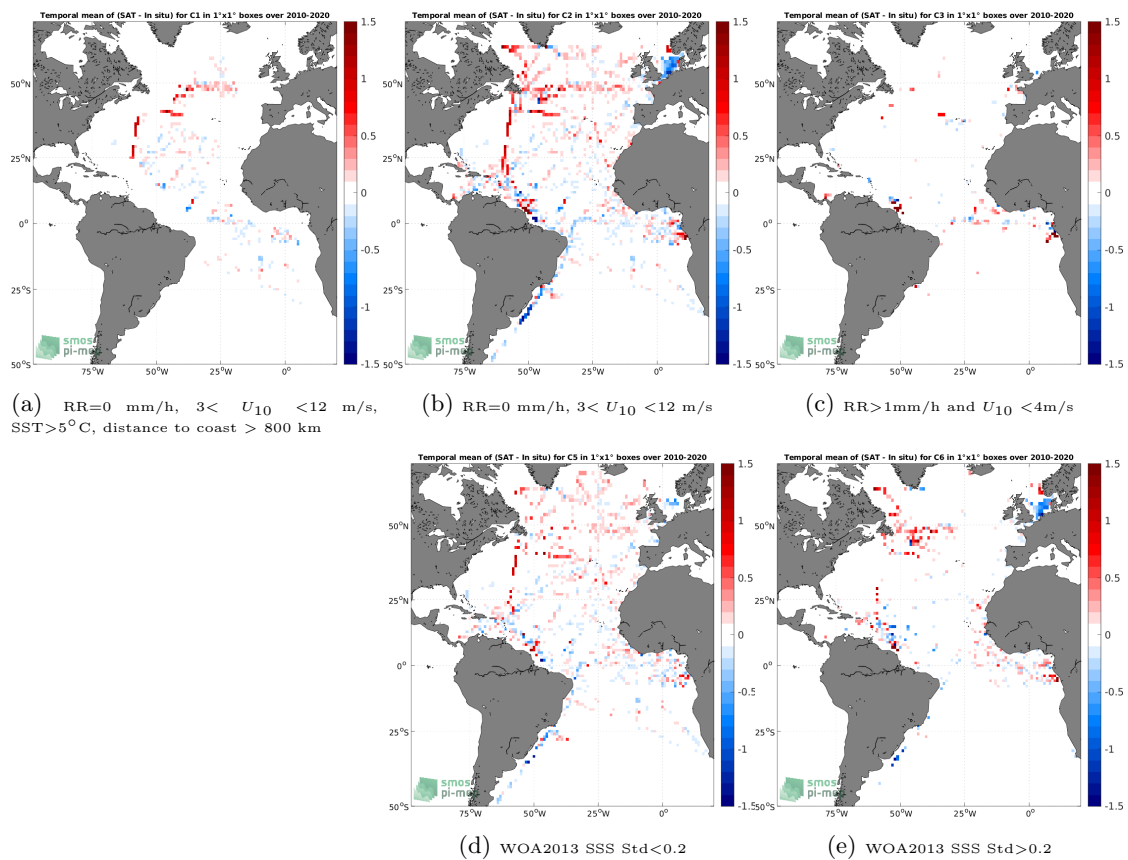
Figure 12: Temporal mean gridded over spatial boxes of size 1^\circ \times 1^\circ of \Delta\text{SSS} (CCI SSS L4 Merged-OI v3.2 - 7-day running (ESA) - TSG (GOSUD-Research-vessel)) for 5 different subdatasets corresponding to:RR=0 mm/h, 3 < U_{10} < 12 m/s, SST>5°C, distance to coast > 800 km (a), RR=0 mm/h, 3 < U_{10} < 12 m/s (b), RR>1mm/h and U_{10} < 4 m/s (c), WOA2013 SSS Std<0.2 (d), WOA2013 SSS Std>0.2 (e).
