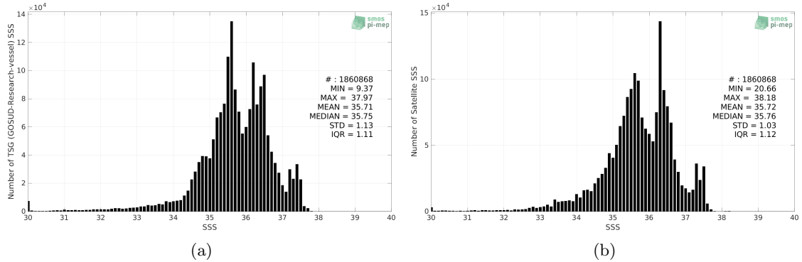
Figure 2: Histograms of SSS from TSG (GOSUD-Research-vessel) (a) and CCI SSS L4 Merged-OI v3.2 - 7-day running (ESA) (b) considering all match-up pairs per bins of 0.1 over the Atlantic Ocean Pi-MEP region and for the full satellite product period.
