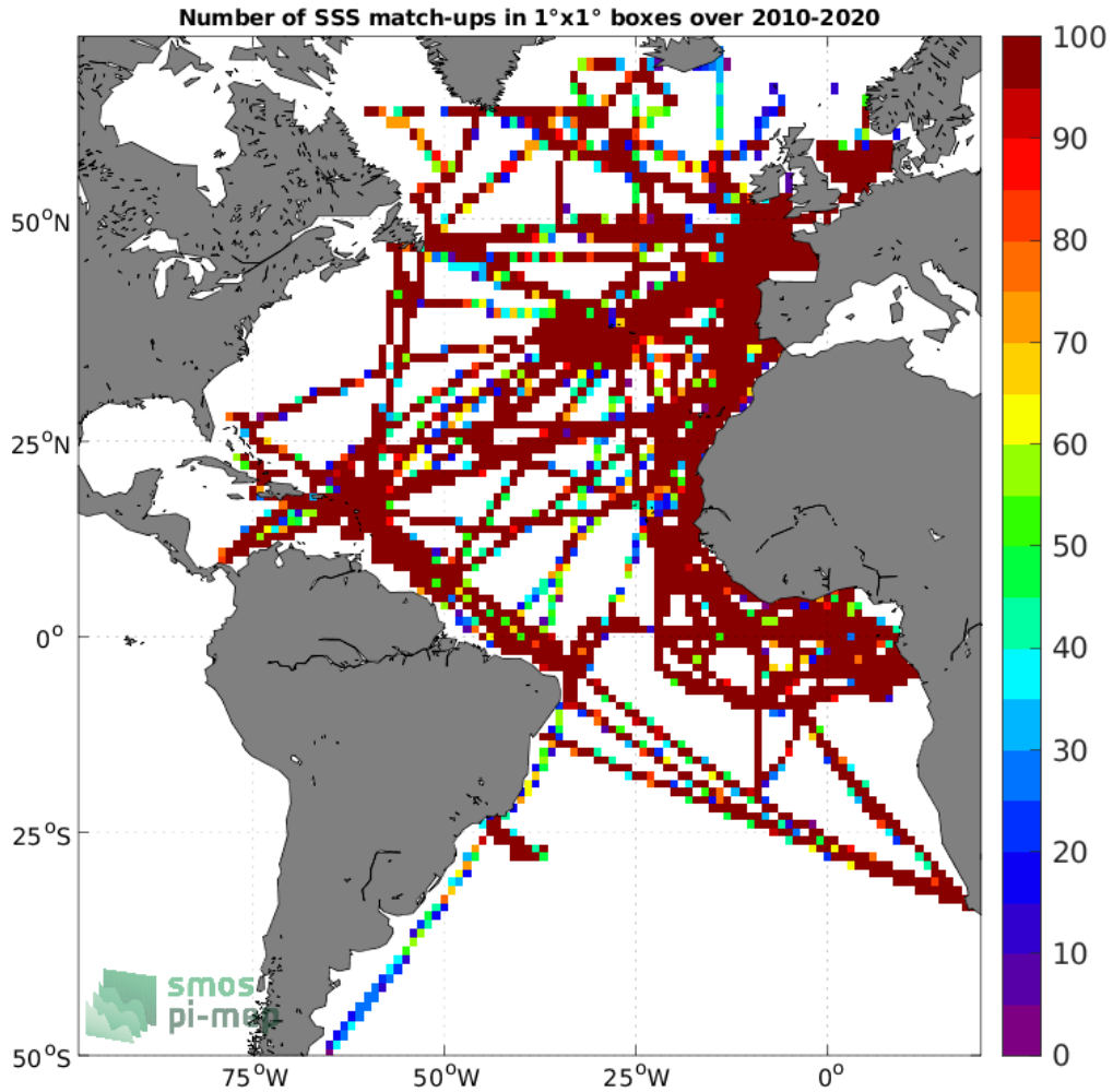
Figure 4: Number of SSS match-ups between TSG (GOSUD-Research-vessel) SSS and the CCI SSS L4 Merged-OI v3.2 - 7-day running (ESA) SSS product for the Atlantic Ocean Pi-MEP region over 1^\circ \times 1^\circ boxes and for the full satellite product period.
