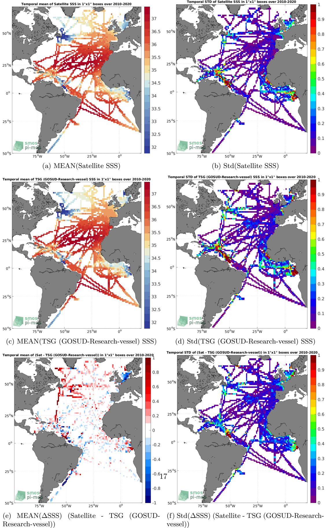
Figure 6: Temporal mean (left) and Std (right) of SSS from CCI SSS L4 Merged-OI v3.2 - 7-day running (ESA) (top), TSG (GOSUD-Research-vessel) (middle), and of \Delta SSS (Satellite - TSG (GOSUD-Research-vessel)). Only match-up pairs are used to generate these maps.
