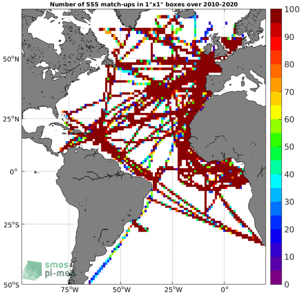
Figure 4: Number of SSS match-ups between TSG (GOSUD-Research-vessel) SSS and the CCI SSS L4 Merged-OI v3.2 - 7-day running (ESA) SSS product for the Atlantic Ocean Pi-MEP region over 1^\circ \times 1^\circ boxes and for the full satellite product period.
