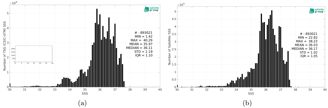
Figure 2: Histograms of SSS from TSG (CSIC-UTM) (a) and CCI SSS L4 Merged-OI v3.2 - 7-day running (ESA) (b) considering all match-up pairs per bins of 0.1 over the Atlantic Ocean Pi-MEP region and for the full satellite product period.
