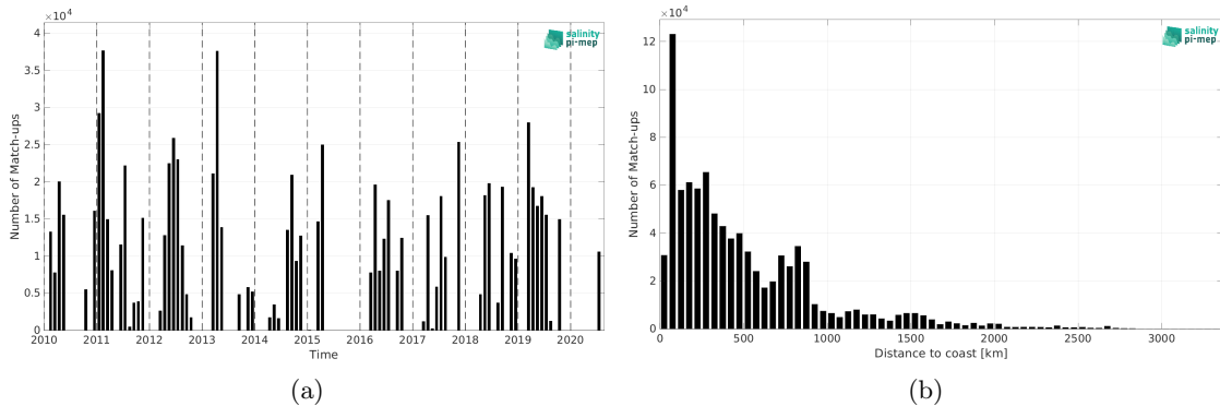
Figure 1: Number of match-ups between TSG (CSIC-UTM) and CCI SSS L4 Merged-OI v3.2 - 7-day running (ESA) SSS as a function of time (a) and as function of the distance to coast (b) over the Atlantic Ocean Pi-MEP region and for the full satellite product period.
