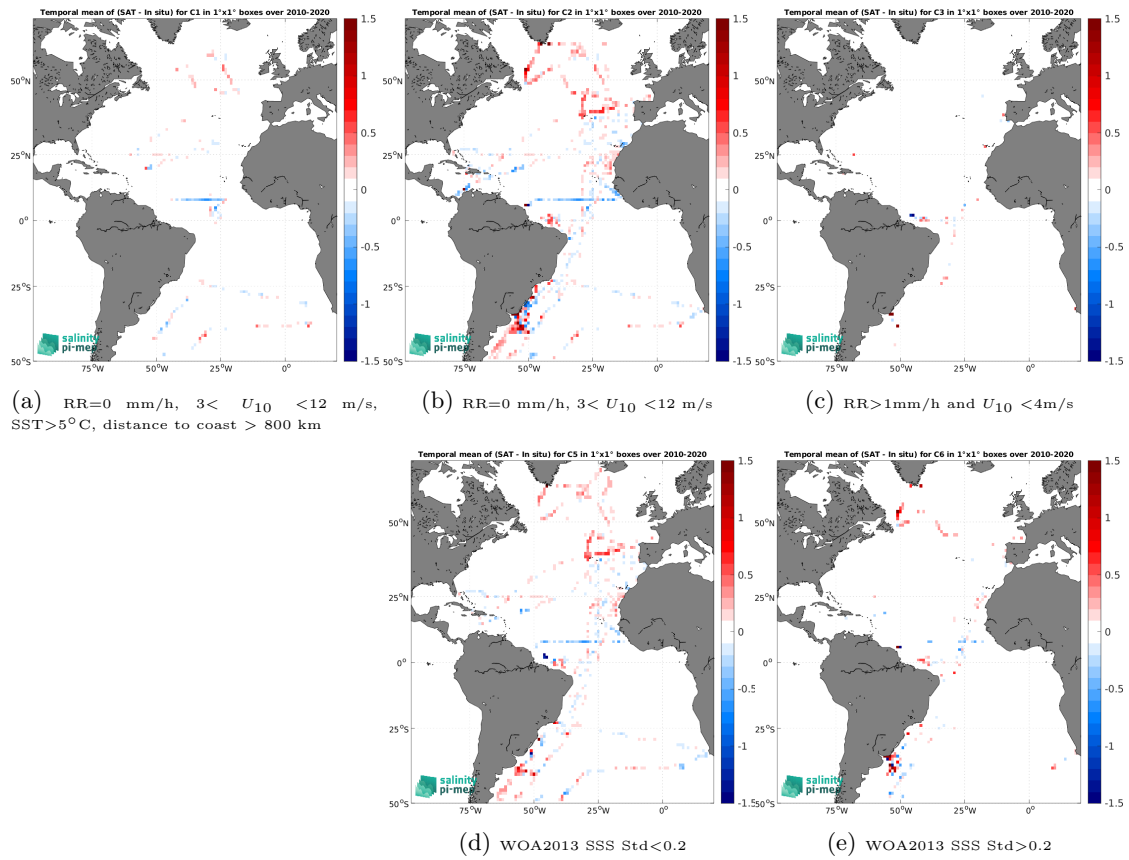
Figure 12: Temporal mean gridded over spatial boxes of size 1^\circ \times 1^\circ of \Delta\text{SSS} (CCI SSS L4 Merged-OI v3.2 - 7-day running (ESA) - TSG (CSIC-UTM)) for 5 different subdatasets corresponding to:RR=0 mm/h, 3 < U_{10} < 12 m/s, SST >5^\circ\text{C} , distance to coast > 800 km (a), RR=0 mm/h, 3 < U_{10} < 12 m/s (b), RR >1 mm/h and U_{10} < 4 m/s (c), WOA2013 SSS Std <0.2 (d), WOA2013 SSS Std >0.2 (e).
