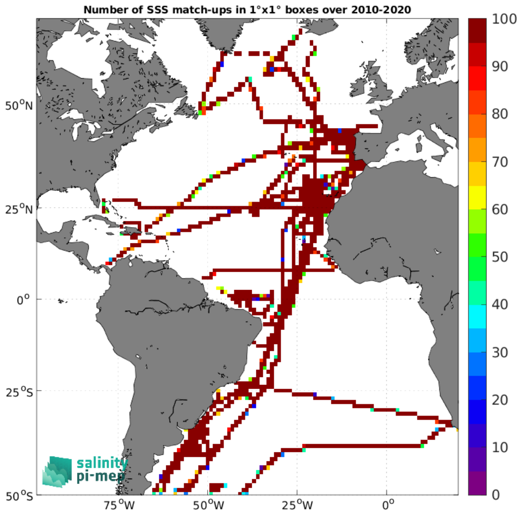
Figure 4: Number of SSS match-ups between TSG (CSIC-UTM) SSS and the CCI SSS L4 Merged-OI v3.2 - 7-day running (ESA) SSS product for the Atlantic Ocean Pi-MEP region over 1^\circ \times 1^\circ boxes and for the full satellite product period.
