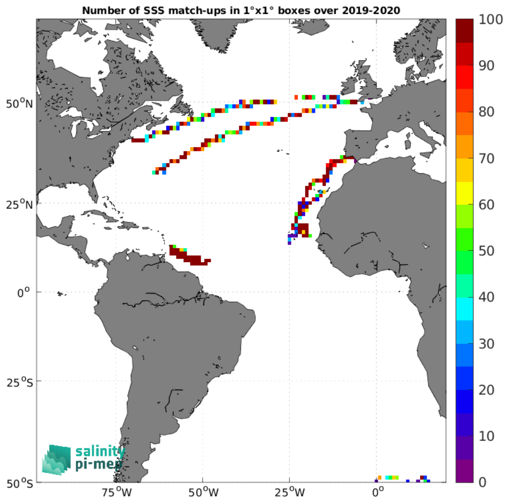
Figure 4: Number of SSS match-ups between Saildrone SSS and the CCI SSS L4 Merged-OI v3.2 - 7-day running (ESA) SSS product for the Atlantic Ocean Pi-MEP region over 1^\circ \times 1^\circ boxes and for the full satellite product period.
