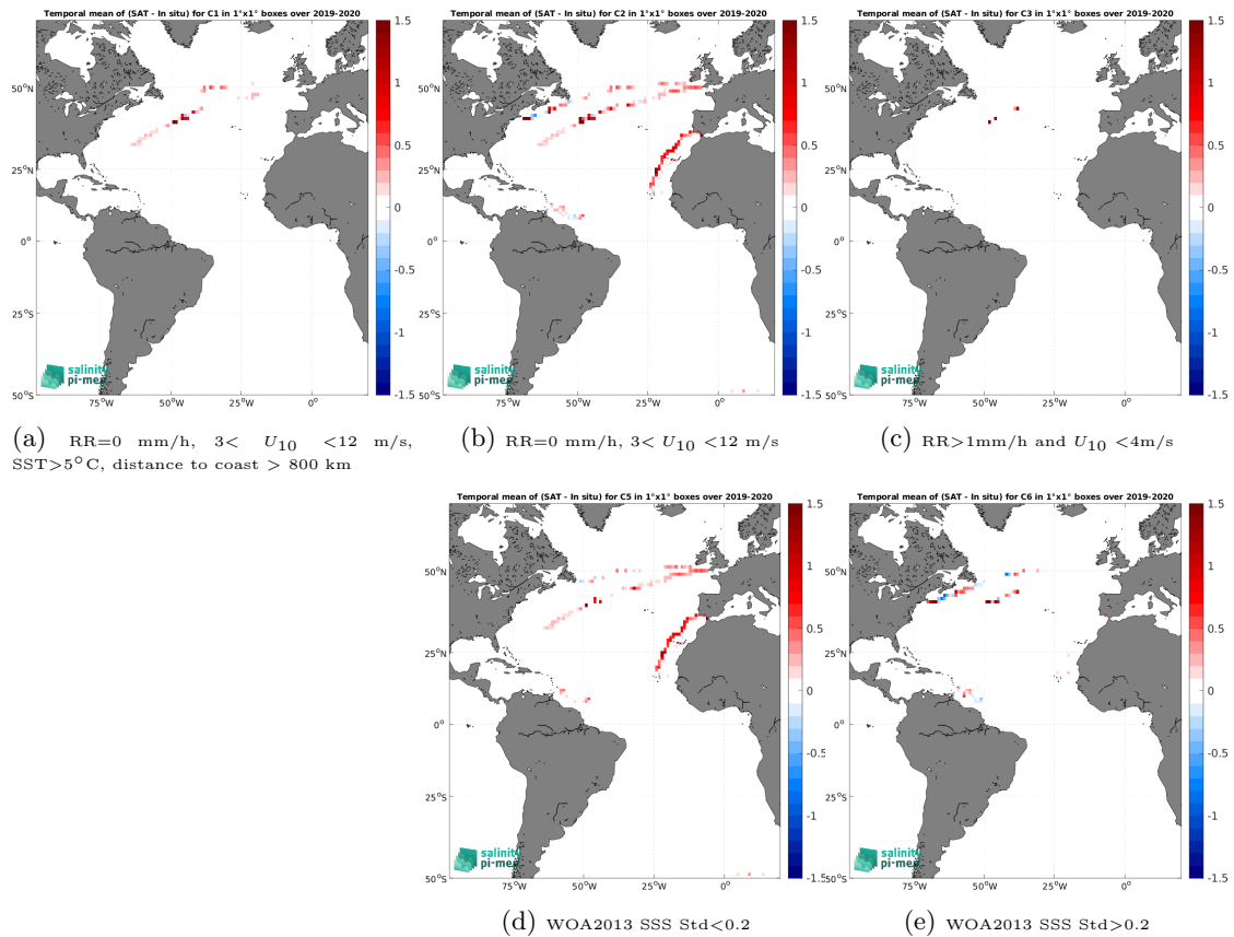
Figure 12: Temporal mean gridded over spatial boxes of size 1^\circ \times 1^\circ of \Delta\text{SSS} (CCI SSS L4 Merged-OI v3.2 - 7-day running (ESA) - Saildrone) for 5 different subdatasets corresponding to:RR=0 mm/h, 3 < U_{10} < 12 m/s, SST >5^\circ\text{C} , distance to coast > 800 km (a), RR=0 mm/h, 3 < U_{10} < 12 m/s (b), RR >1 mm/h and U_{10} < 4 m/s (c), WOA2013 SSS Std <0.2 (d), WOA2013 SSS Std >0.2 (e).
