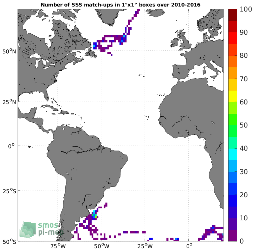
Figure 4: Number of SSS match-ups between Marine mammals SSS and the CCI SSS L4 Merged-OI v3.2 - 7-day running (ESA) SSS product for the Atlantic Ocean Pi-MEP region over 1°x1° boxes and for the full satellite product period.
