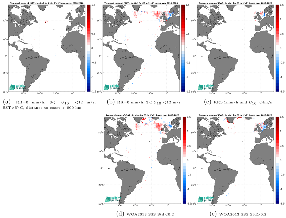
Figure 12: Temporal mean gridded over spatial boxes of size 1^\circ \times 1^\circ of \Delta\text{SSS} (CCI SSS L4 Merged-OI v3.2 - 7-day running (ESA) - ICES) for 5 different subdatasets corresponding to:RR=0 mm/h, 3 < U_{10} < 12 m/s, SST >5^\circ\text{C} , distance to coast > 800 km (a), RR=0 mm/h, 3 < U_{10} < 12 m/s (b), RR >1 mm/h and U_{10} < 4 m/s (c), WOA2013 SSS Std <0.2 (d), WOA2013 SSS Std >0.2 (e).
