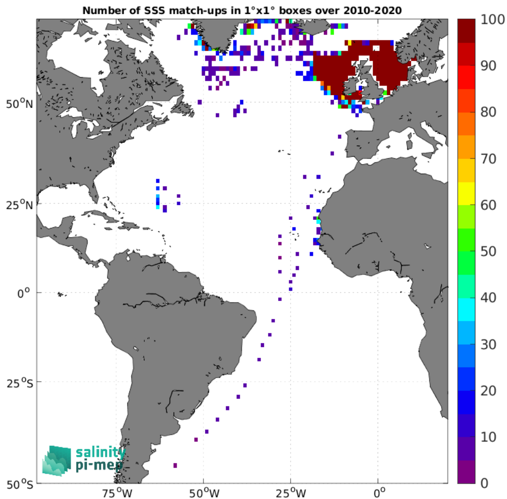
Figure 4: Number of SSS match-ups between ICES SSS and the CCI SSS L4 Merged-OI v3.2 - 7-day running (ESA) SSS product for the Atlantic Ocean Pi-MEP region over 1°×1° boxes and for the full satellite product period.
