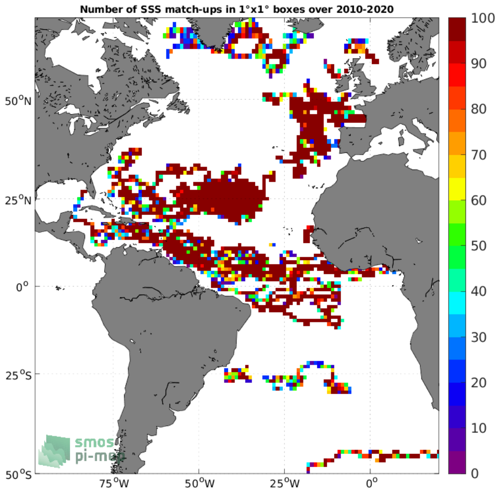
Figure 3: Number of SSS match-ups between Surface drifters SSS and the CCI SSS L4 Merged-OI v3.2 - 7-day running (ESA) SSS product for the Atlantic Ocean Pi-MEP region over 1^\circ \times 1^\circ boxes and for the full satellite product period.
