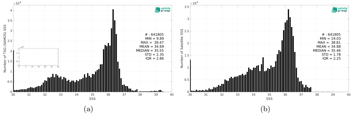
Figure 2: Histograms of SSS from TSG (SAMOS) (a) and CCI SSS L4 Merged-OI v3.2 - 30-day running (ESA) (b) considering all match-up pairs per bins of 0.1 over the Atlantic Ocean Pi-MEP region and for the full satellite product period.
