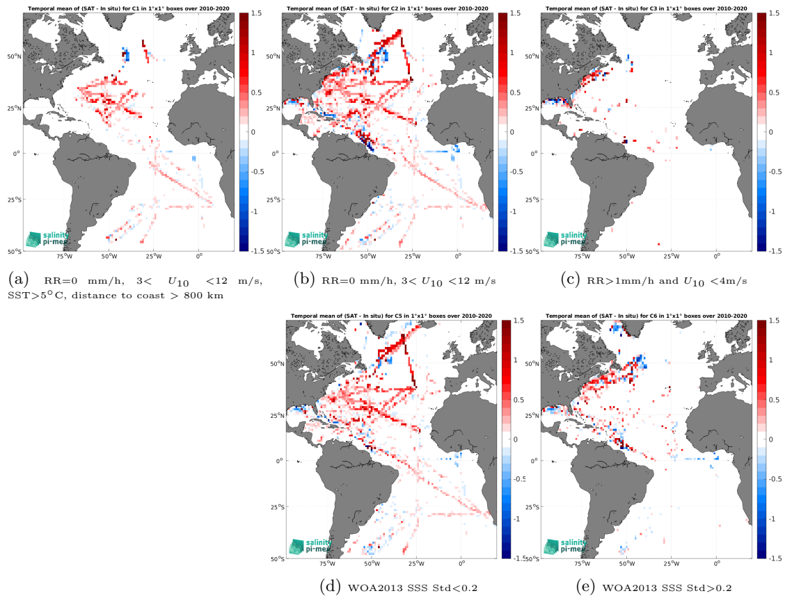
Figure 12: Temporal mean gridded over spatial boxes of size 1^\circ \times 1^\circ of \Delta\text{SSS} (CCI SSS L4 Merged-OI v3.2 - 30-day running (ESA) - TSG (SAMOS)) for 5 different subdatasets corresponding to:RR=0 mm/h, 3 < U_{10} < 12 m/s, SST >5^\circ\text{C} , distance to coast > 800 km (a), RR=0 mm/h, 3 < U_{10} < 12 m/s (b), RR >1 mm/h and U_{10} < 4 m/s (c), WOA2013 SSS Std <0.2 (d), WOA2013 SSS Std >0.2 (e).
