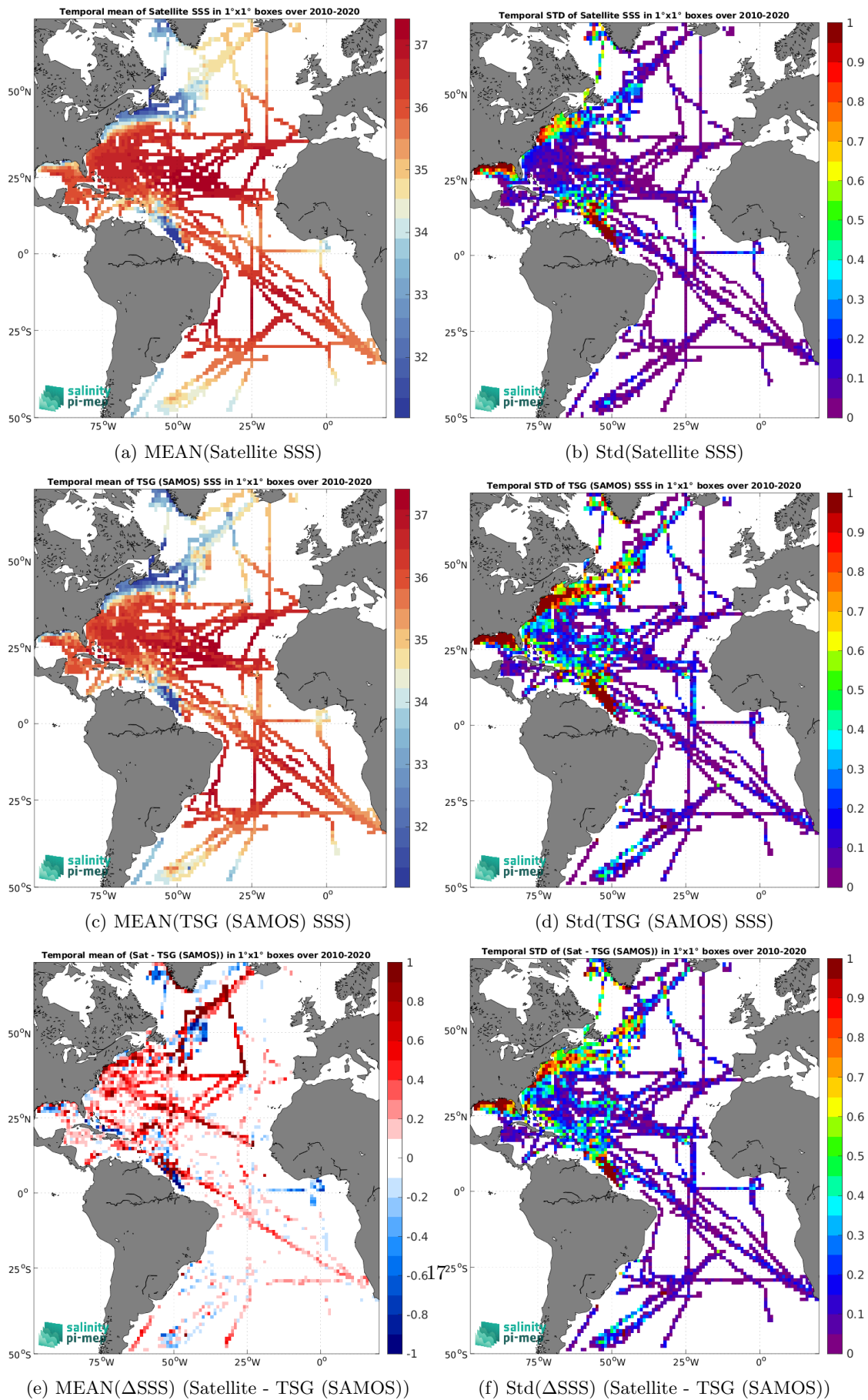
Figure 6: Temporal mean (left) and Std (right) of SSS from CCI SSS L4 Merged-OI v3.2 - 30-day running (ESA) (top), TSG (SAMOS) (middle), and of \Delta SSS (Satellite - TSG (SAMOS)). Only match-up pairs are used to generate these maps.
