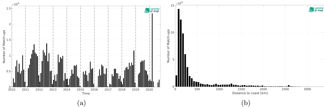
Figure 1: Number of match-ups between TSG (SAMOS) and CCI SSS L4 Merged-OI v3.2 - 30-day running (ESA) SSS as a function of time (a) and as function of the distance to coast (b) over the Atlantic Ocean Pi-MEP region and for the full satellite product period.
