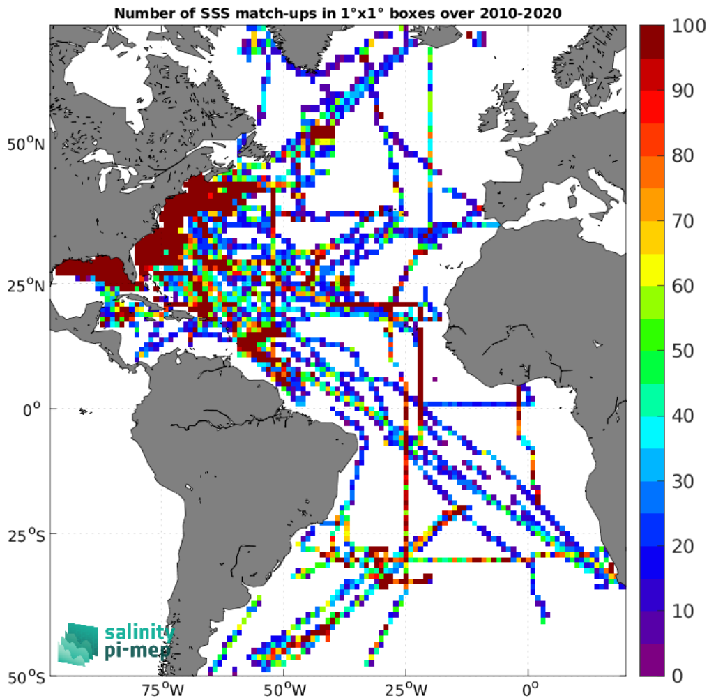
Figure 4: Number of SSS match-ups between TSG (SAMOS) SSS and the CCI SSS L4 Merged-OI v3.2 - 30-day running (ESA) SSS product for the Atlantic Ocean Pi-MEP region over 1^\circ \times 1^\circ boxes and for the full satellite product period.
